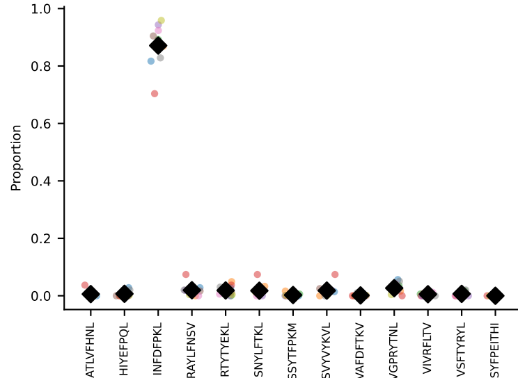
#19 AV8-1-CATDGSSGSWQLIF-AJ22_BV4-CASTTANTEVFF-BJ1-1 coh=0.993, n=11
