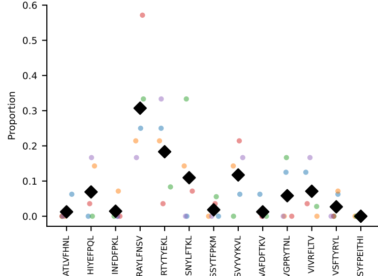
#95 AV16/DV11-CAMRSNTGYQNIFY-AJ49_BV13-1-CASSGLREQYF-BJ2-7 coh=0.656, n=5
