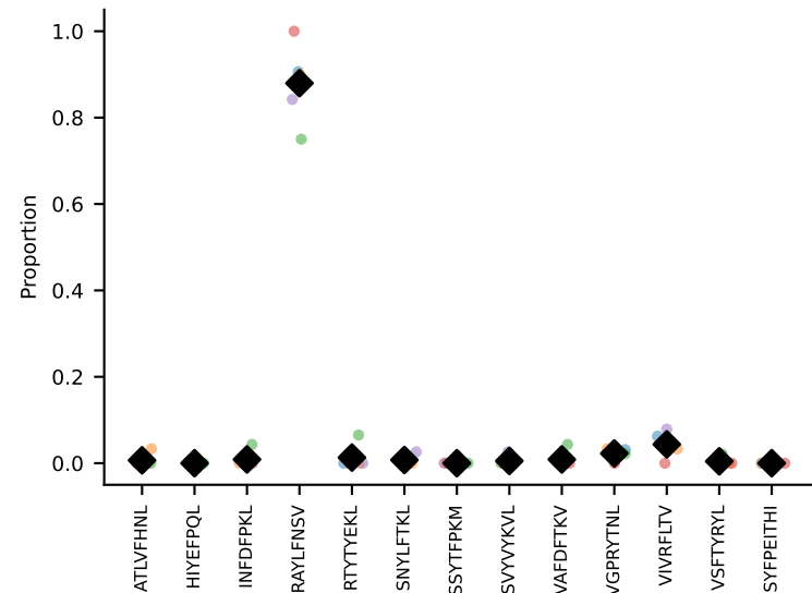
#21 AV16D/DV11-CAMREDNAGAKLTF-AJ39_BV2-CASSQDHVSNERLFF-BJ1-4 coh=0.992, n=6
