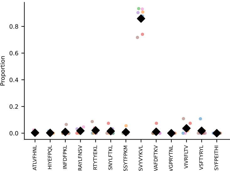
#29 AV7-3-CAVSIAGSWQLIF-AJ22_BV13-1-CASSDAGYEYQF-BJ2-7 coh=0.985, n=11
