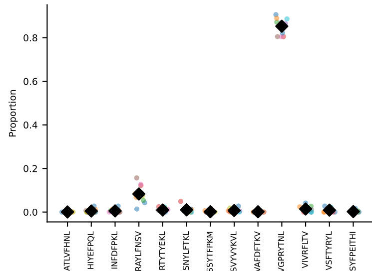
#18 AV16D/DV11-CAMREDTGYQNFYF-AJ49_BV19-CASTGTGSNYAEQFF-BJ2-1 coh=0.995, n=15
