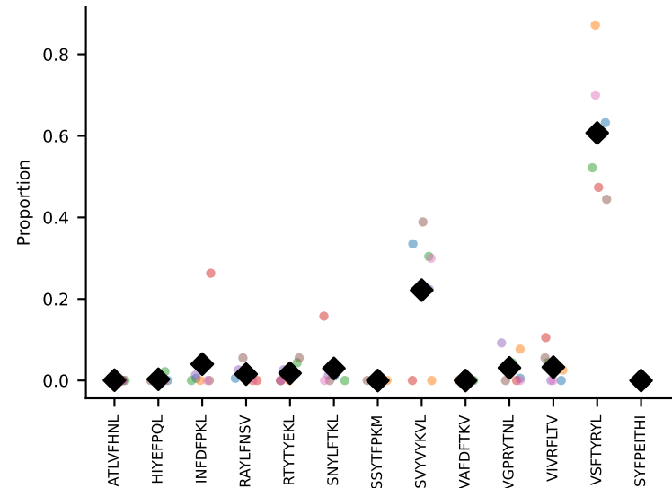
#69 AV6D-5-CALGDQGGSAKLIF-AJ57_BV13-2-CASGDWGWWEQYF-BJ2-7 coh=0.881, n=7
