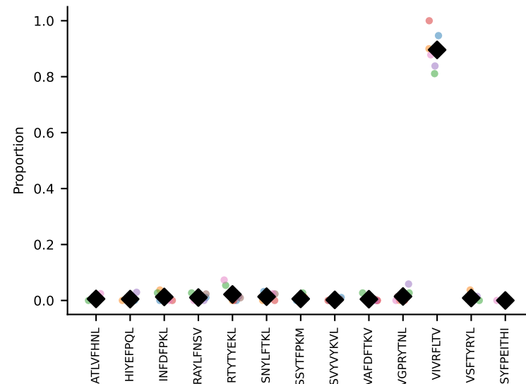
#17 AV6D-6-CALRWDTNAYKVIF-AJ30_BV19-CASRGGVTYEQYF-BJ2-7 coh=0.995, n=5
