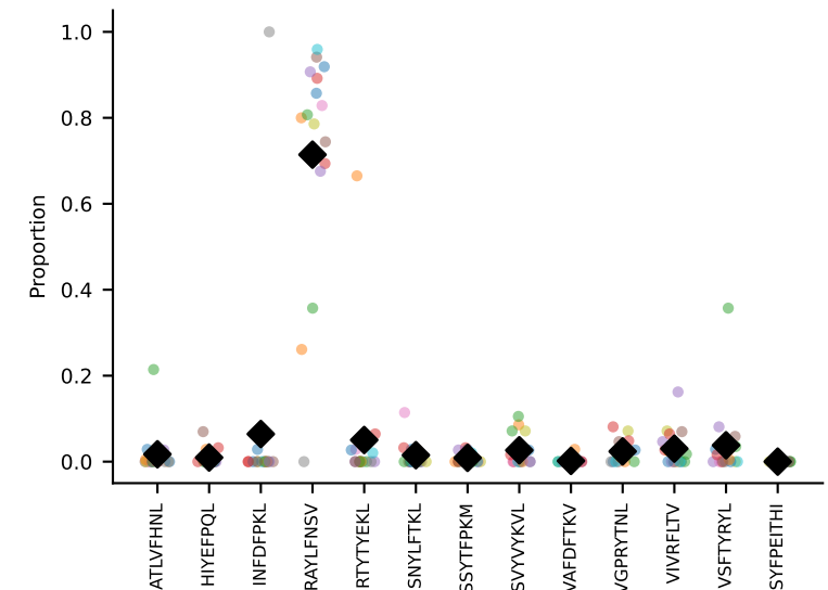
#92 AV8-1-CATEPDTGYQNIFY-AJ49_BV3-CASSLAWGLNYAEQFF-BJ2-1 coh=0.727, n=5
