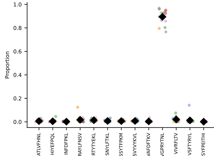
#22 AV9-3-CAVSSDYANKMIF-AJ47_BV3-CASSSGTGGYEYF-BJ2-7 coh=0.992, n=14
