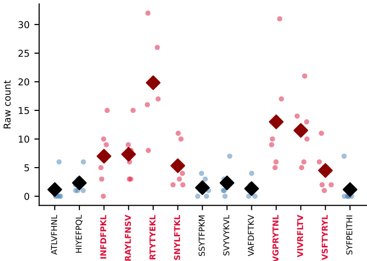
#181 AV12-2-CALSDQPYANKMIF-AJ47_BV5-CASSQAGQNTVEFF-BJ1-1 MULTIPLE (RTYTYEKL+VGPRYTNL+5more) coherence=0.825, n=6, cumulative sum=0.87
