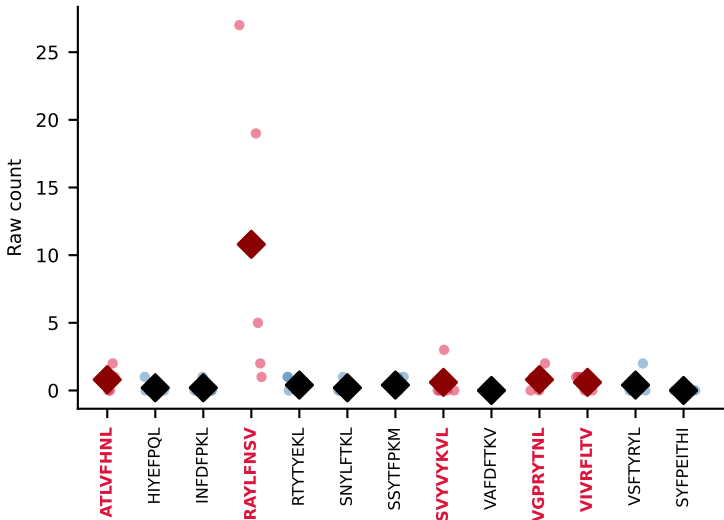
#233 AV3-3-CAVSVNYGGSGNKLIF-AJ32_BV5-CASSQDLWGAGSQNTLYF-BJ2-4 MULTIPLE (RAYLFNSV+VGPRYTNL+3more) coherence=0.626, n=5, cumulative sum=0.88
