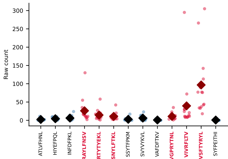
#190 AV16D/DV11-CAMREGNTNTGKLTf-AJ27_BV1-CTCSADGVYAEQFF-BJ2-1 MULTIPLE (VSFTYRYL+VIVRFLTV+4more) coherence=0.809, n=14, cumulative sum=0.89
