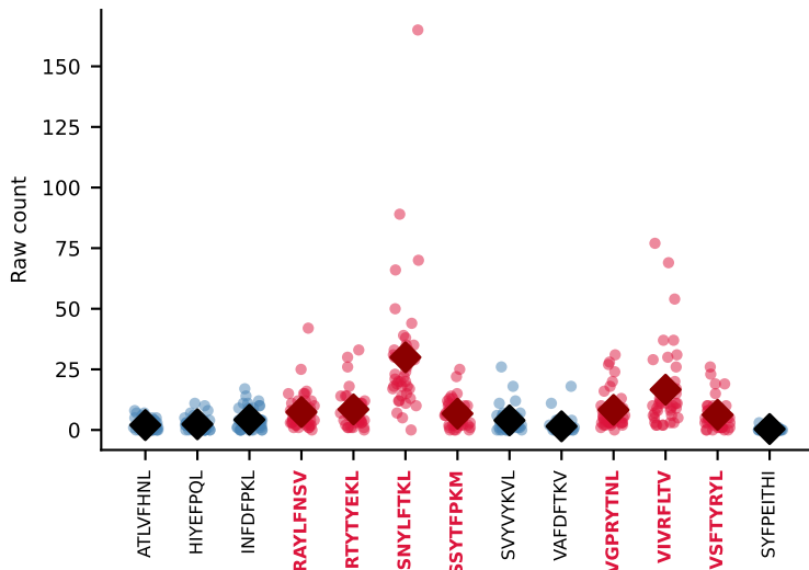
#187 AV19-CAAANTGYQNIFYF-AJ49_BV17-CASSRDPWGGSATLYF-BJ2-3 MULTIPLE (SNYLFTKL+VIVRFLTV+5more) coherence=0.817, n=39, cumulative sum=0.85
