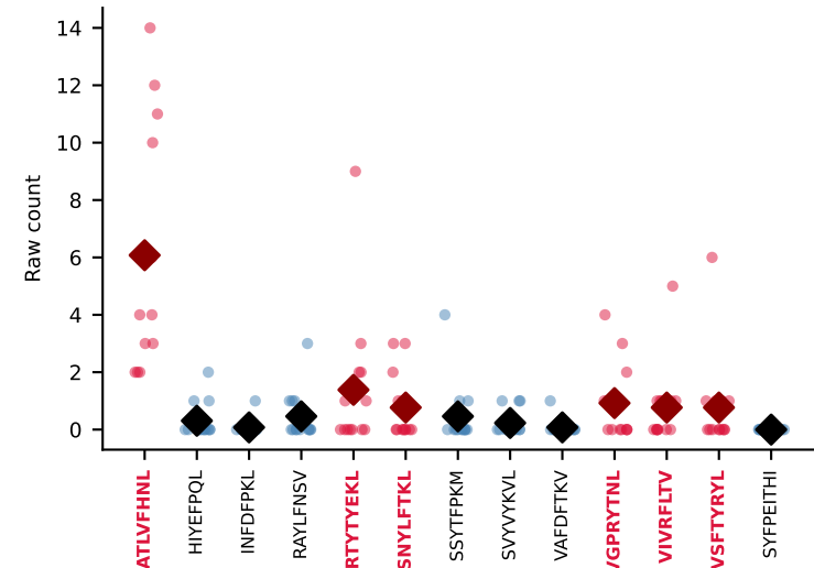
#211 AV12-3-CALSDTNAYKVIF-AJ30_BV3-CASSPDRDTEVFF-BJ1-1 MULTIPLE (ATLVFHNL+RTTYYEKL+4more) coherence=0.758, n=13, cumulative sum=0.87
