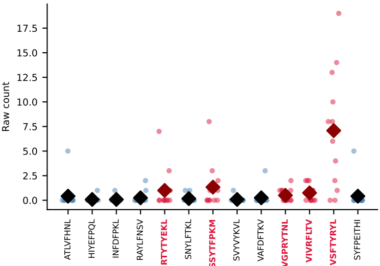
#240 AV4-3-CAADQGRALIF-AJ15_BV13-2-CASGWAPLGDYEQYF-BJ2-7 MULTIPLE (VSFTYRYL+SSYTFPKM+3more) coherence=0.500, n=12, cumulative sum=0.86
