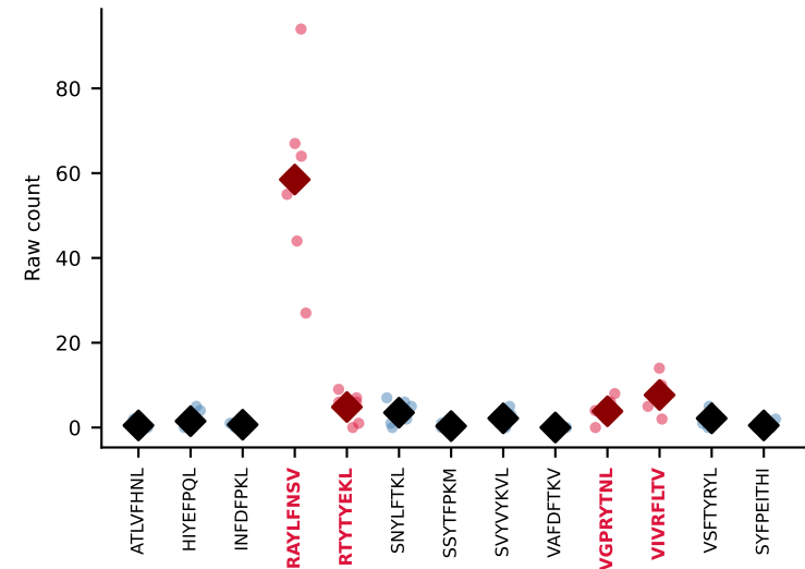
#107 AV16D/DV11-CAMRPYGGSGNKLIF-AJ32_BV1-CTCSAVREDTQYf-BJ2-5 MULTIPLE (RAYLFNSV+VIVRFLTV+2more) coherence=0.958, n=6, cumulative sum=0.87
