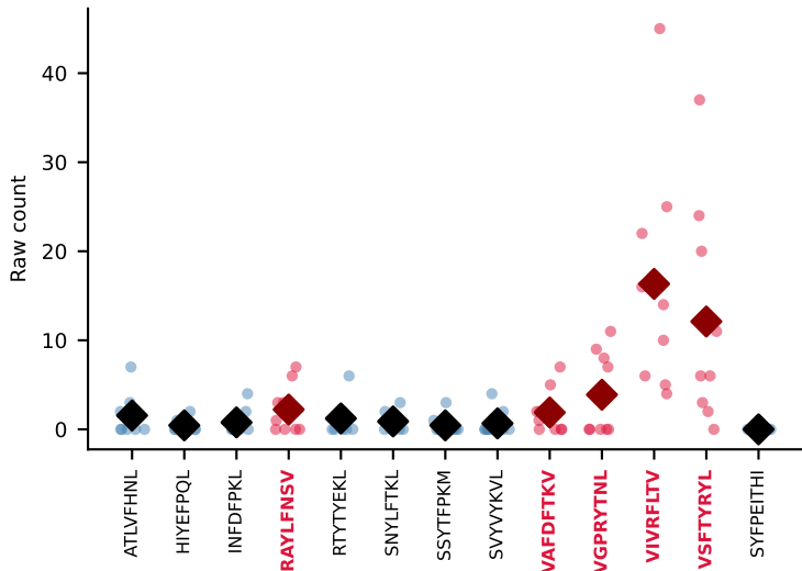
#184 AV3D-3-CAVNSGSWQLIF-AJ22_BV1-CTCSADPGDYAEQFF-BJ2-1 MULTIPLE (VIVRFLTV+VSFTYRYL+3more) coherence=0.823, n=9, cumulative sum=0.86
