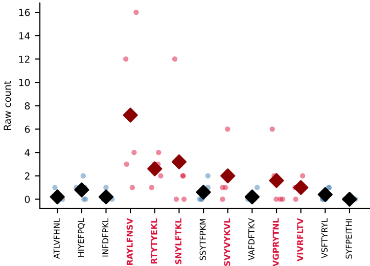
#230 AV16/DV11-CAMRSNTGYQNFYF-AJ49_BV13-1-CASSGLREQYF-BJ2-7 MULTIPLE (RAYLFNSV+SNYLFTKL+4more) coherence=0.656, n=5, cumulative sum=0.88
