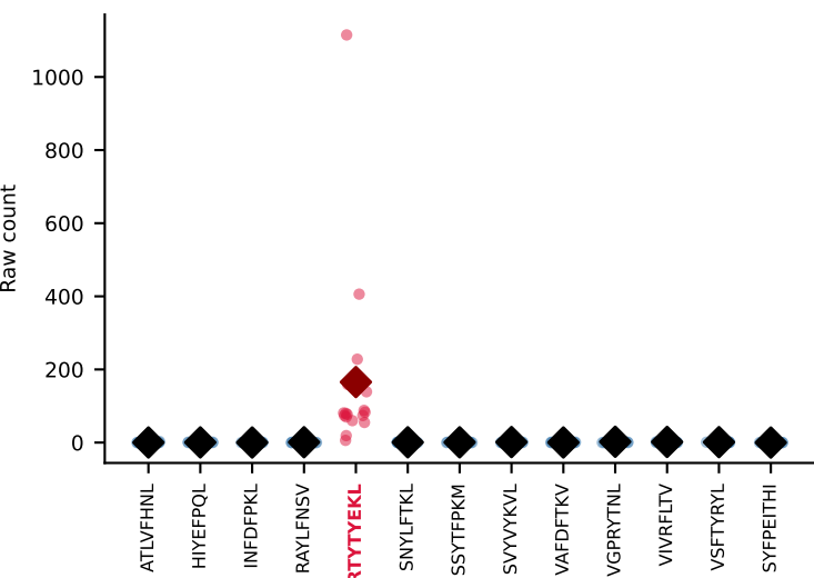
#10 AV16/DV11-CAMREAFSGGSNAKLTF-AJ42_BV13-2-CASGDSYEQYF-BJ2-7 SINGLE (RTYTYEKL) coherence=0.998, n=17, cumulative sum=0.94
