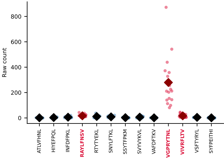
#97 AV16D/DV11-CAMREDSGYNKLTf-AJ11*p02_BV13-2-CASGTTYEQYf-BJ2-7 MULTIPLE (VGPRYTNL+RAYLFNSV+1more) coherence=0.972, n=17, cumulative sum=0.87
