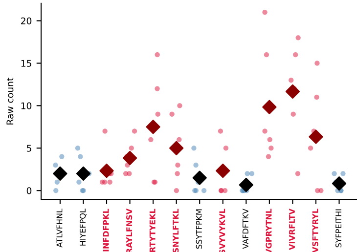
#227 AV13D-4-CAMDTGYQNFYf-AJ49_BV5-CASSQDSNTEVFF-BJ1-1 MULTIPLE (VIVRFLTV+VGPRYTNL+6more) coherence=0.709, n=6, cumulative sum=0.87
