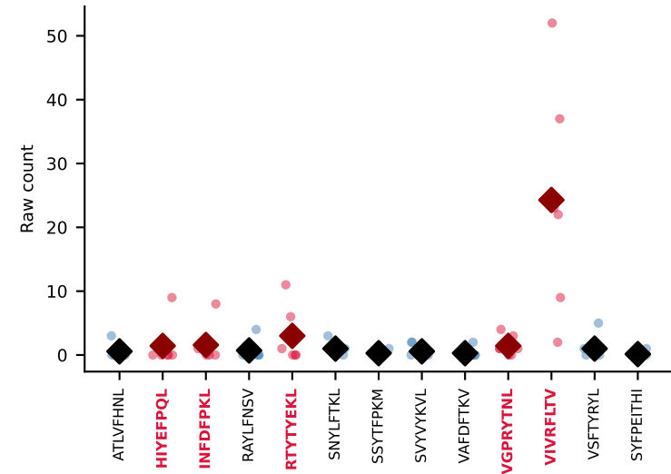
#103 AV9D-4-CALSATNAYKVIF-AJ30_BV13-2-CASGDAAGKDTQYf-BJ2-5 MULTIPLE (VIVRFLTV+RTTYEKL+3more) coherence=0.960, n=7, cumulative sum=0.87
