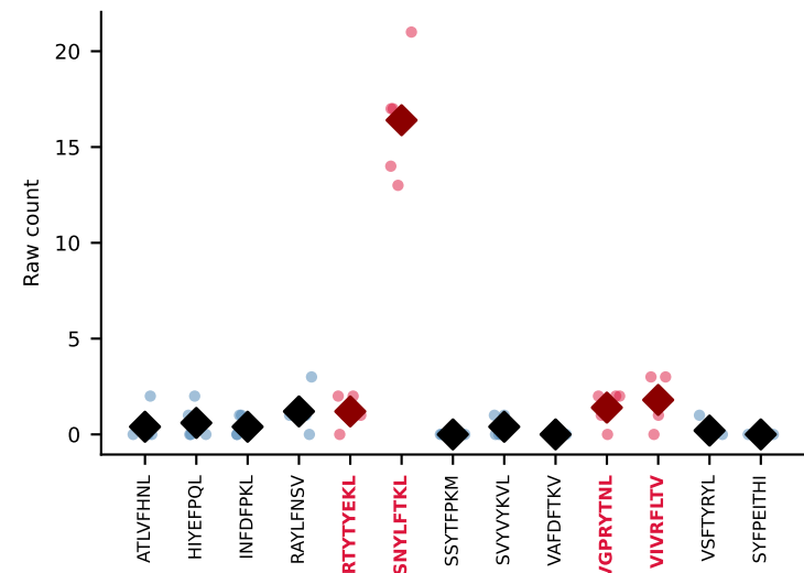
#96 AV10-CAAGQGGRALIF-AJ15_BV31-CAWNWGGSQNTLYF-BJ2-4 MULTIPLE (SNYLFTKL+VIVRFLTV+2more) coherence=0.974, n=5, cumulative sum=0.87
