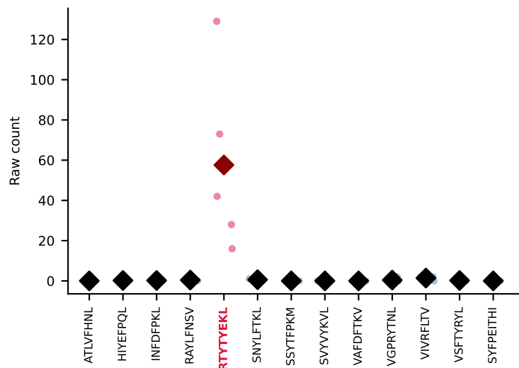
#3 AV16D/DV11-CAMREGDSNYQLIW-AJ33_BV3-CASSATGANTGQLYF-BJ2-2 SINGLE (RTYTYEKL) coherence=0.999, n=5, cumulative sum=0.94
