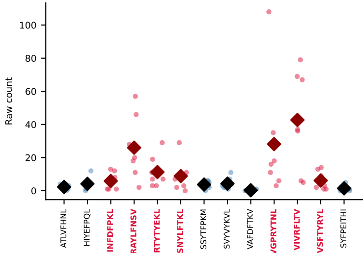
#207 AV6-6-CALGDLGTGSKLSF-AJ58_BV13-2-CASGPGTSEVFF-BJ1-1 MULTIPLE (VIVRFLTV+VGPRYTNL+5more) coherence=0.766, n=7, cumulative sum=0.89
