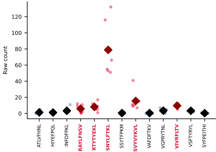
#99 AV16/DV11-CAMREGNNNNAPRF-AJ43*p03_BV13-2-CASGENTGQLYf-BJ2-2 MULTIPLE (SNYLFTKL+SVVYKVL+3more) coherence=0.970, n=6, cumulative sum=0.89
