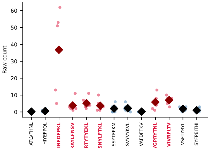
#210 AV7D-3-CAVYQGGRALIF-AJ15_BV13-2-CASGDVLGGYEQYF-BJ2-7 MULTIPLE (INFDFPKL+VIVRFLTV+4more) coherence=0.760, n=6, cumulative sum=0.89
