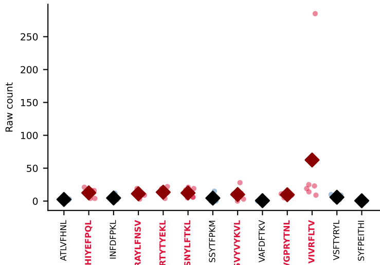
#215 AV9-3-CAVSIHYGNEKITF-AJ48_BV13-1-CASSGDRGYNSPLYF-BJ1-6 MULTIPLE (VIVRFLTV+RTTYYEKL+5more) coherence=0.746, n=6, cumulative sum=0.88
