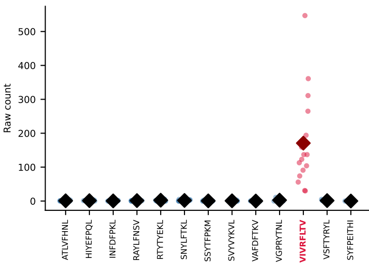
#5 AV3-1-CAVRASSGSWQLIF-AJ22_BV4-CASSSIEQFF-BJ2-1 SINGLE (VIVRFLTV) coherence=0.999, n=16, cumulative sum=0.93
