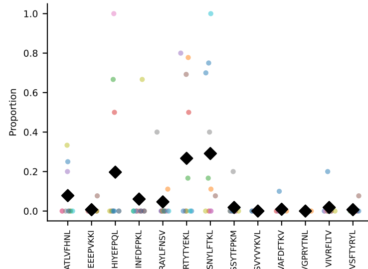
#68 AV7D-5-CAVRDTGGLSGKLT-F-AJ2_BV1-CTCSADRLGSAETLYF-BJ2-3 coh=0.272, n=7
