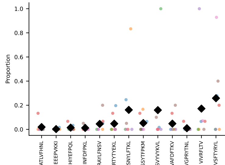
#84 AV8D-2-CATDPSSGQKLf-AJ16_BV3-CASSLAWGASYEQYF-BJ2-7 coh=0.249, n=6
