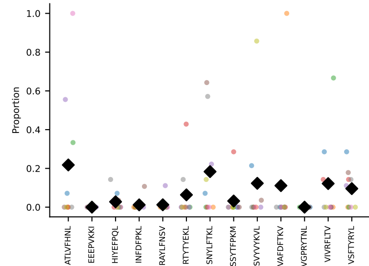
#125 AV9D-3-CAVSMLSGSFNKLTF-AJ4_BV3-CASSQYL RDNQDTQYF-BJ2-5 coh=0.180, n=32
