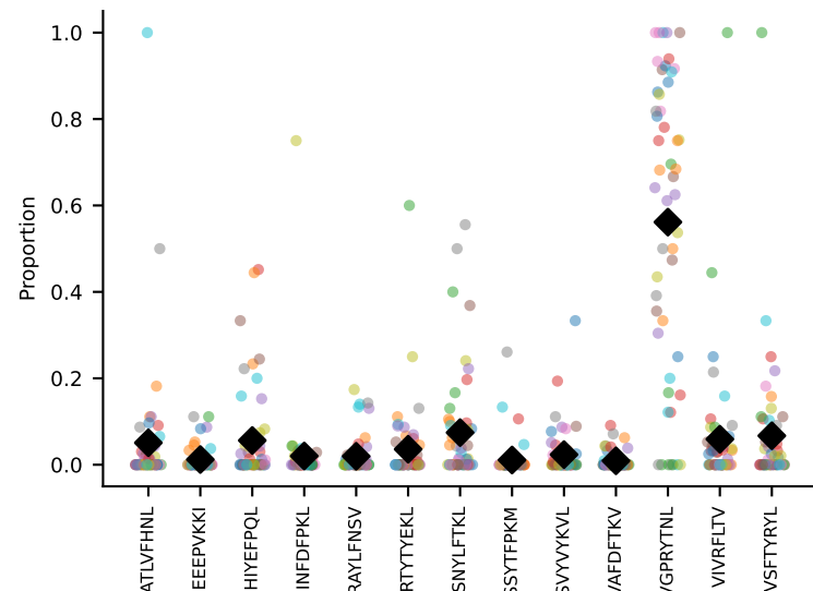
#10 AV14-2-CAASGDYAQGLTF-AJ26_BV3-CASSLGQDTQYF-BJ2-5 coh=0.596, n=50
