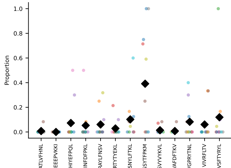
#58 AV19-CAAGAAGYQNFYF-AJ49_BV17-CASSRRTGANTGQLYF-BJ2-2 coh=0.294, n=11
