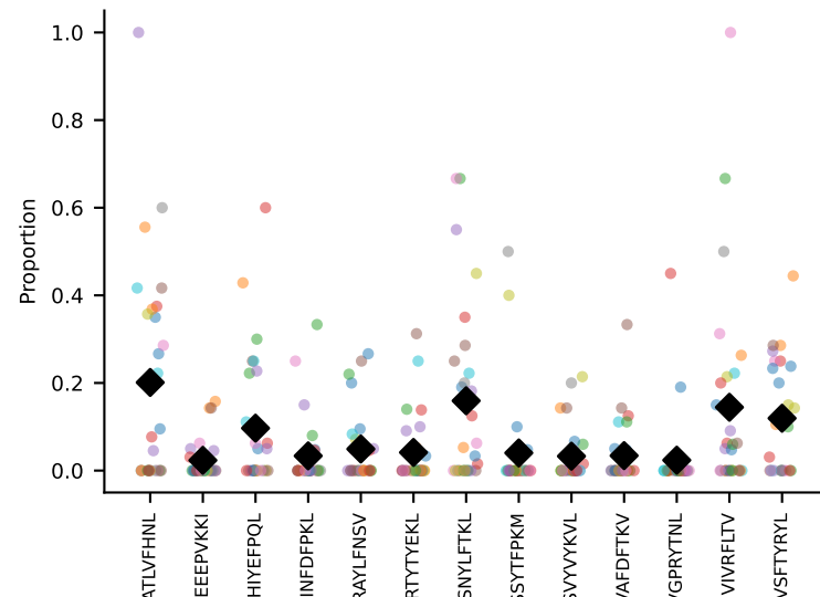
#42 AV13-2-CAIDSNNTNKVVFF-AJ34_BV1-CTCSSQNTLYF-BJ2-4 coh=0.332, n=6
