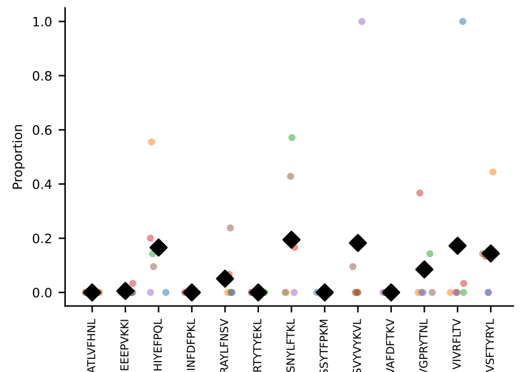
#103 AV4D-4-CAAEPASSGSWQLIF-AJ22_BV16-CASSLELGSDTQYF-BJ2-5#104 AV7-2-CAASMRGSALGRLHF-AJ18_BV14-CASSFRQGAVTGQLYF-BJ2-1 coh=0.225, n=8coh=0.223, n=7
