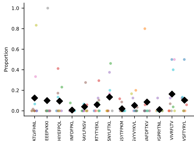
#103 AV4D-4-CAAEPASSGSWQLIF-AJ22_BV16-CASSLELGSDTQYF-BJ2-5#104 AV7-2-CAASMRGSALGRLHF-AJ18_BV14-CASSFRQGAVTGQLYF-BJ2-1 coh=0.225, n=8coh=0.223, n=7
