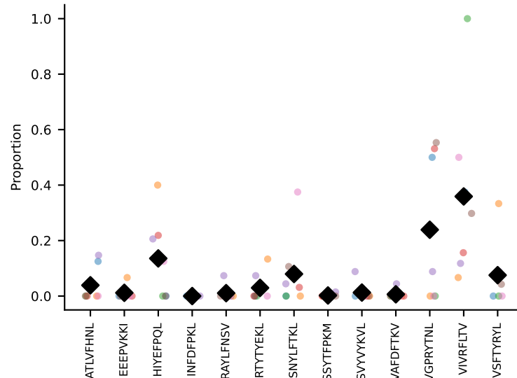
#23 AV21/DV12-CILRVANNNNAPRF-AJ43_BV2-CASSQEQGYAEQFF-BJ2-1 coh=0.437, n=41
