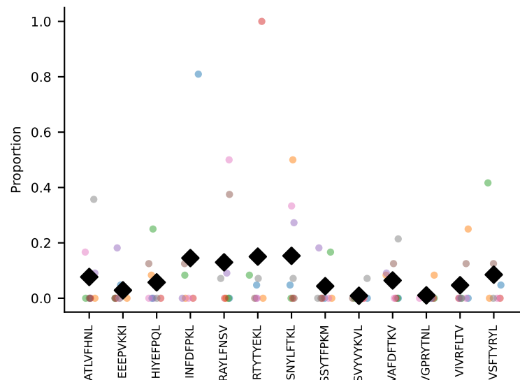
#107 AV16-CAMREDGYQNIFYF-AJ49_BV16-CASSLGWGGREQYF-BJ2-7 coh=0.220, n=38
