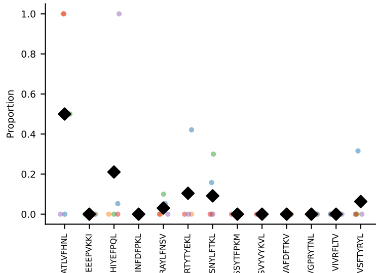
#53 AV19-CAANQGGSAKLIF-AJ57_BV5-CASSRQVNYAEQFF-BJ2-1 coh=0.300, n=10
