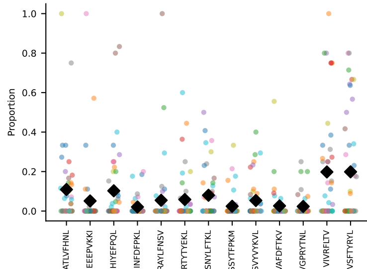
#67 AV7-4-CAASSDTNAYKVIF-AJ30_BV2-CASSQRTGVNTLYF-BJ2-4 coh=0.272, n=5
