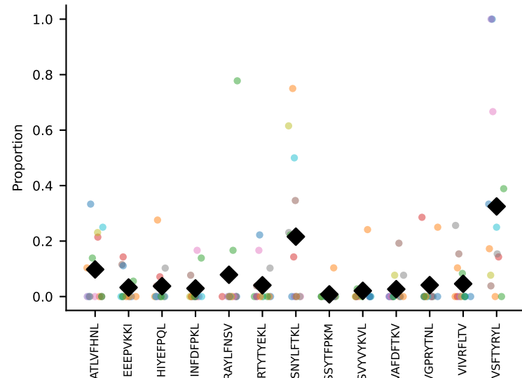
#30 AV6-6-CALGESGGSNAKLTF-AJ42_BV13-3-CASSDAQTYNSPLYF-BJ1-6 coh=0.371, n=18
