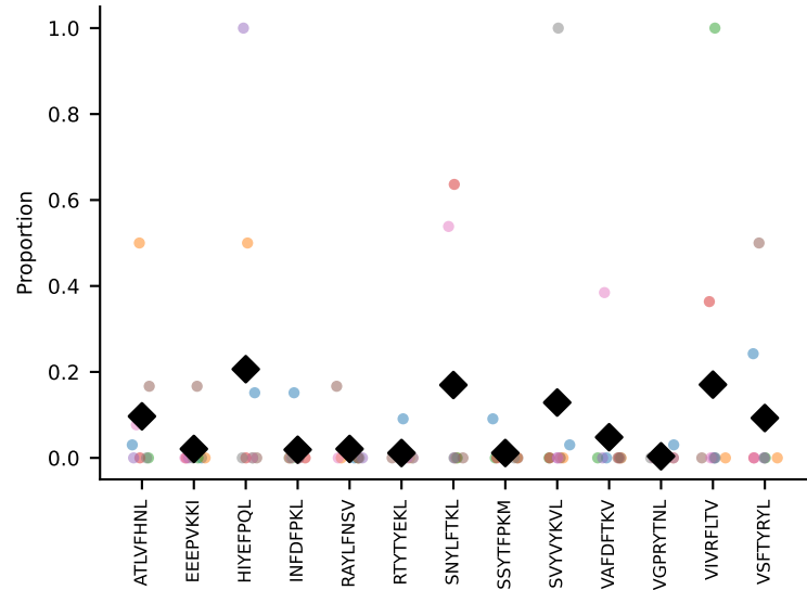
#131 AV11-CVVGRRYGSSGNKLIF-AJ32_BV19-CASSTDRGLNSPLYF-BJ1-6 coh=0.155, n=8
