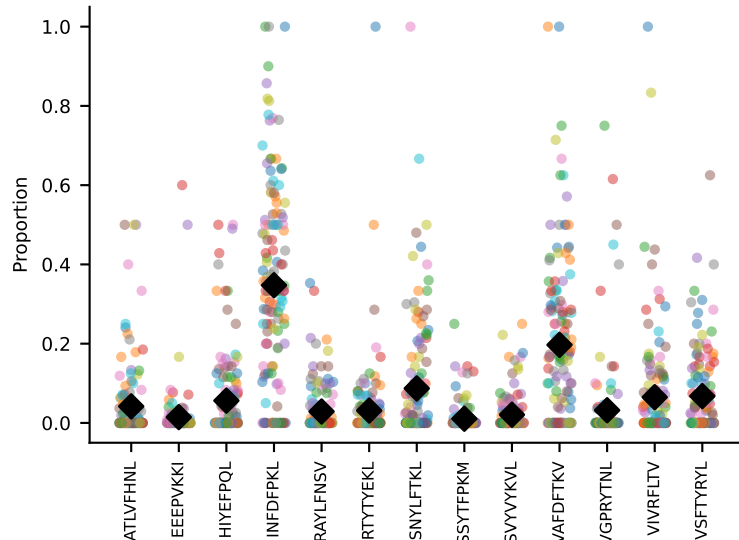
#21 AV16N-CAMREGNSNNRIFF-AJ31_BV13-1-CASRDINTEVFF-BJ1-1 coh=0.448, n=12
