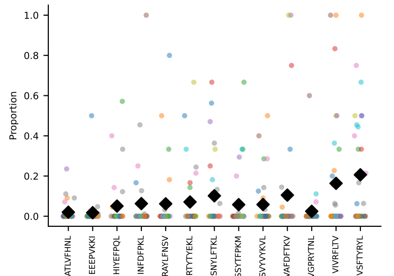
#108 AV7-3-CAVSAEGADRLTF-AJ45_BV1-CTCSADRGGSPLYF-BJ1-6 coh=0.219, n=32
