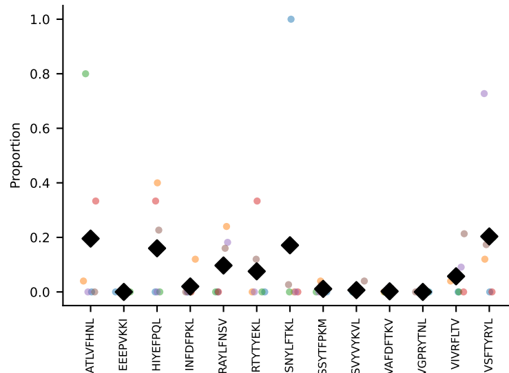
#82 AV9-1-CAVRASNTNKVVf-AJ34_BV31-CAWSLRTGGSYEQYF-BJ2-7 coh=0.252, n=6
