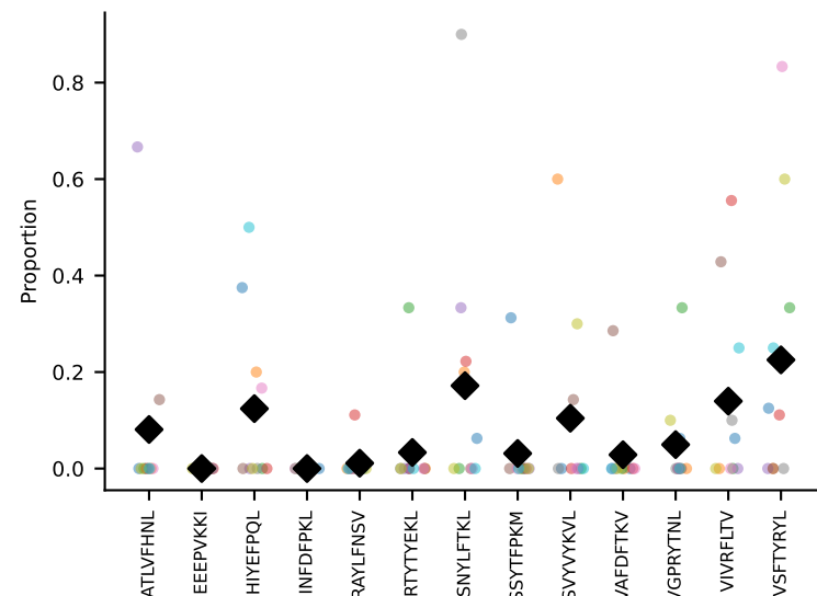
#101 AV16-CAMGTGSGGKLTf-AJ44_BV1-CTCSTRGANERLFF-BJ1-4 coh=0.226, n=46
