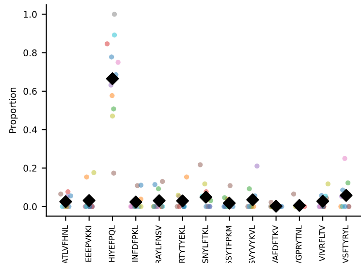
#5 AV16-CAMREANTGYQNFYF-AJ49_BV13-2-CASGDGAQNTLYF-BJ2-4 coh=0.742, n=13
