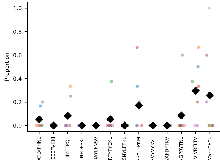
#55 AV12-3-CALSDNYNQGLIF-AJ23_BV2-CASSQAVSYEQYF-BJ2-7 coh=0.298, n=17
