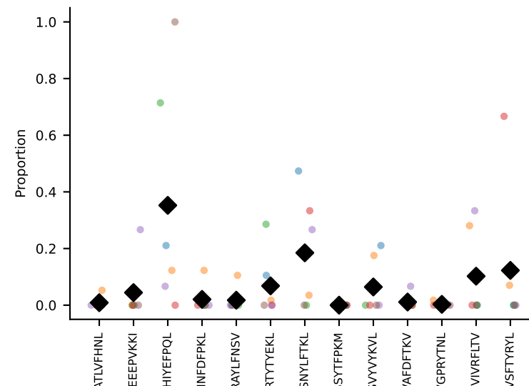
#48 AV7-4-CAASEDYNQGKLIF-AJ23_BV31-CAWSLGHYAEQFF-BJ2-1 coh=0.305, n=58
