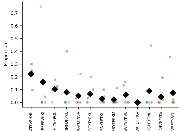
#79 AV14-1-CAASADTGNYKYVF-AJ40_BV13-3-CASSDSNTEVFF-BJ1-1 coh=0.255, n=11
