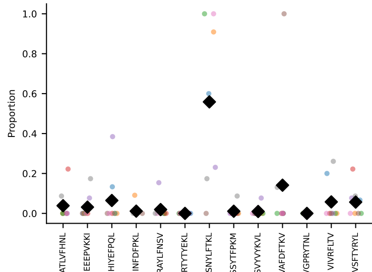
#19 AV14-2-CAASADTGNYKYVF-AJ40_BV13-3-CASSDNNQAPLF-BJ1-5 coh=0.473, n=7
