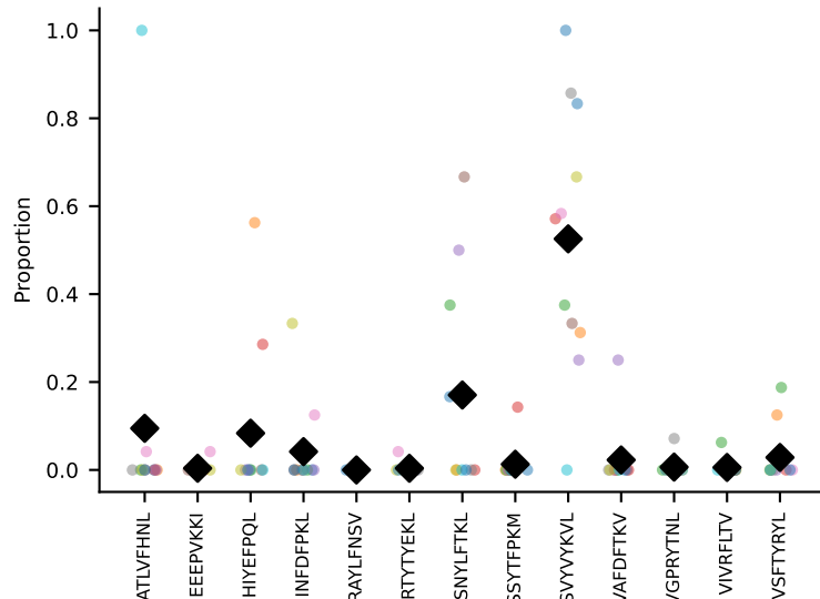
#17 AV13-2-CAPNNNAGAKLTF-AJ39_BV14-CASSDRYEQYF-BJ2-7 coh=0.502, n=133
