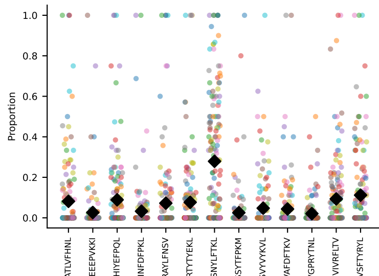
#47 AV13-2-CAIDSNNTGKLTF-AJ27_BV13-2-CASGDAGGEVFF-BJ1-1 coh=0.306, n=158
