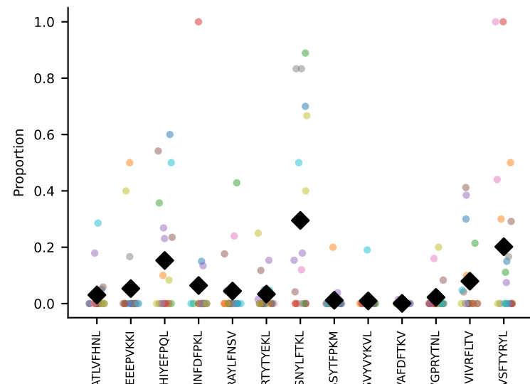
#45 AV7-5-CAVSLTGNTGKLIF-AJ37_BV19-CASSKDRFAEQFF-BJ2-1 coh=0.312, n=6
