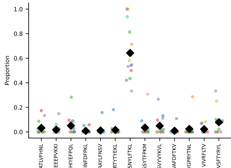
#7 AV5-1-CSASPSSGSWQLIF-AJ22_BV4-CASSNTGGAGAETLYF-BJ2-3 coh=0.685, n=22
