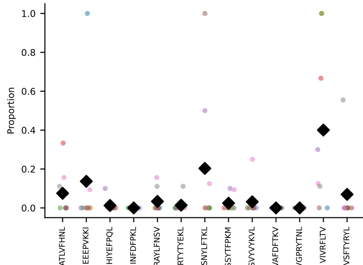
#66 AV17-CALEGSYGNEKITF-AJ48_BV1-CTCSADRVGSDYTF-BJ1-2 coh=0.273, n=37
