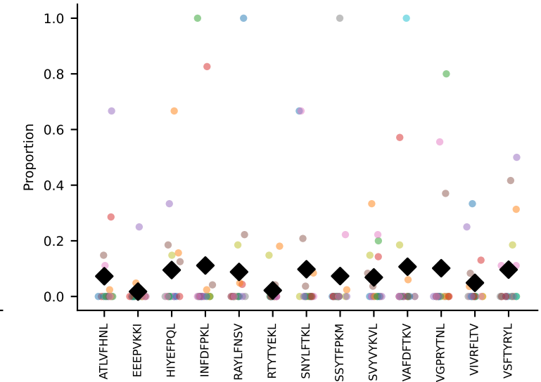
#132 AV6-6-CALGDLTGGNNKLTF-AJ56_BV13-3-CASKDRGREQYF-BJ2-2 coh=0.147, n=17
