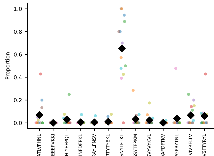
#9 AV16-CAMREANTGYQNFYF-AJ49_BV13-2-CASGTGGQNTLYF-BJ2-4 coh=0.607, n=87
