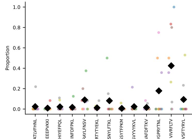
#32 AV14-2-CAASADYGSSGNKLIF-AJ32_BV4-CASRQFSYNSPLYF-BJ1-6 coh=0.362, n=33
