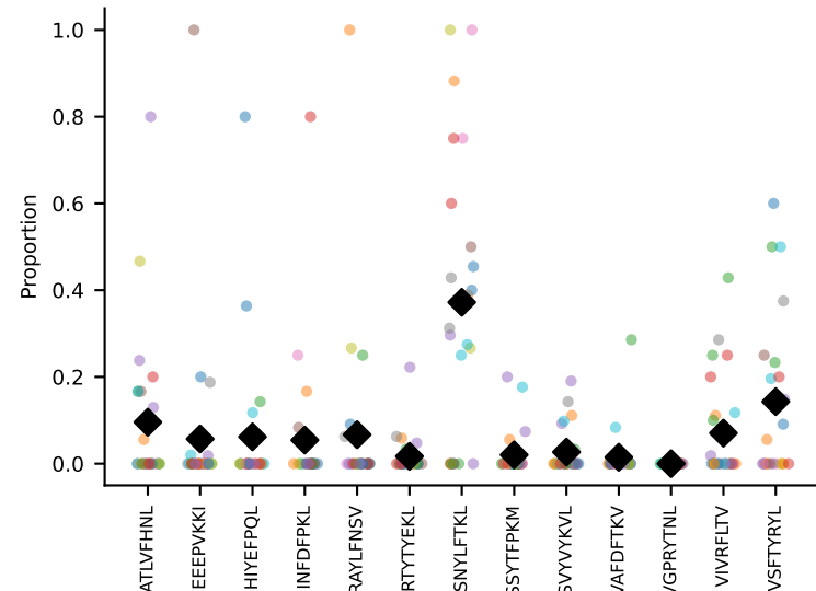
#29 AV16/DV11-CAMREGGGYKVVF-AJ12_BV13-2-CASGARTYNyAEQFF-BJ2-1 coh=0.375, n=12
