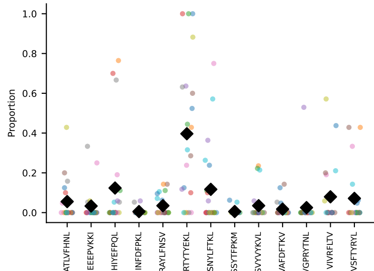
#31 AV14-1-CAASASSGSWQLIF-AJ22_BV1-CTCSGRDRANQAPLF-BJ1-5 coh=0.363, n=5
