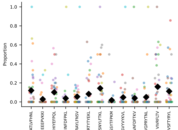
#81 AV7-2-CAASKGGRALIF-AJ15_BV13-1-CASSDWASSYEQYF-BJ2-7 coh=0.253, n=34
