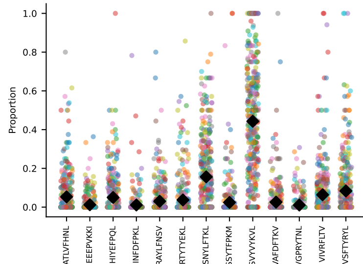
#18 AV14D-3/DV8-CAAGASSGSWLIF-AJ22_BV31-CAWSPRQGAGTEVFF-BJ1-1 coh=0.497, n=6
