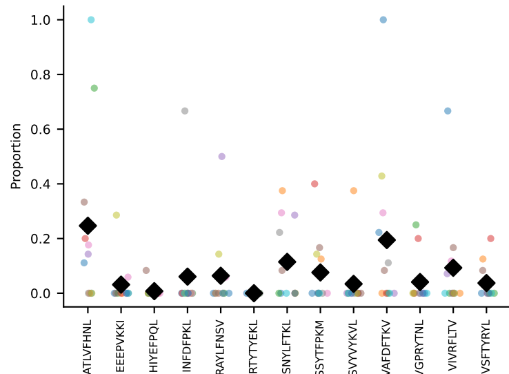
#83 AV7-3-CAVRQTQVVGQLTF-AJ5_BV20-CGARMGTEVFF-BJ1-1 coh=0.250, n=18
