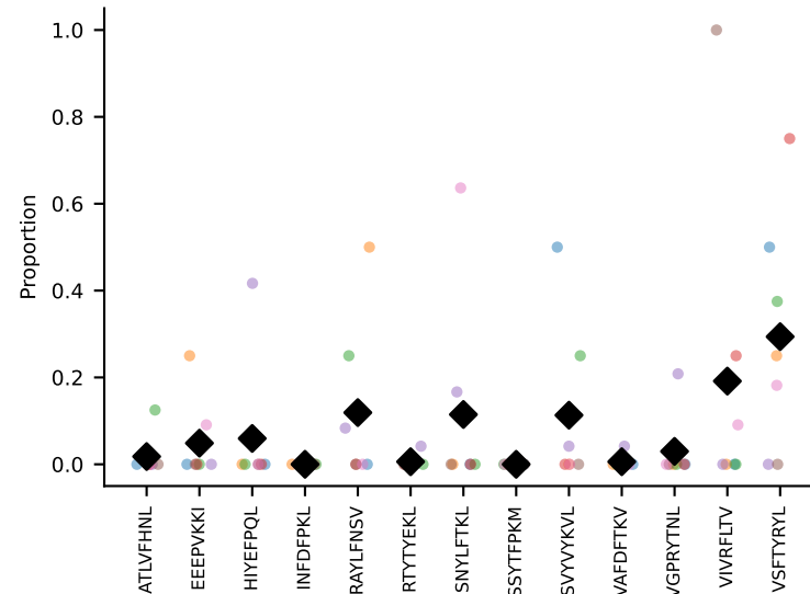
#80 AV10-CAASDVGDNSKLIW-AJ38_BV1-CTCSADWTSGNTLYF-BJ1-3 coh=0.254, n=7
