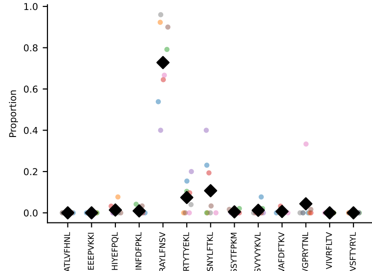
#20 AV7-2-CAAINNTNTGKLTF-AJ27_BV13-2-CASGDAGGGNERLFF-BJ1-4 coh=0.844, n=5
