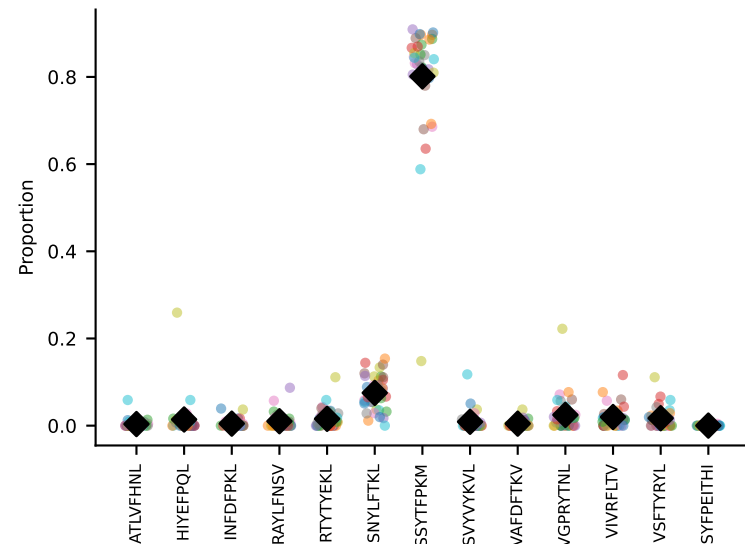
#41 AV9-2-CAASMDYANKMIF-AJ47_BV3-CASSLGAGYEQYF-BJ2-7 coh=0.951, n=6
