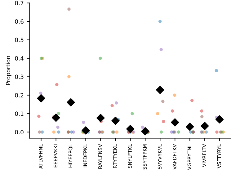
#29 AV9-2-CVL SVTGS GGLTL-AJ44_BV14-CASSFANTGQLYF-BJ2-2 coh=0.296, n=22
