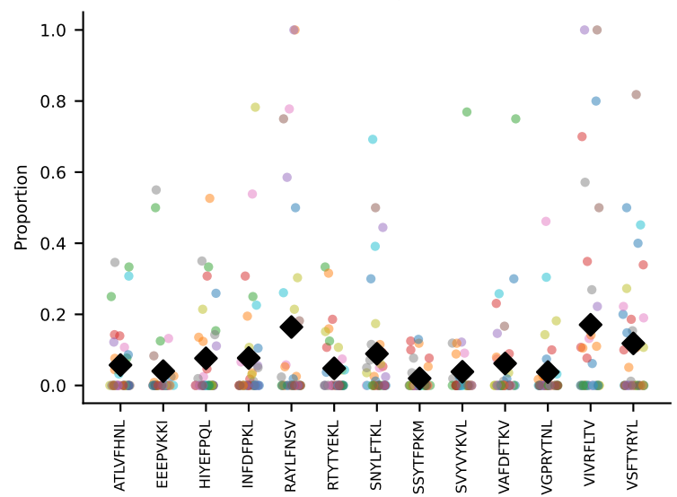
#41 AV16-CAMREANYGNEKITF-AJ48_BV16-CASSLRTGVYEYF-BJ2-7 coh=0.241, n=5
