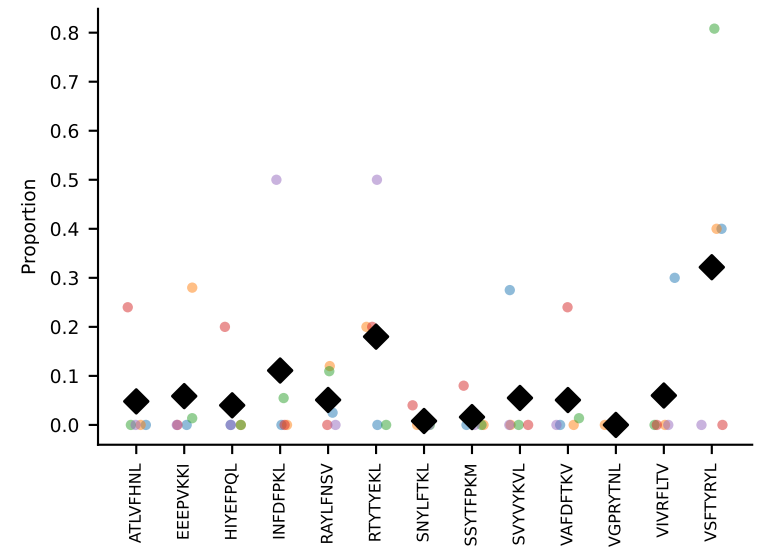
#36 AV14-3-CAARQGTQVVGQLTF-AJ5_BV1-CTCSGTGDEQYF-BJ2-7 coh=0.262, n=11
