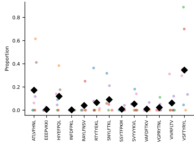
#17 AV16N-CAMREVVQGGRALIF-AJ15_BV16-CASSFVGNQDTQYF-BJ2-5 coh=0.349, n=6
