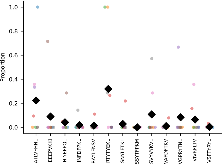
#53 AV16-CAMRETGYQNIFY-AJ49_BV13-1-CASSDAYTEVFF-BJ1-1 coh=0.196, n=21
