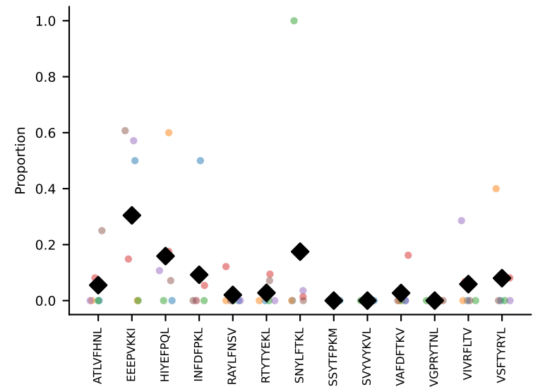
#32 AV3-3-CAVSRNTEGADRLTF-AJ45_BV17-CASSRDRADTQYF-BJ2-5 coh=0.279, n=5
