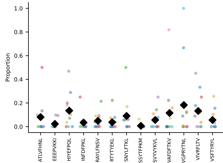
#24 AV6N-6-CALSAHYGNEKITF-AJ48_BV14-CASSFPSGQNTTEVFF-BJ1-1 coh=0.312, n=11
