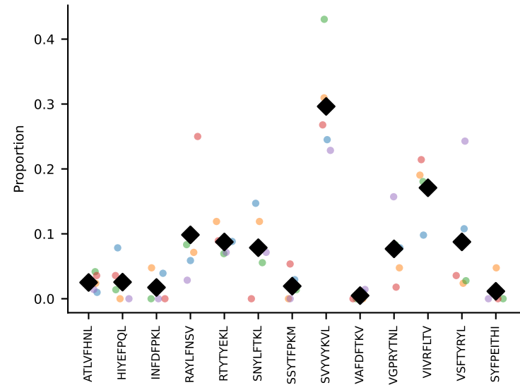
#103 AV19-CAAANTGYQNFYF-AJ49_BV17-CASSRDPWGGSAETLYF-BJ2-3 coh=0.817, n=39
