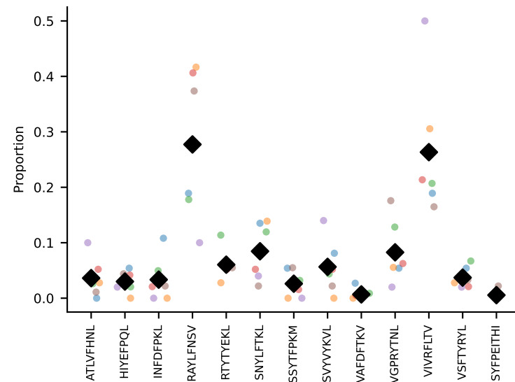
#107 AV8D-2-CATDNNNAPRF-AJ43*p03_BV1-CTCSAGQPNTGQLYF-BJ2-2 coh=0.809, n=6
