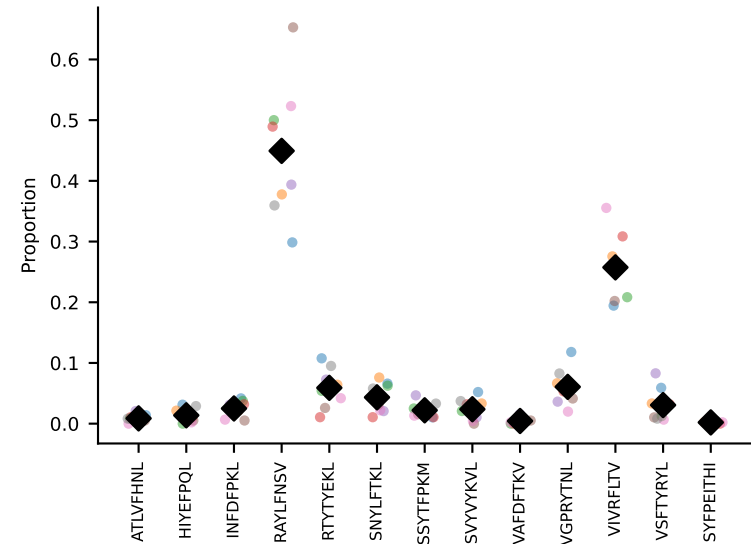
#44 AV15-1/DV6-1-CALWELASSNTDKVVF-AJ34*p03_BV3-CASSFGTGGYEQYF-BJ2-5 coh=0.955, n=10
