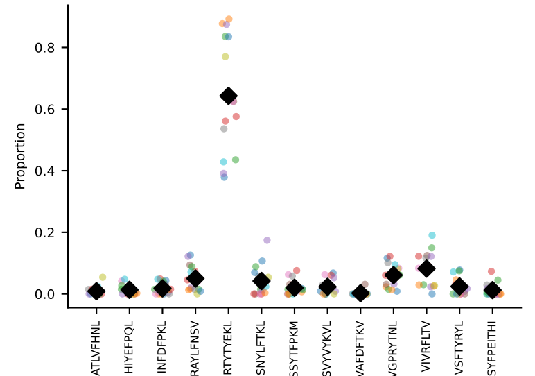
#56 AV5-1-CSASTGGFASALTFF-AJ35_BV2-CASSQDGAGANSDYTF-BJ1-2 coh=0.938, n=5
