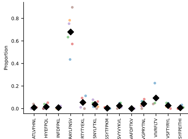
#47 AV16/DV11-CAMREGLANKMIF-AJ47_BV13-2-CASGETGGAYEQYF-BJ2-7 coh=0.953, n=5
