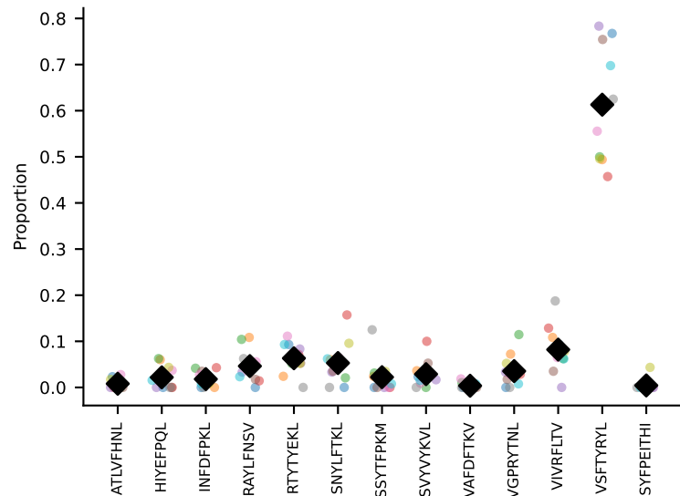
#46 AV16D/DV11-CAMREANSQYQRF-AJ13_BV1-CTCSADKVYAEQFF-BJ2-2 coh=0.955, n=12
