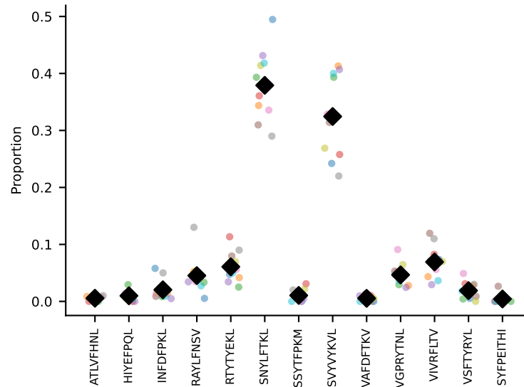
#43 AV16D/DV11-CAMRDPYGGSGNKLIF-AJ32_BV1-CTCSAVREDTQYF-BJ2-3 coh=0.958, n=6
