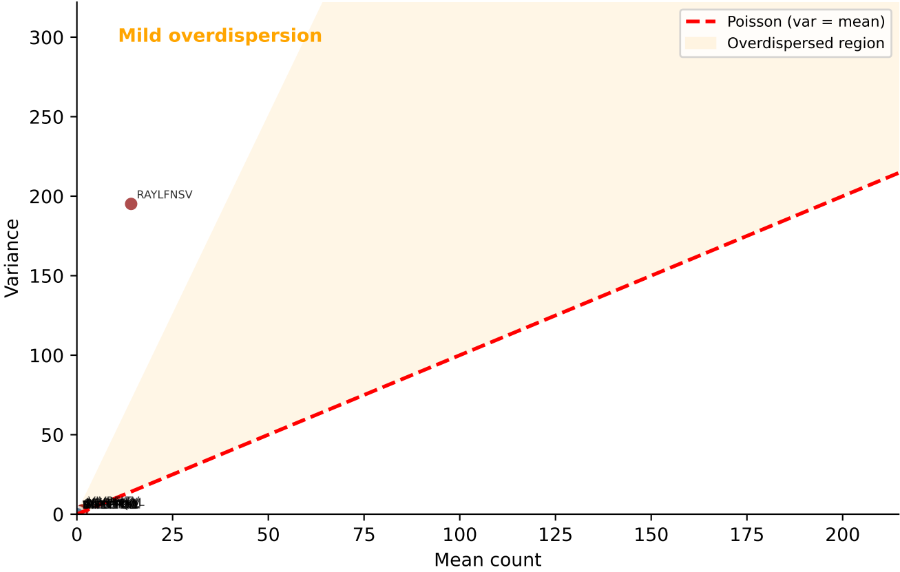
Variance vs Mean (Dispersion index: 1.54)
