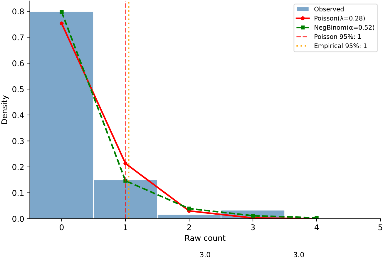
Background counts (n=60)
