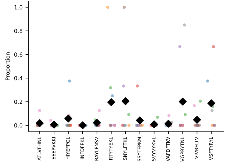
#304 AV8D-2-CATDPSSGQKLVF-AJ16_BV3-CASSLAW GASYE QYF-BJ2-7 coh=0.249, n=6
