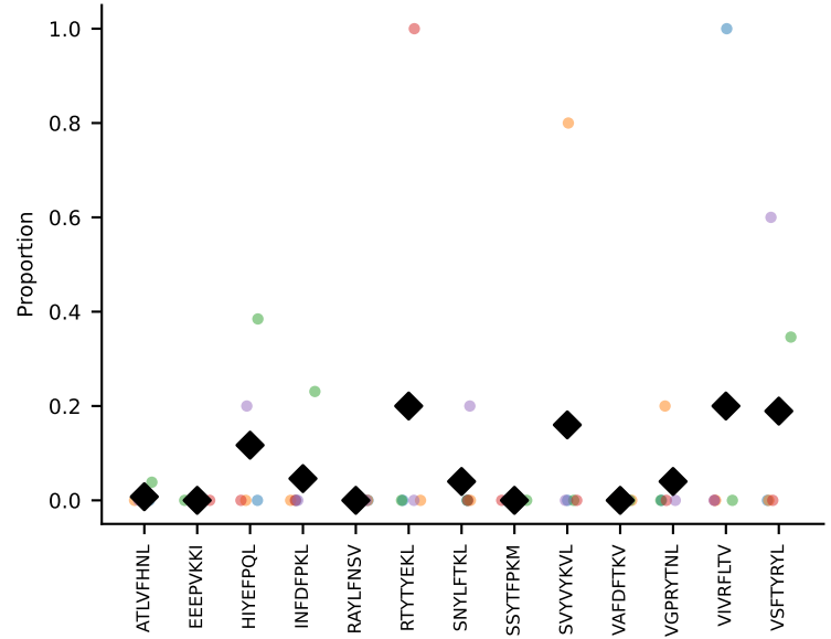
#391 AV9-4-CAVSALNAYKVIF-AJ30_BV1-CTCSAAGGDTQYF-BJ2-5 coh=0.076, n=5
