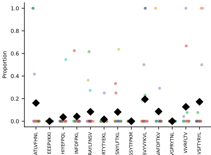
#380 AV16N-CAMREGTGGNNKLTIF-AJ56_BV1-CTCRTGTDSYNSPLYF-BJ1-6 coh=0.120, n=5
