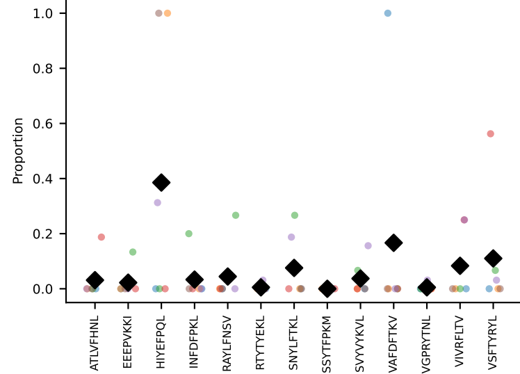
#137 AV14-2-CAASASSGSWQLIF-AJ22_BV31-CAWSLGGSAETLYF-BJ2-2 coh=0.198, n=10
