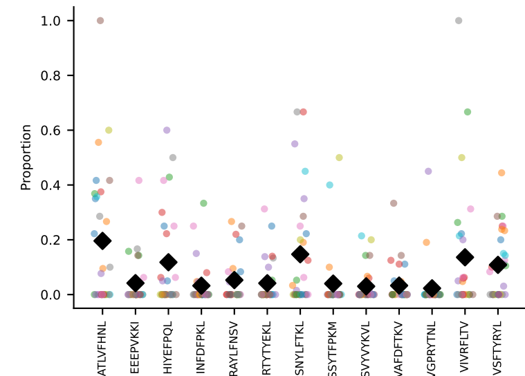
#64 AV6-4-CALVESGGGSAKLTF-AJ42_BV19-CASSMGVGNTEVFF-BJ1-1 coh=0.323, n=28
