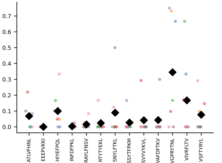
#73 AV10-CAASMDYANKMIF-AJ47_BV3-CASSPGTGYEQYF-BJ2-7 coh=0.294, n=8
