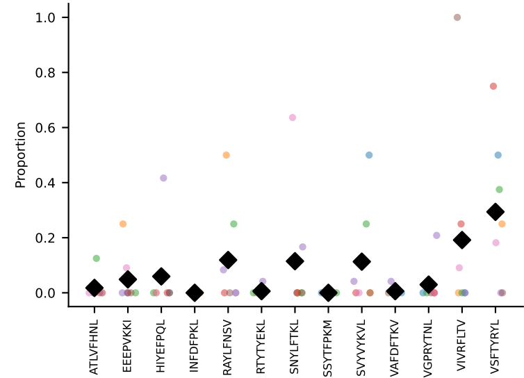
#96 AV8-1-CATDYDTNAYKVIF-AJ30_BV13-2-CASG DPIRNERLFF-BJ1-4 coh=0.256, n=11
