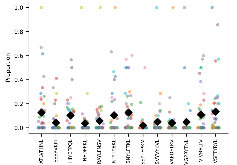
#202 AV14-3-CAASAAYANKMIF-AJ47_BV3-CASSLG PANTGQLYF-BJ2-2 coh=0.253, n=8
