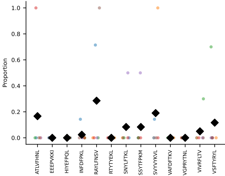
#390 AV14-3/DV8-CAAGHDTNAYKVIF-AJ30_BV13-2-CASGDAAEQYF-BJ2-7 coh=0.077, n=6
