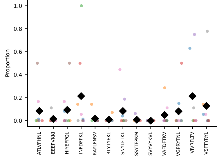
#139 AV7-3-CAVSAEGADRLTF-AJ45_BV1-CTCSADRGGNSPLYF-BJ1-1 coh=0.196, n=28 #140 AV15D-2/DV6D-2-CALSELRDRGSALGRLHF-AJ18_BV4-CASSPTGKVFF coh=0.196, n=8
