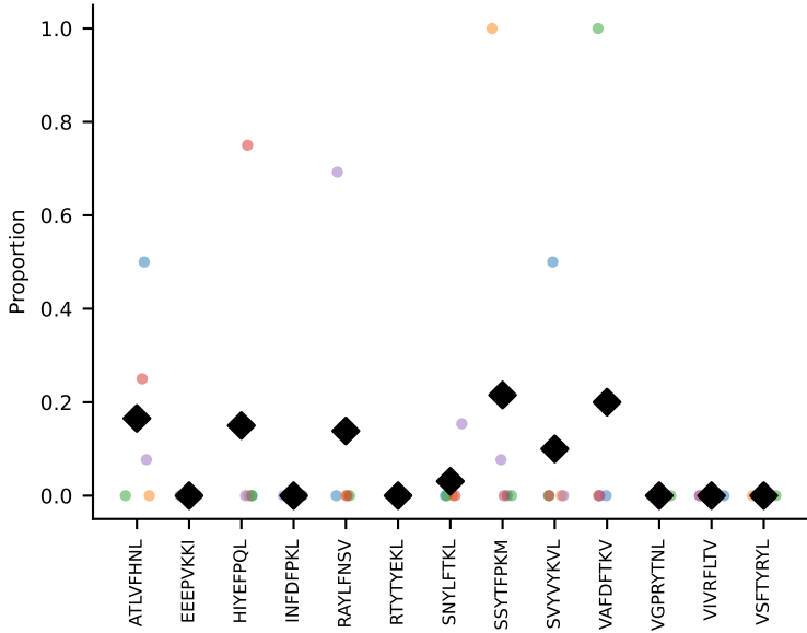
#392 AV16N-CAMREGDSNYQLIW-AJ33_BV13-2-CASGEAPSAETLYF-BJ2-7 coh=0.044, n=5
