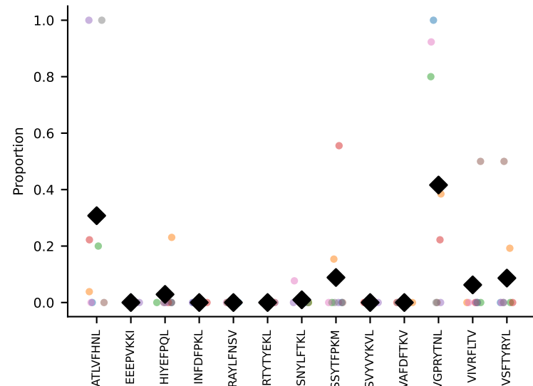
#264 AV6-5-CALSDRGSSNAKLTF-AJ42_BV17-CASSRGYNSPLYF-BJ1-6 coh=0.333, n=8
