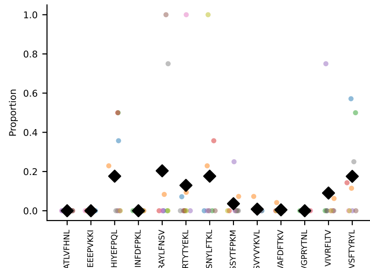
#317 AV13-1-CALGTNSAGNKLTFF-AJ17_BV2-CASSQDRVYEYF-BJ2-7 coh=0.226, n=9
