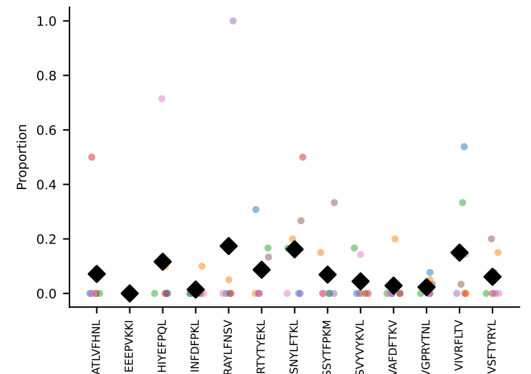
#127 AV7D-3-CAGQGGRALIF-AJ15_BV1-CTCSADQNSGNTLYF-BJ1-3 coh=0.209, n=39
