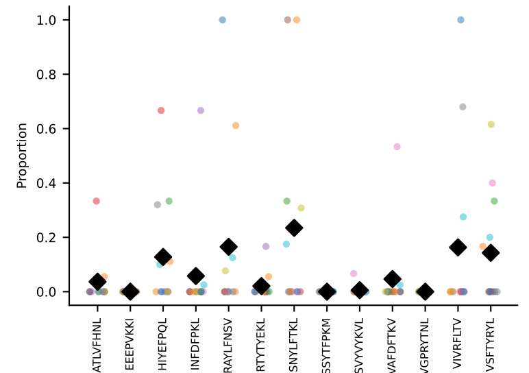
#125 AV13-2-CAIDTNTGKLTF-AJ27_BV13-2-CASGDVNTEVFF-BJ1-1 coh=0.213, n=7
