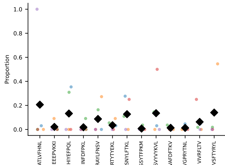
#133 AV6D-5-CALGDSGYNKLTf-AJ11_BV31-CAWSRLRGQDTQYF-BJ2-5 coh=0.205, n=15
