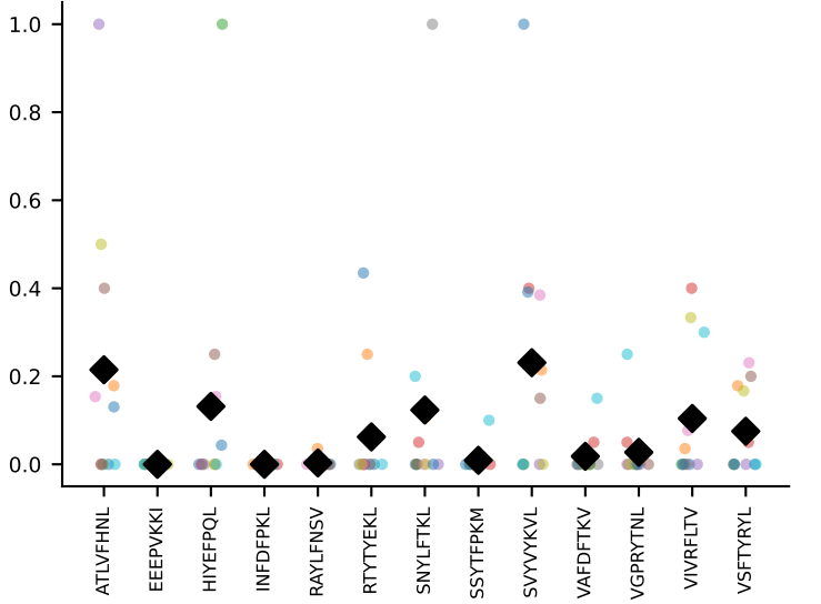
#285 AV19-CAAGLATGGNNKLTf-AJ56_BV13-1-CASSELGFSaETLYF-BJ2-7 coh=0.291, n=11
