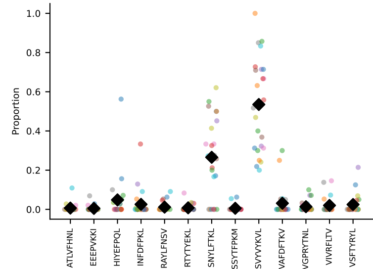
#13 AV19-CAAGNTGYQNIFY-AJ49_BV17-CASSRLGSSYEYF-BJ2-7 coh=0.713, n=6
