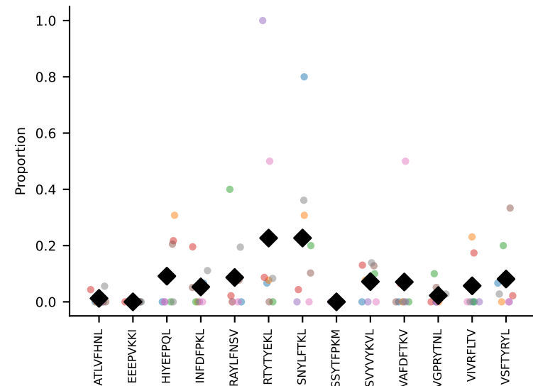
#270 AV10N-CAASPNNVLYF-AJ21_BV13-1-CASSDVGGQDQTQYF-BJ2-5 coh=0.325, n=5
