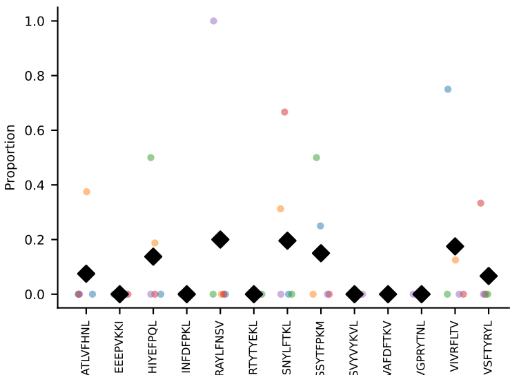
#383 AV7-3-CAVSDYNQGKLIF-AJ23_BV1-CTCSGDRVGNTLYF-BJ1-3 coh=0.108, n=5
