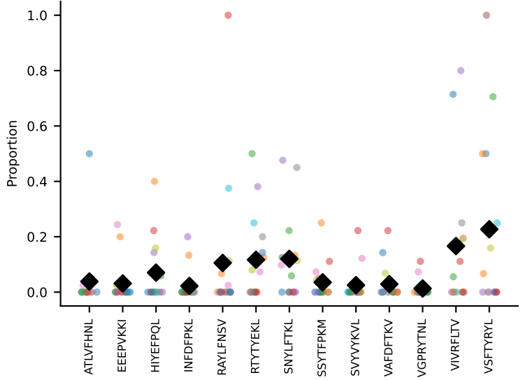
#74 AV6-6-CALGDTGGYKVVVF-AJ12_BV14-CASSFWNYAEQFF-BJ2-1 coh=0.294, n=15
