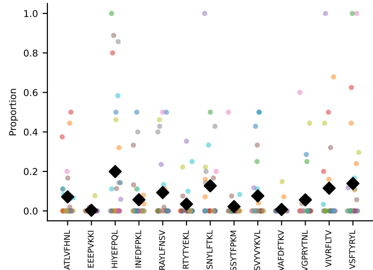
#116 AV14-2-CAASASSGSWQLIF-AJ22_BV13-1-CASSGTGGINQAPLF-BJ2-1 coh=0.229, n=32
