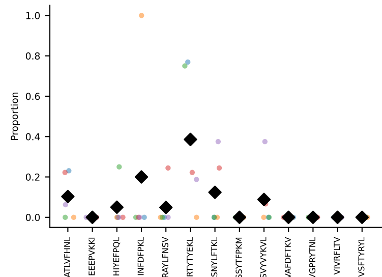
#196 AV5-1-CSASMNYNQGKLIF-AJ23_BV3-CASSLGTDEHQYF-BJ2-7 coh=0.319, n=22
