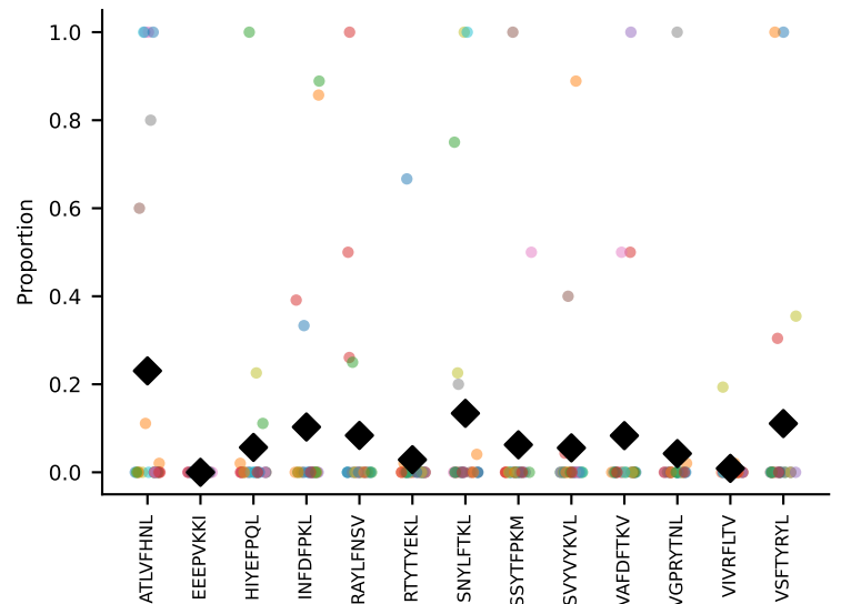
#382 AV8D-2-CATDNQGGRALIF-AJ15_BV13-1-CASSDLGVSYEQYF-BJ2-2 coh=0.116, n=10
