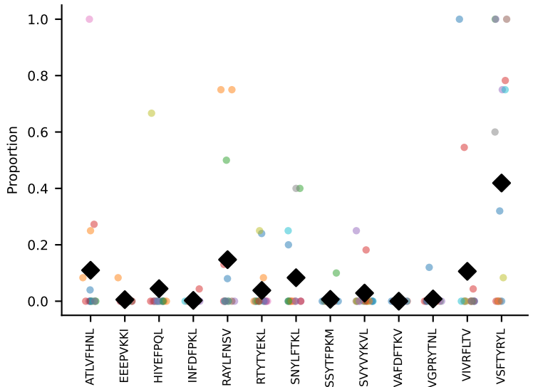
#70 AV6N-6-CALSATSSGQKLVF-AJ16_BV23-CSSSQSQTTNTEVFF-BJ1-1 coh=0.297, n=31
