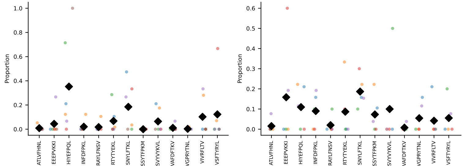
#67 AV14-1-CAAMSNNVLYF-AJ21_BV20-CGARDRNTGQLYF-BJ2-2 #276 AV13D-2-CAIDYNQGKLIF-AJ23_BV1-CTCSAVRISGNTLYF-BJ1-3 coh=0.310, n=10 coh=0.308, n=5
