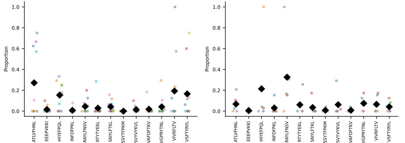
#278 AV9N-4-CALSIDTNAYKVIF-AJ30_BV31-CAWTDWGDQNTLYF-BJ2-4 #279 AV4D-3-CAADTNAYKVIF-AJ30_BV29-CASSEDNNQAPLF-BJ1-5 coh=0.305, n=5 coh=0.305, n=5
