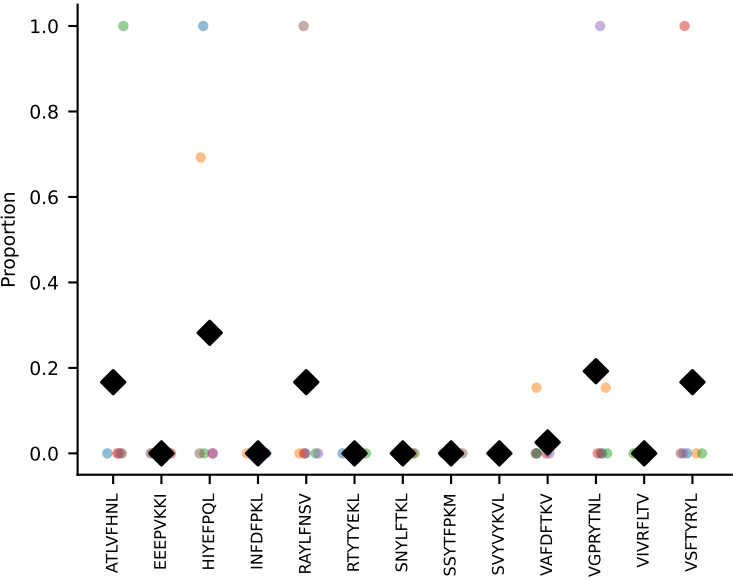
#389 AV16-CAMREGGGASSSFSKLVF-AJ50_BV16-CASSSGQYEQYF-BJ2-7 coh=0.078, n=6
