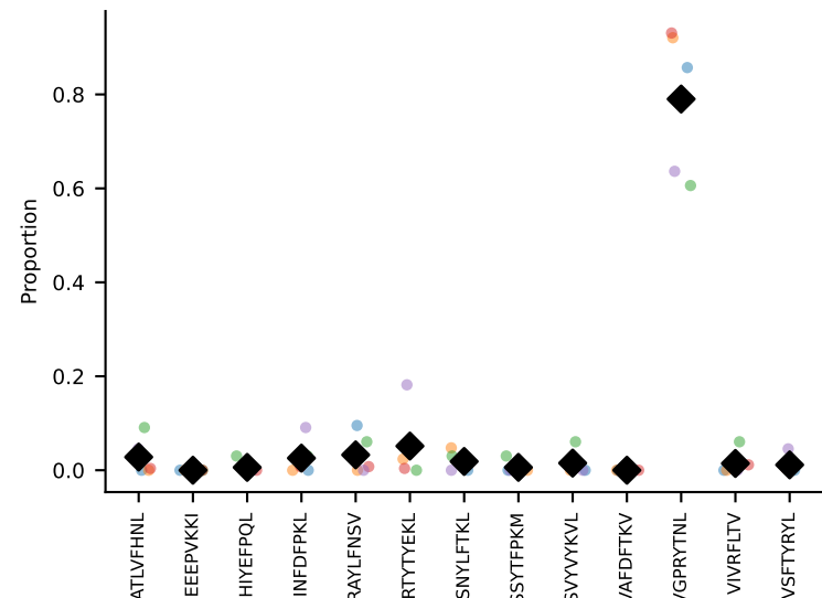
#9 AV15-1/DV6-1-CALWELNNNAGAKLTf-AJ39_BV3-CASSLGgGYEQYF-BJ2-7 coh=0.970, n=5
