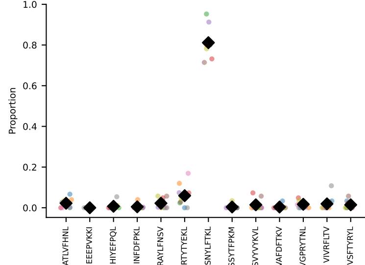
#10 AV13-2-CAIDTNTGKLTf-AJ27_BV31-CAWSLGNyAEQFF-BJ2-1 coh=0.951, n=5
