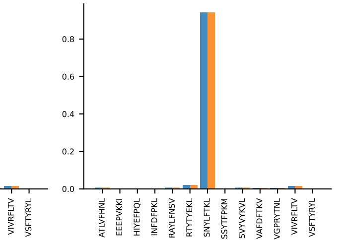
AV11-CVVGANNYAQGLTf-AJ26_BV13-2-CASGDVGGNSPLYf-BJ1-6 PROP n:5→5
