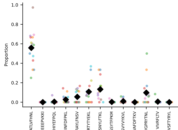
#32 AV16/DV11-CAMRENTGGLSGKLTF-AJ2_BV13-1-CASSDEQYNNQAPLF-BJ2-1 coh=0.730, n=7
