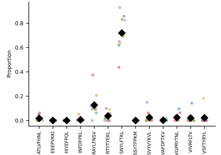
#24 AV6-7/DV9-CALSVDNSNYQLIW-AJ33_BV13-2-CASGLGGDTQYF-BJ2-4 coh=0.858, n=38
