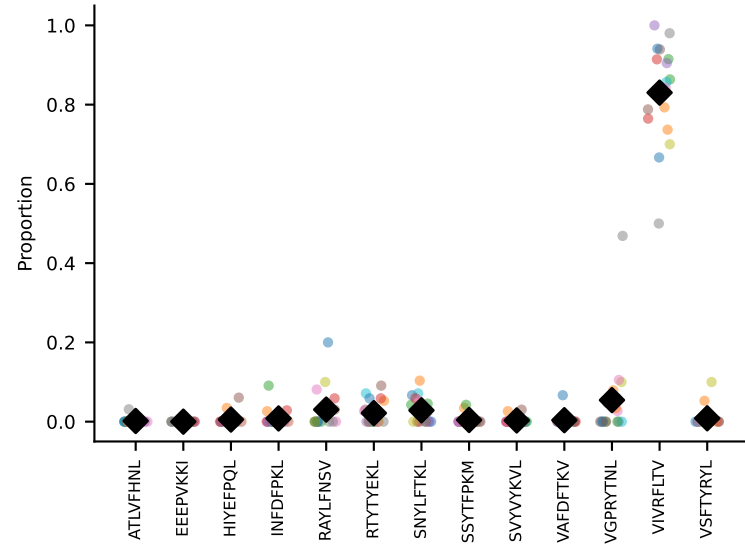
#18 AV9-2-CAPIASSFSKLVF-AJ50_BV13-2-CASGDVGGANERLFF-BJ1-4 coh=0.943, n=7
