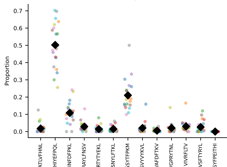
#11 AV4-3-CAGTGNT RKLIF-AJ37*p02_BV4-CASSPGTG YAEQFF-BJ2-1 coh=0.914, n=21
