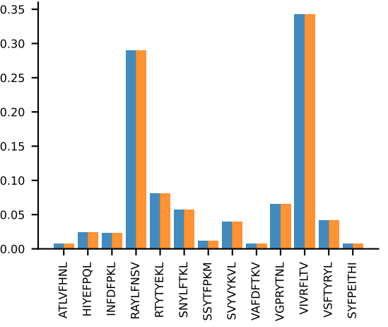
AV12-2-CALSDRYGNEKITF-AJ48_BV29-CASSPLKGANSDYTF-BJ1-1AV12-2-CALSDRYGNEKITF-AJ48_BV29-CASSPLKGANSDYTF-BJ1-1 PROP n:6→6
