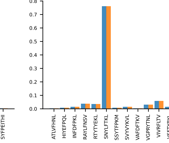
AV7-3-CAVNAYKVIF-AJ30_BV13-2-CASGDLGGRDAETLYF-BJ2-3AV7-3-CAVNAYKVIF-AJ30_BV13-2-CASGDLGGRDAETLYF-BJ2-3 PROP n:6→6
