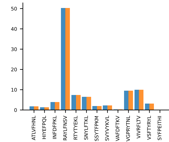
AV6-5-CALSDGGTGSKLSF-AJ58_BV17-CASSPGLGGRFNEQYF-BJ2-2AV6-5-CALSDGGTGSKLSF-AJ58_BV17-CASSPGLGGRFNEQYF-BJ2-2 MEAN n:6→6
