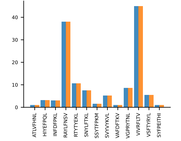
AV12-2-CALSDRYGNEKITF-AJ48_BV29-CASSPLKGANSDYTF-BJ1-1AV12-2-CALSDRYGNEKITF-AJ48_BV29-CASSPLKGANSDYTF-BJ1-1 MEAN n:6→6
