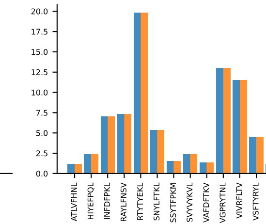
AV7-3-CAVNAYKVIF-AJ30_BV13-2-CASGDLGGRDAETLYF-BJ2-3AV7-3-CAVNAYKVIF-AJ30_BV13-2-CASGDLGGRDAETLYF-BJ2-3 MEAN n:6→6
