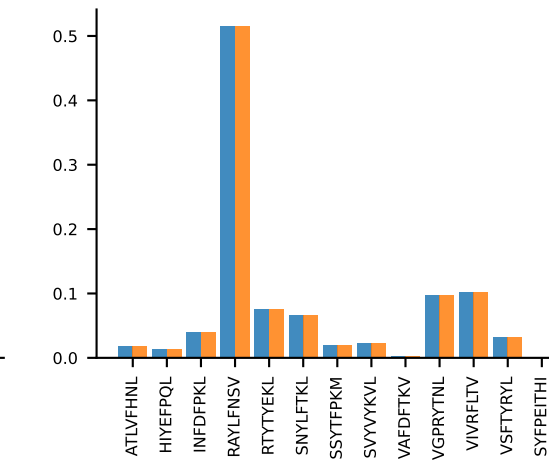
AV6-5-CALSDGGTGSKLSF-AJ58_BV17-CASSPGLGGRFNEQYF-BJ2-2AV6-5-CALSDGGTGSKLSF-AJ58_BV17-CASSPGLGGRFNEQYF-BJ2-2 PROP n:6→6
