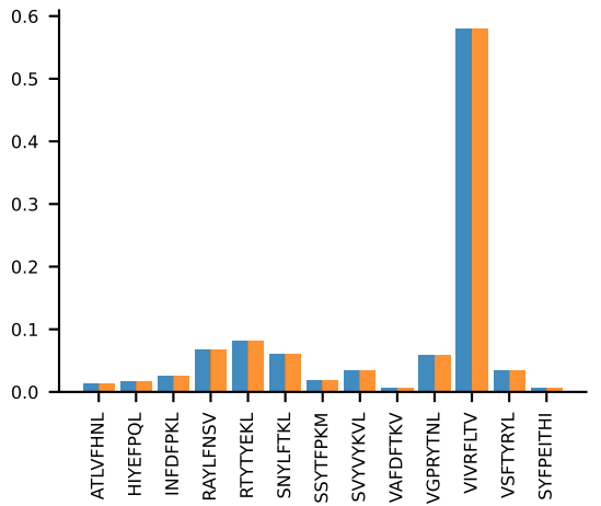
AV14-1-CAARGDNRIFF-AJ31_BV1-CTCSANRVNDNQAPLF-BJ1-5AV14-1-CAARGDNRIFF-AJ31_BV1-CTCSANRVNDNQAPLF-BJ1-5 PROP n:6→6
