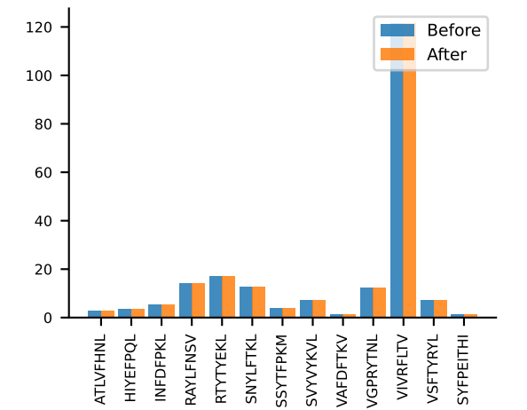
AV14-1-CAARGDNRIFF-AJ31_BV1-CTCSANRVNDNQAPLF-BJ1-5AV14-1-CAARGDNRIFF-AJ31_BV1-CTCSANRVNDNQAPLF-BJ1-5 MEAN n:6→6
