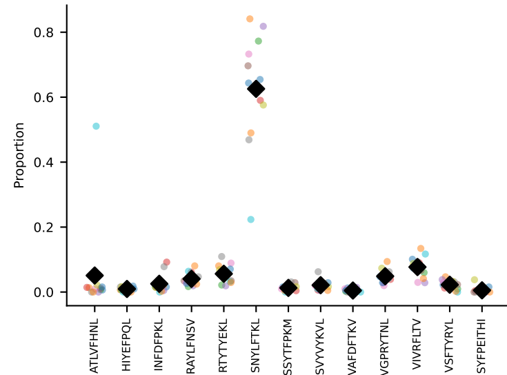
#68 AV6-1-CVLVPSSGSWQLIF-AJ22_BV13-3-CASSDQNSDYTF-BJ1-2 coh=0.881, n=8
