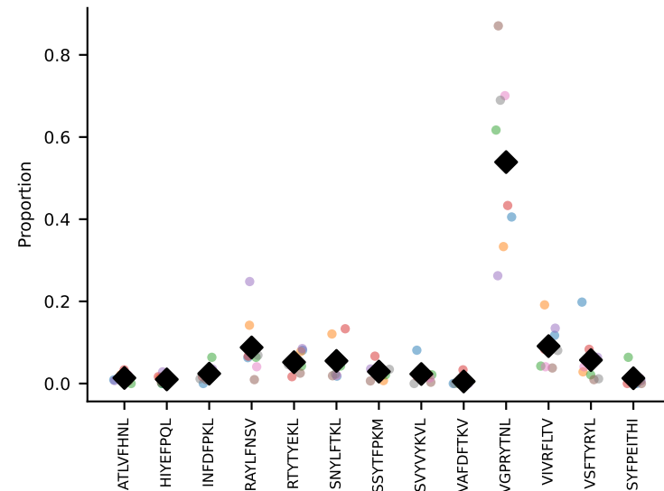
#72 AV16D/DV11-CAMREGNTGNYKYVF-AJ40_BV13-2-CASGDLYEQYF-BJ2-1 coh=0.857, n=17
