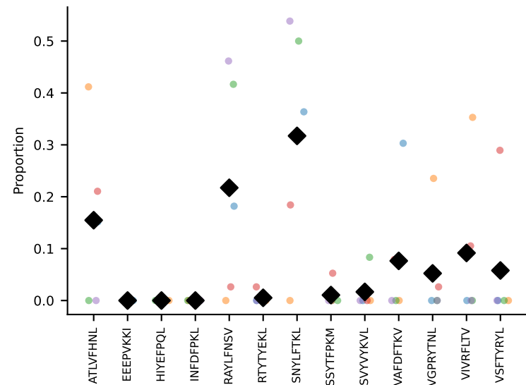
#9 AV16N-CAMREGDSNYQLIW-AJ33_BV13-2-CASGDRANSDYTF-BJ1-2 coh=0.448, n=5
