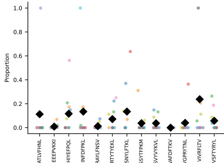
#47 AV14-2-CAASGTEGADRLTF-AJ45_BV1-CTCSAVRVTGQLYF-BJ2-2 coh=0.232, n=6
