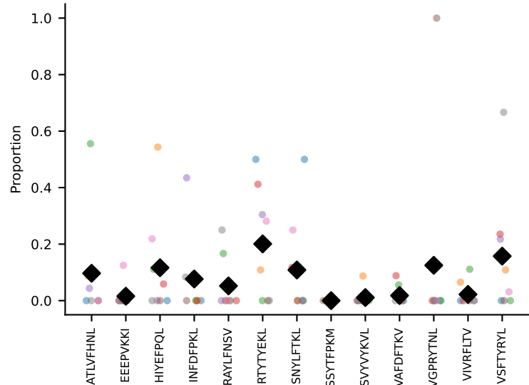
#38 AV12D-2-CALSDDYAQGLTF-AJ26_BV14-CASSPNRVGEQYF-BJ2-7 coh=0.247, n=8
