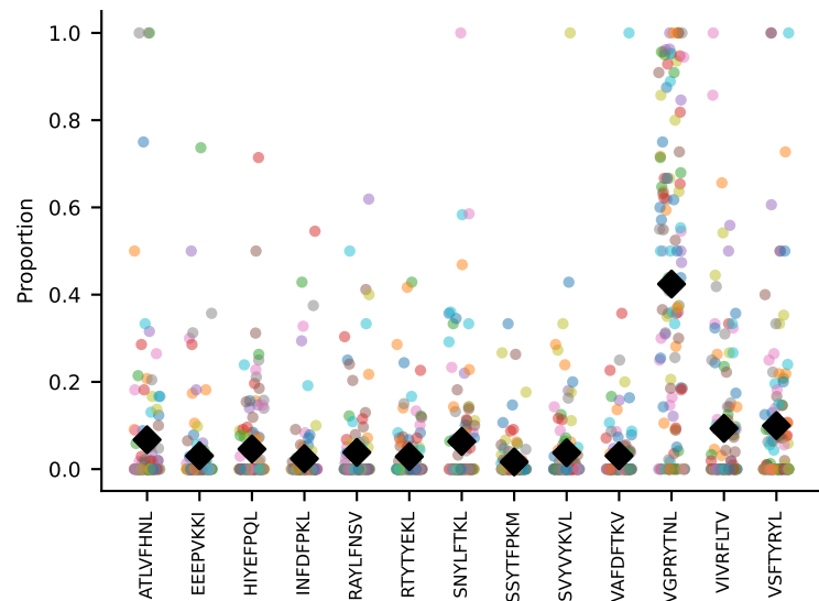
#11 AV16N-CAMRDNYAQLTF-AJ26_BV3-CASSLGPSSYEYF-BJ2-7 coh=0.436, n=122
