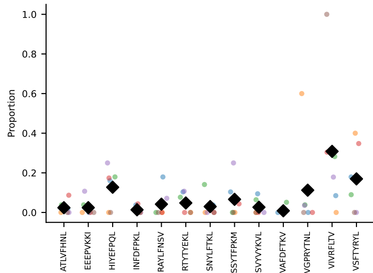
#12 AV14-2-CAAENSAGNKLTF-AJ17_BV3-CASSLGTGYEQYF-BJ2-7 coh=0.434, n=5
