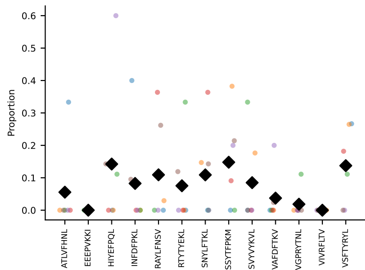
#35 AV9D-2-CVLSDNYAQLTF-AJ26_BV1-CTCSAGLGEGAETLYF-BJ2-3 coh=0.265, n=6
