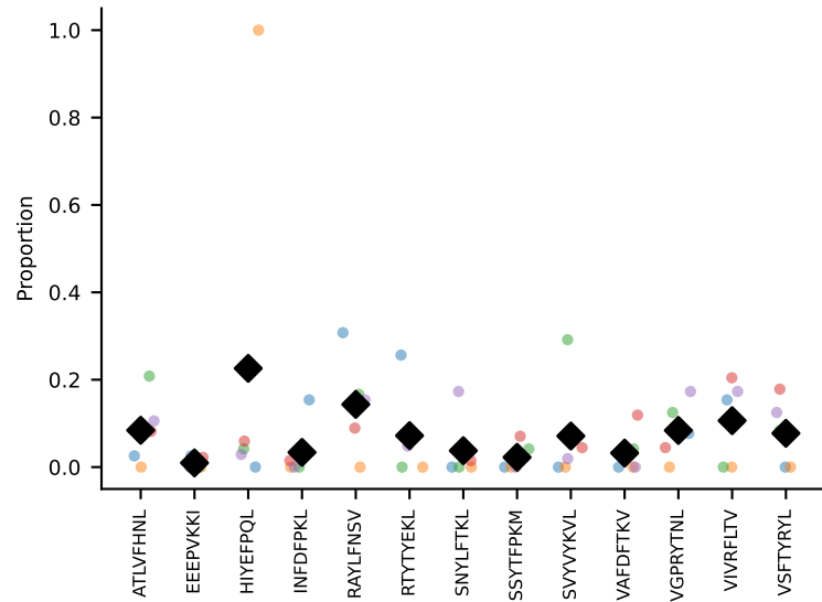
#20 AV14-2-CAASVAMGYLTF-AJ9_BV19-CASSIEERLFF-BJ1-4 coh=0.333, n=6
