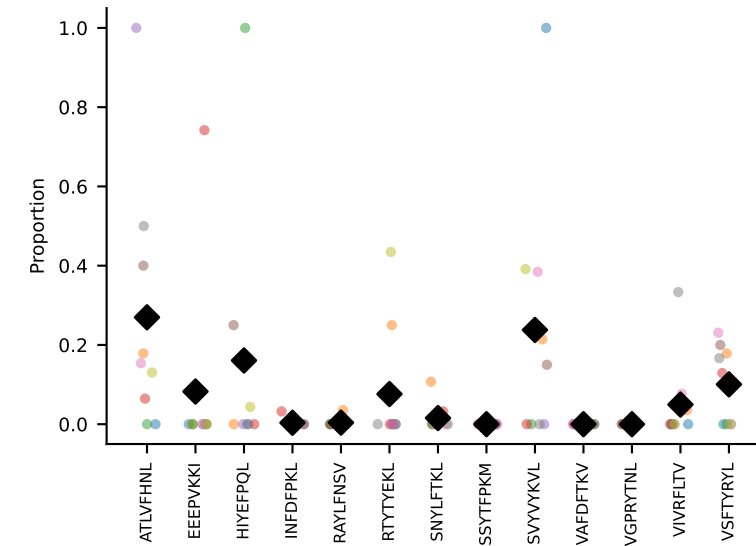
#21 AV19-CAAGLATGGNNKLTF-AJ56_BV13-1-CASSELGFS AETLYF-BJ2-3 coh=0.327, n=9
