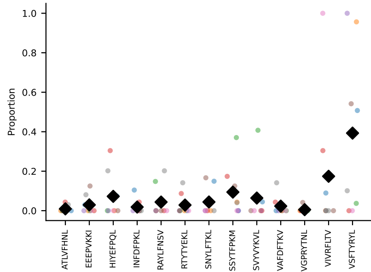
#23 AV16N-CAMREDQGGRALIF-AJ15_BV16-CASSLVGAQDTQYF-BJ2-5 coh=0.323, n=9
