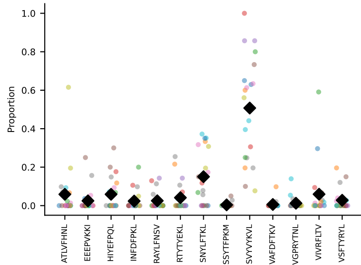
#7 AV16N-CAMREGNSNNRIFF-AJ31_BV13-1-CASRDINTEVFF-BJ1-1 coh=0.475, n=6
