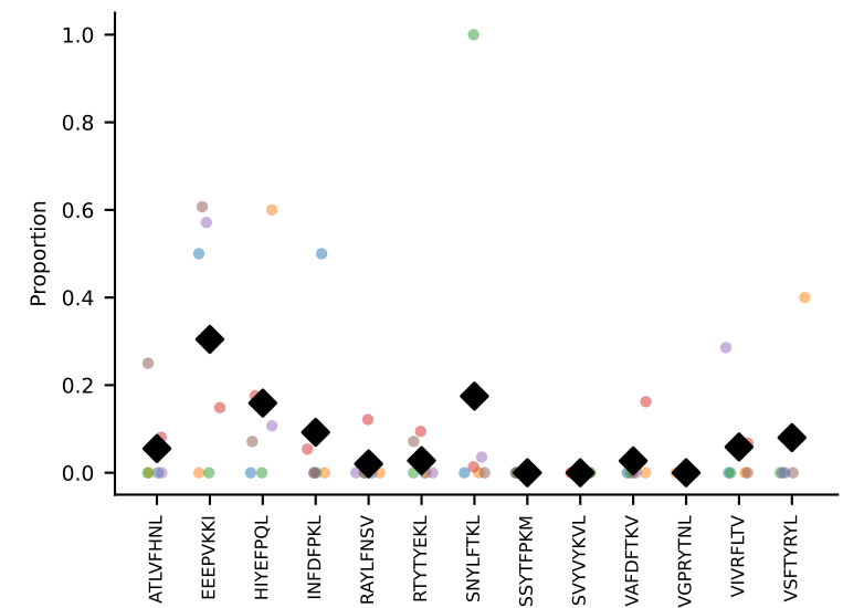
#32 AV3-3-CAVSRNTEGADRLTF-AJ45_BV17-CASSRDRADTQYF-BJ2-5 coh=0.279, n=5
