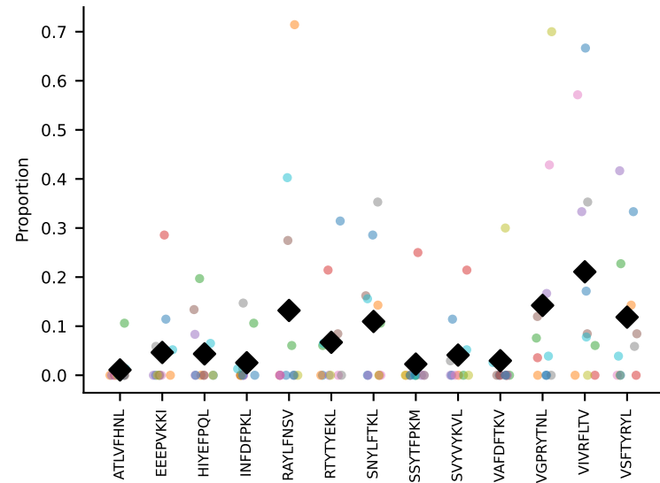
#22 AV14-2-CAASPYTGNYKYVF-AJ40_BV13-2-CASGDVGGLYF-BJ1-3 coh=0.327, n=11
