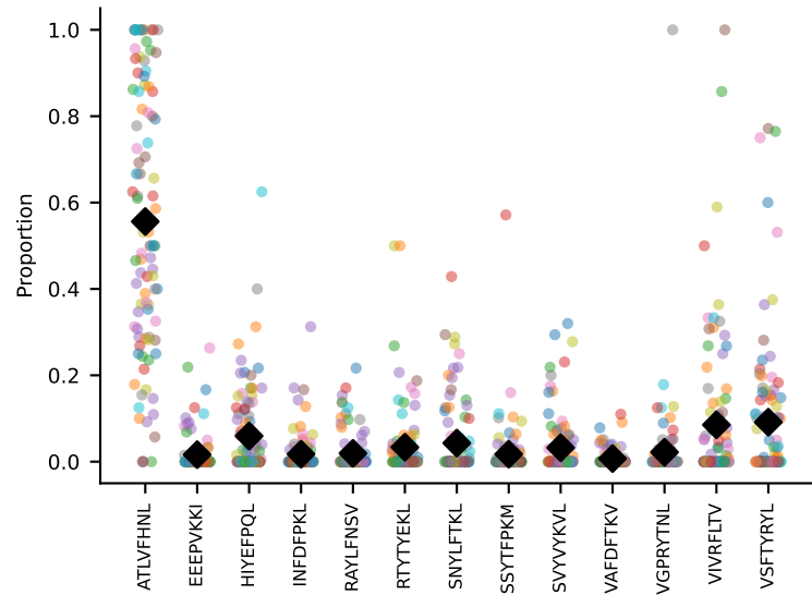
#8 AV8-1-CATSASSGSWQLIF-AJ22_BV13-2-CASGDEISNERLFF-BJ1-4 coh=0.451, n=6
