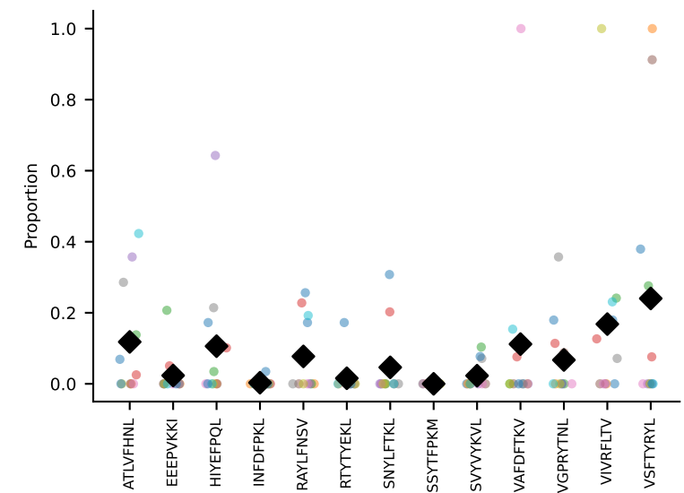
#36 AV14-3-CAARQGTQVVGQLTF-AJ5_BV1-CTCSGTGDEQYF-BJ2-7 coh=0.262, n=11
