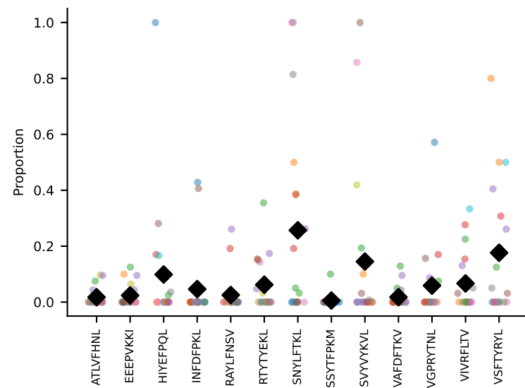
#33 AV14-3-CAASAGSGGKLT-AJ44_BV3-CASSLDFGQNTLYF-BJ2-4 coh=0.279, n=18
