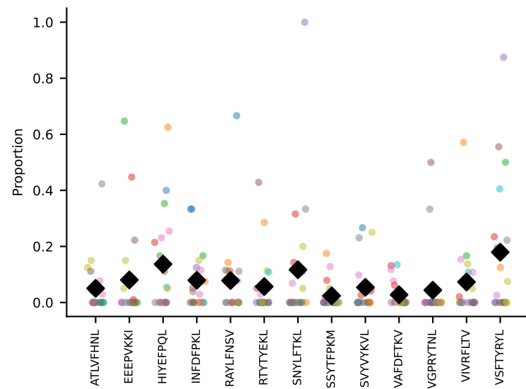
#30 AV13-1-CALERSNNRIFF-AJ31_BV2-CASSQDRRGDEQYF-BJ2-7 coh=0.294, n=5
