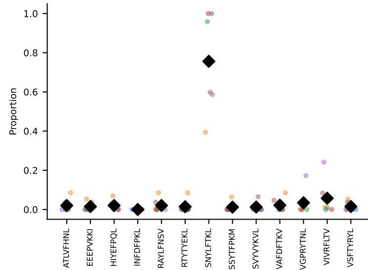
#5 AV7-6-CAVGYQNFYF-AJ49_BV4-CASSDRDINYAEQFF-BJ2-1 coh=0.615, n=11
