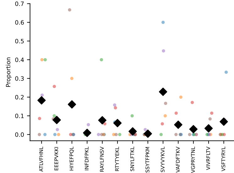
#29 AV9-2-CVLSTGSGGKLT-AJ44_BV14-CASSFANTGQLYF-BJ2-2 coh=0.296, n=22
