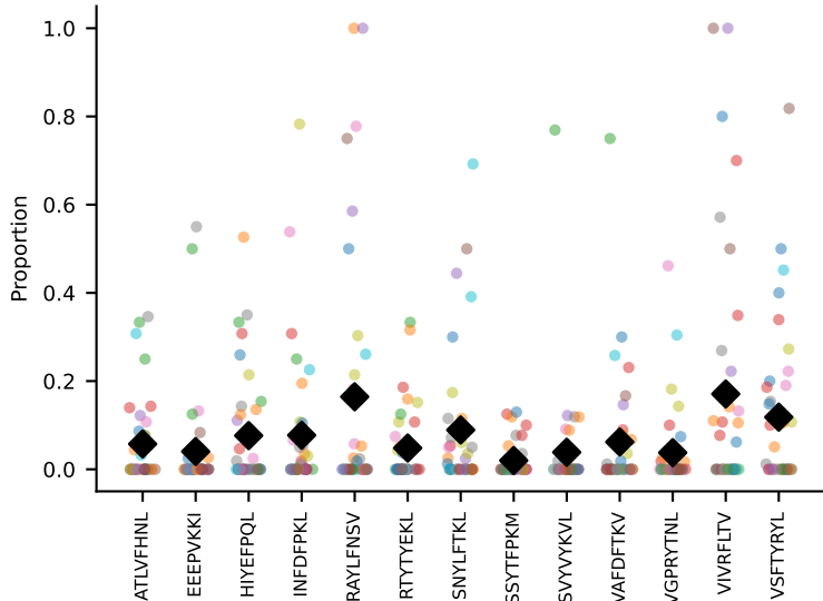
#37 AV9-4-CAVSGNYNVLYF-AJ21_BV13-1-CASRTGGHEQYF-BJ2-7 coh=0.256, n=36
