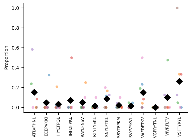
#34 AV4D-3-CAAYQGGRALIF-AJ15_BV1-CTCSGDRVAEQFF-BJ2-1 coh=0.268, n=7
