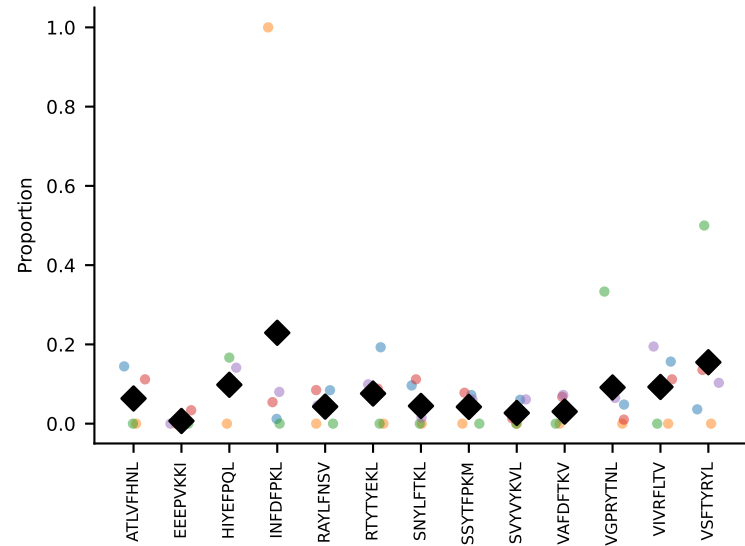
#18 AV13D-2-CAIDRQGGRALIF-AJ15_BV13-1-CASSRTGVNQAPLF-BJ1-5 coh=0.345, n=9
