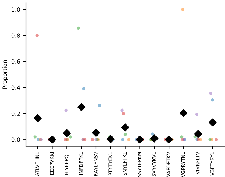
#64 AV12-2-CALSDDGSGGKLTLL-AJ44_BV1-CTCSADGGLATEVFF-BJ1-1 coh=0.127, n=5
