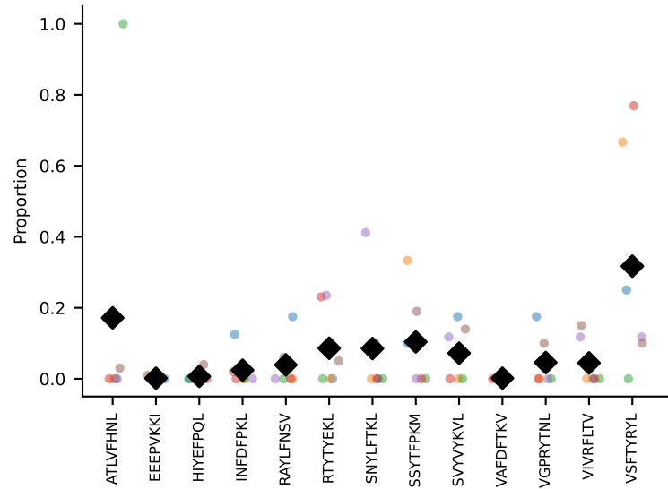
#24 AV6N-6-CALSAHYGNEKITF-AJ48_BV14-CASSFPSGQNTVEFF-BJ1-1 coh=0.312, n=11
