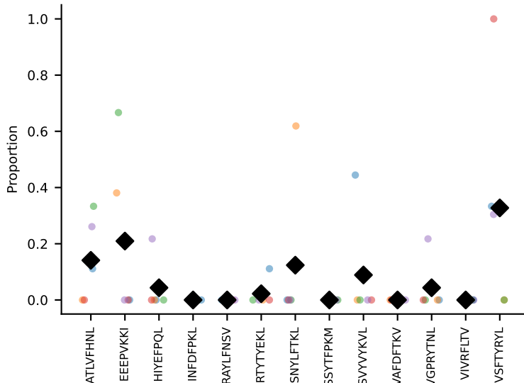
#45 AV19-CAAGADYANKMIF-AJ47_BV3-CASSLTVNQDTQYF-BJ2-5 coh=0.233, n=8
