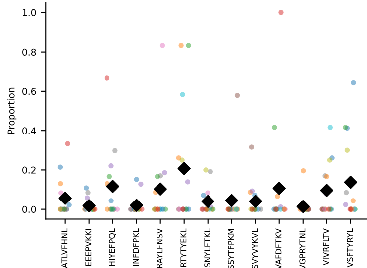
#39 AV8D-2-CATEYQGGRALIF-AJ15_BV19-CASSIGTNERLFF-BJ1-4 coh=0.245, n=14
