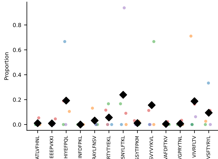
#46 AV13D-1-CAMERSNNRIFF-AJ31_BV2-CASSQDRRGDTQYF-BJ2-5 coh=0.232, n=10
