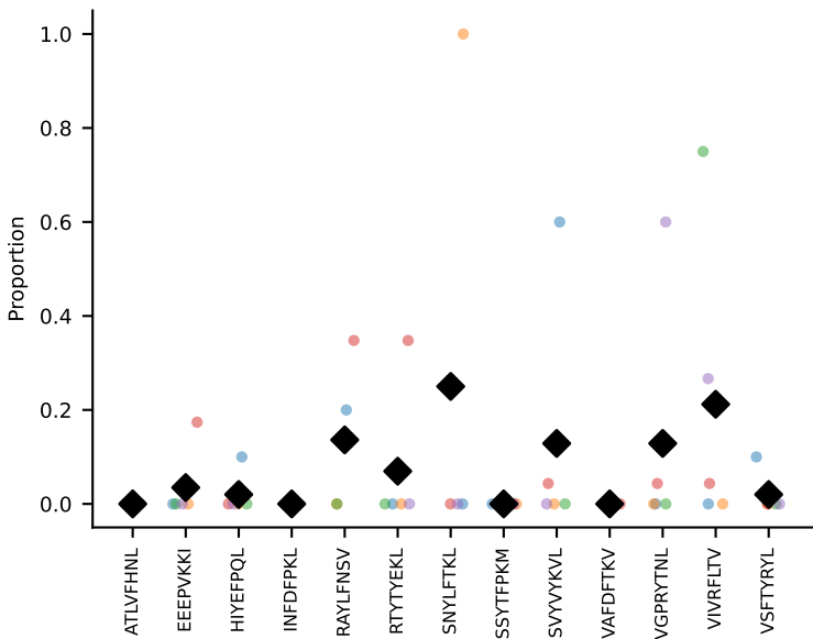
#63 AV7D-5-CAVRDSGYNKLTFF-AJ11_BV1-CTCSADRLGNTLYF-BJ2-4 coh=0.135, n=5
