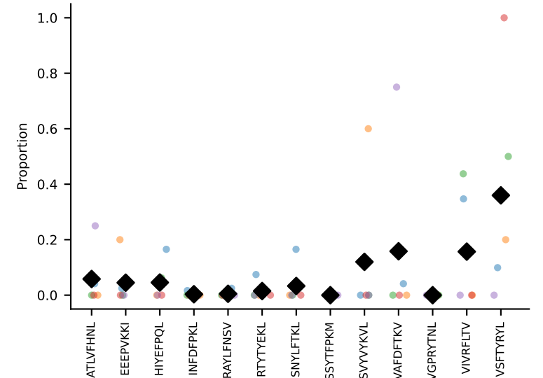
#40 AV6-6-CALGMSNYNVLYF-AJ21_BV13-2-CASGDEGPQDTQYF-BJ2-5 coh=0.242, n=5
