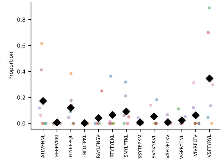
#17 AV16N-CAMREVYQGGRALIF-AJ15_BV16-CASSFVGNQDTQYF-BJ2-5 coh=0.349, n=6
