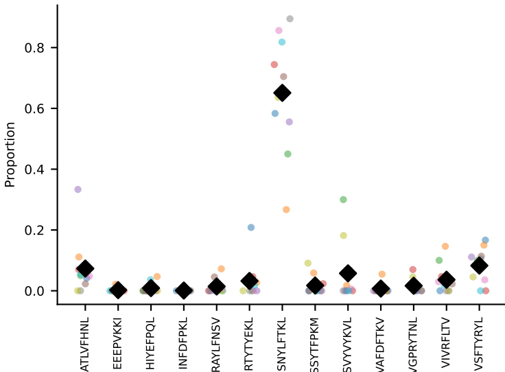
#5 AV6N-6-CARASSGSWQLIF-AJ22_BV13-1-CASSDAGTEVFF-BJ1-1 coh=0.645, n=6
