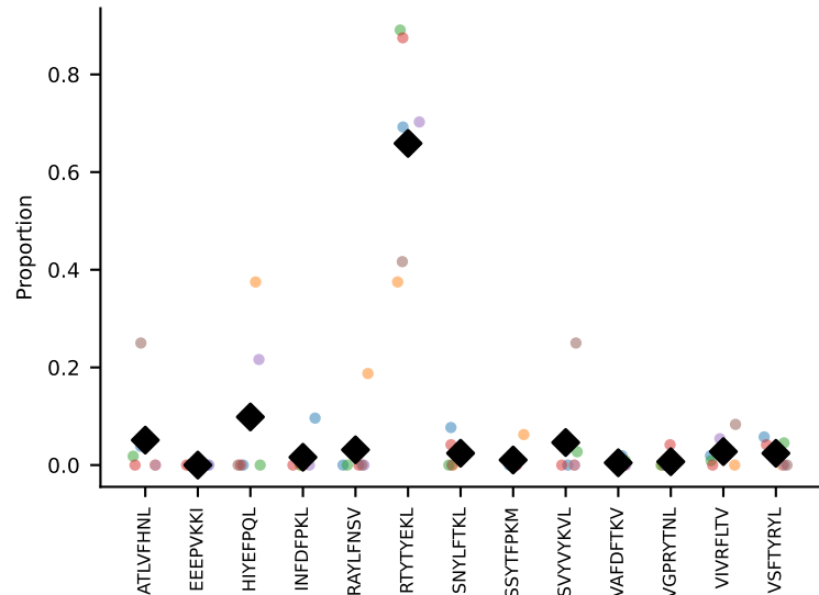
#6 AV16-CAMREANTGYQNIFY-AJ49_BV13-2-CASGTGGQNTLYF-BJ2-4 coh=0.622, n=19
