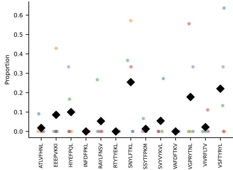
#48 AV7-2-CAADNVGDNSKLIW-AJ38_BV4-CASSPGTGYSYDTF-BJ1-2 coh=0.295, n=5
