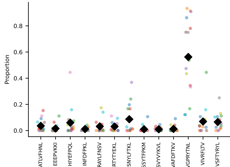
#8 AV4-3-CAAYGSSGNKLIF-AJ32_BV17-CASSSLGGFYAEQFF-BJ2-1 coh=0.614, n=5
