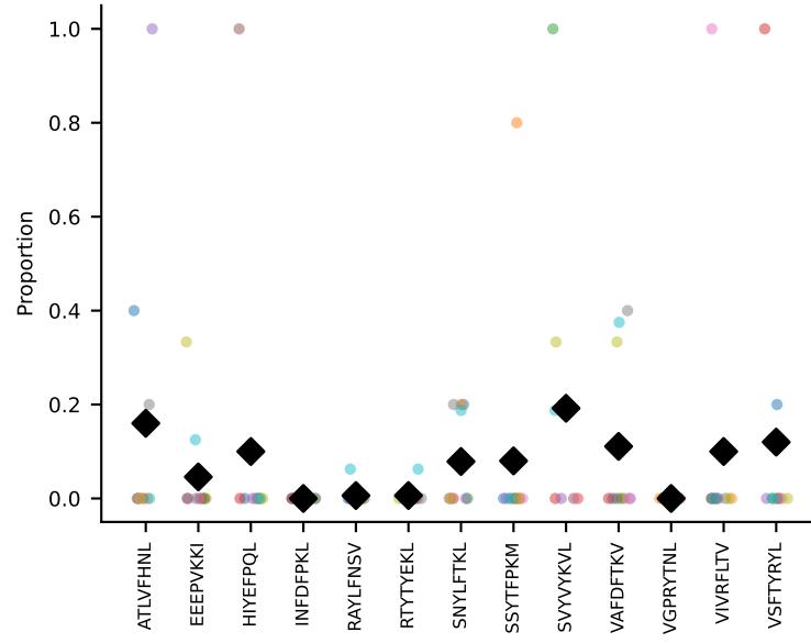
#67 AV2-CIVTDMNYNQGKLIF-AJ23_BV19-CASSPTGPNSDYTF-BJ1-2 coh=0.154, n=10
