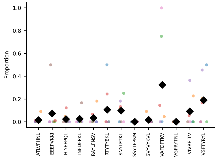
#44 AV6-6-CALGDTGGYKVVF-AJ12_BV14-CASSFWNYAEQFF-BJ2-1 coh=0.309, n=11
