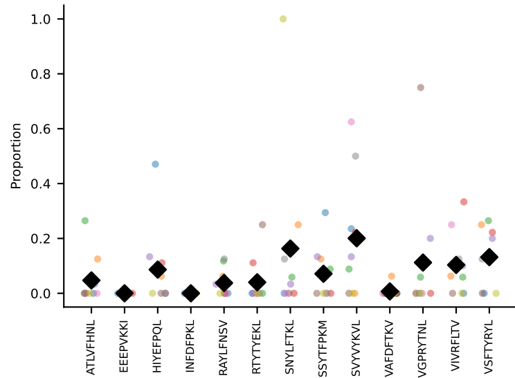
#43 AV3D-3-CAAGTGGYKVVF-AJ12_BV26-CASSLGS LNQDTQYF-BJ2-5 coh=0.311, n=8
