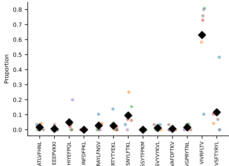
#7 AV16-CAMRESNTGYQNIFY-AJ49_BV13-2-CASGTGGQNTLYF-BJ2-4 coh=0.618, n=84
