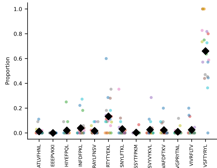
#16 AV12D-2-CALNQGGSAKLIF-AJ57_BV1-CTCSADWGNVYAEQFF-BJ2-5 coh=0.818, n=21
