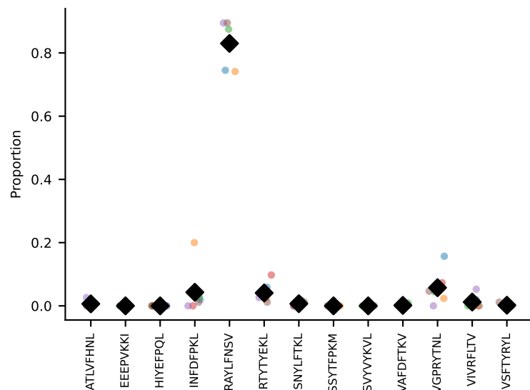
#46 AV9-2-CVLSSTSGGNYPKTF-AJ6_BV1-CTCSAVRVDTEVFF-BJ1-1 coh=0.982, n=6
