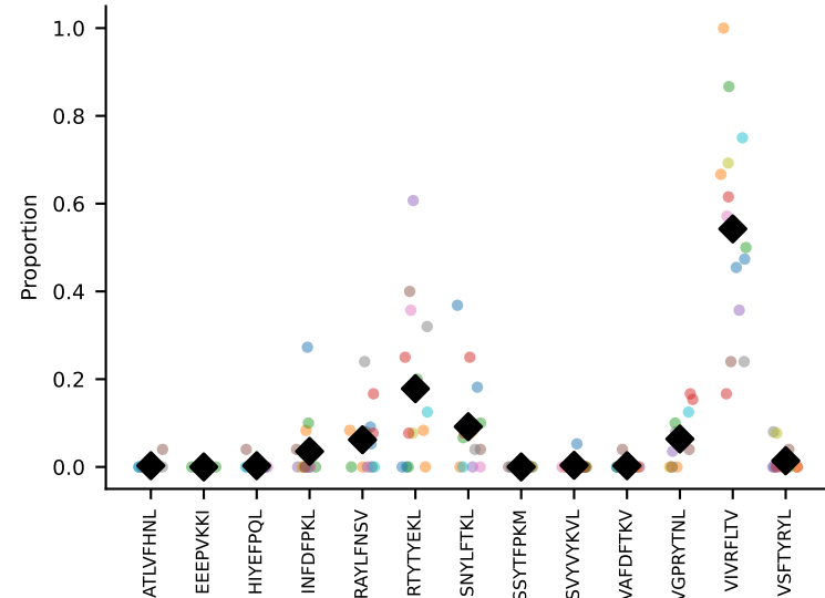
#181 AV4-3-CAAEASTGNYKYVF-AJ40_BV3-CASSLVQVTEVFF-BJ1-1 coh=0.753, n=14
