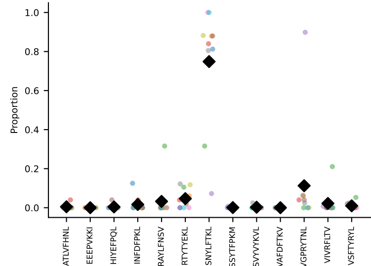
#184 AV13-2-CAIDTNTGKLTF-AJ27_BV13-3-CASSDANSDYTF-BJ1-2 coh=0.750, n=10
