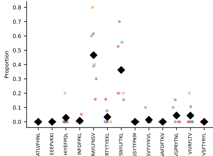
#183 AV7N-4-CAVSEPGTQVVGQLTF-AJ5_BV1-CTCSAGGSYAEQFF-BJ2-1 coh=0.752, n=7
