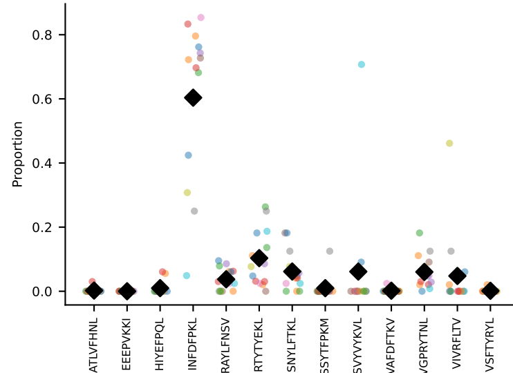
#182 AV9-2-CVLSDDTNAYKVIF-AJ30_BV31-CAWTDWGDQNTLYF-BJ2-4 coh=0.752, n=14
