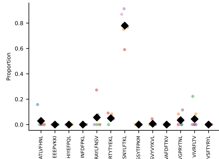
#81 AV16/DV11-CAMRESNTGYQNIFY-AJ49_BV13-2-CASGEGQGKNTLYF-BJ2-4 coh=0.953, n=7
