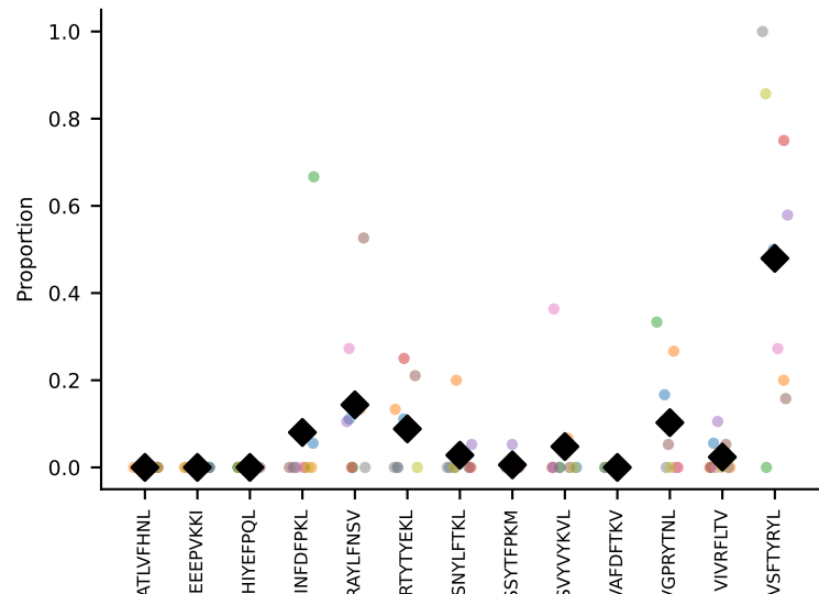
#438 AV14-2-CAASSNNRIF-AJ31_BV13-2-CASGGGWGTEVFF-BJ1-1 coh=0.524, n=19
