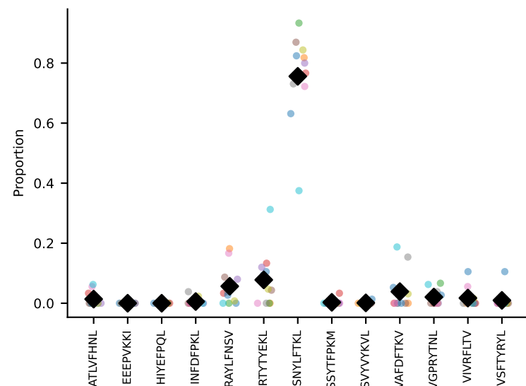
#288 AV16-CAMREANTGYQNIFY-AJ49_BV13-2-CASGPGGQNTLYF-BJ2-4 coh=0.932, n=59
