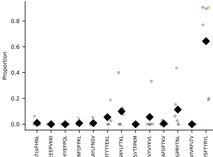
#428 AV16-CAMREGASSSFASKLVF-AJ50_BV29-CASSLGGLYAEQFF-BJ2-7 coh=0.630, n=6
