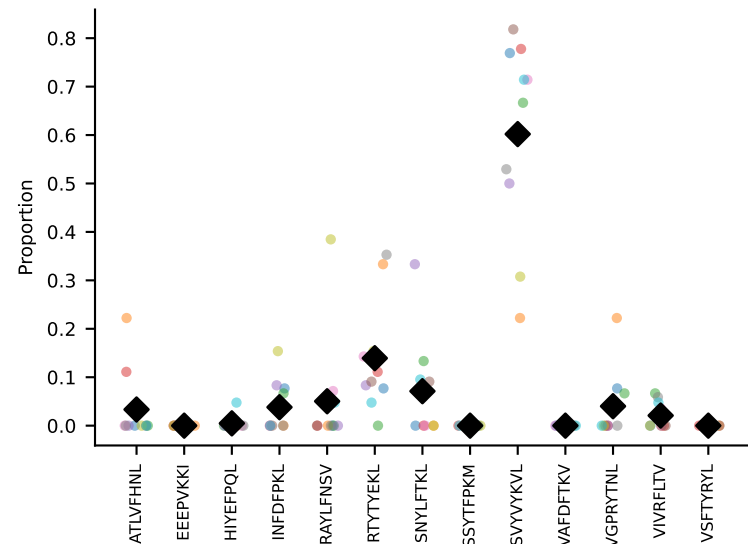
#413 AV14-2-CAASADTGNYKYVF-AJ40_BV13-3-CASSDMGGQNTLYF-BJ2-3 coh=0.781, n=8
