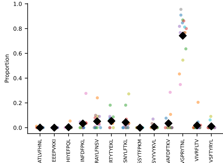
#180 AV14-2-CAATNTGKLTF-AJ27_BV13-2-CASGDVGGSNERLFF-BJ1-4 coh=0.906, n=8
