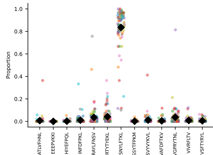
#181 AV8-1-CATEGYQNIFY-AJ49_BV12-1-CASSLTGGGYEQYF-BJ2-7 coh=0.905, n=45
