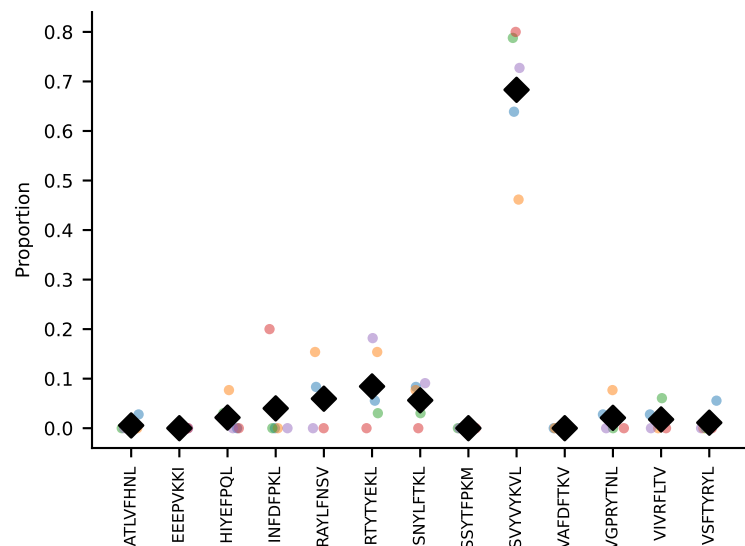
#395 AV16N-CAMREGSSGSWQLIF-AJ22_BV13-2-CASGVQGSATLYF-BJ1-4 coh=0.940, n=5
