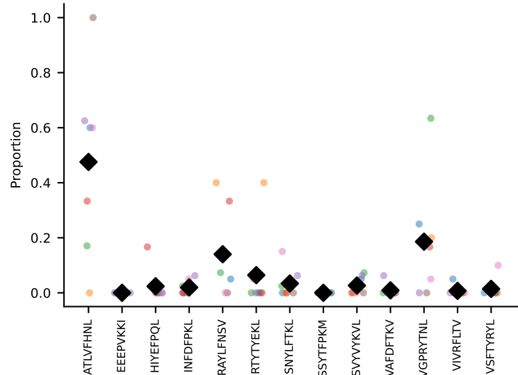
#437 AV16N-CAMRASSGSWQLIF-AJ22_BV1-CTCSASGTGDNSPLYF-BJ1-1 coh=0.537, n=9
