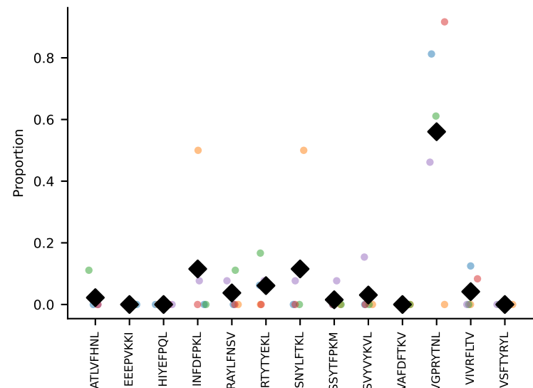
#435 AV8N-2-CATDGQGGRALIF-AJ15_BV13-1-CASSETGVSSYEYF-BJ2-7 coh=0.561, n=26
