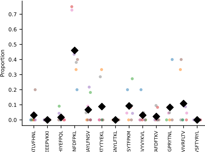
#370 AV14-2-CAASASSGSWQLIF-AJ22_BV31-CAWSLAGSGNTLYF-BJ coh=0.640, n=10
