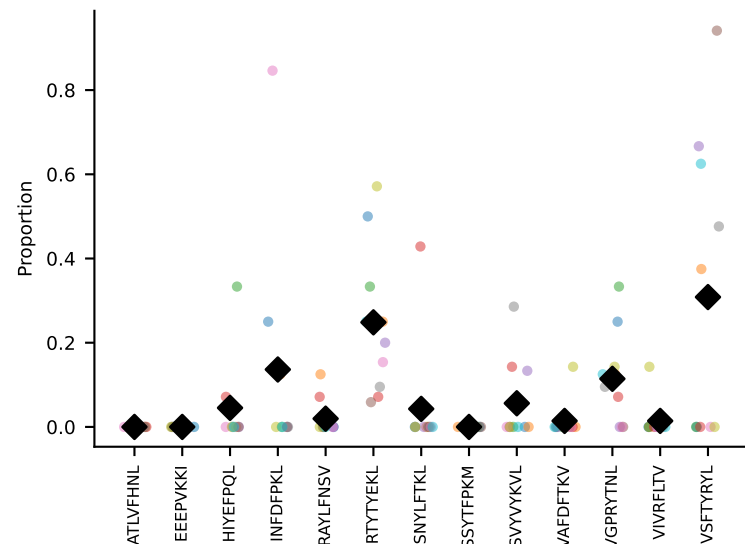
#247 AV4-4/DV10-CAAEATGGNNKLTf-AJ56_BV2-CASSQRPNTGQLYF-BJ2-2 coh=0.375, n=17
