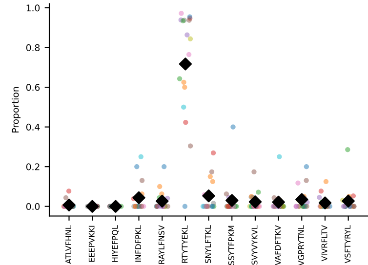
#349 AV7-2-CAASNMGYKLTF-AJ9_BV20-CGARLGGDYQYF-BJ2-5 coh=0.799, n=7
