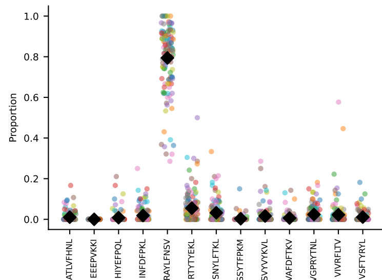
#165 AV8-1-CATDGASSFSKLVF-AJ50_BV1-CTCSADGVEQYF-BJ2-7 coh=0.935, n=9
