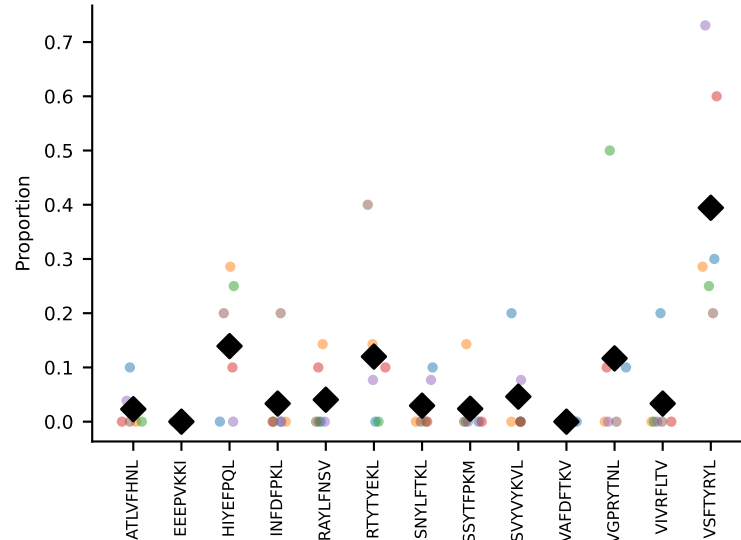
#436 AV4-4/DV10-CAAEANTGYQNIFY-AJ49_BV16-CASSWDRGNTQYF-BJ2-5 coh=0.541, n=14
