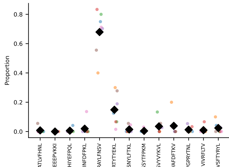
#176 AV12D-3-CALIASGSWQLIF-AJ22_BV13-2-CASGDAGNQAPLF-BJ1-5 coh=0.912, n=5
