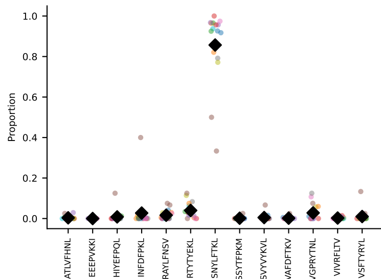
#284 AV16N-CAMRDDSGYNKLTF-AJ11_BV13-2-CASGDAGTGVDSDYTF-BJ1-4 coh=0.941, n=6
