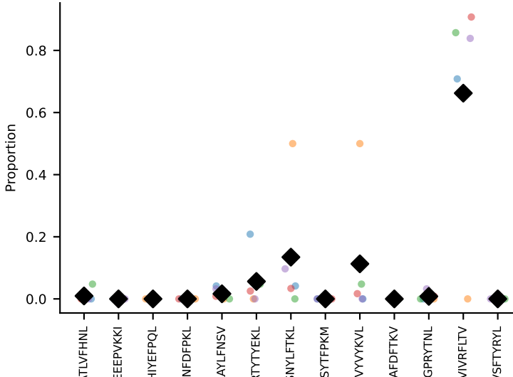
#231 AV13N-4-CAMEPSSFSKLVF-AJ50_BV31-CAWSLGGAEQFF-BJ2 coh=0.607, n=5
