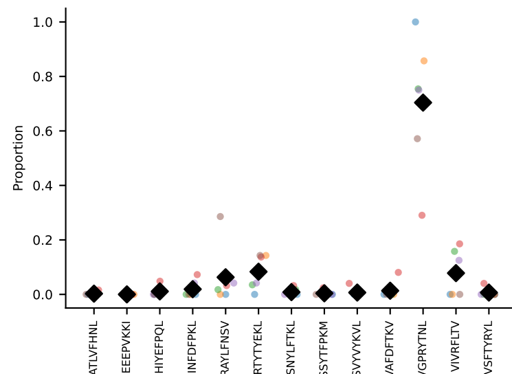
#315 AV6-7/DV9-CALSEDGTQNFYF-AJ49_BV17-CASSRDRGYTLF-BJ2-4 coh=0.889, n=6
