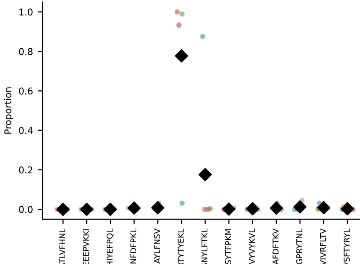
#230 AV16N-CAMRDDTNAYKVIF-AJ30_BV13-2-CASGDQGASGNTLYF-BJ] coh=0.614, n=5
