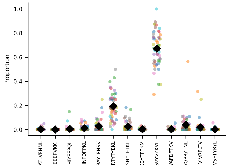
#302 AV14D-3/DV8-CAATGNTGKLIF-AJ37_BV19-CASSIVRVSEYEQYF-BJ2-7 coh=0.915, n=7
