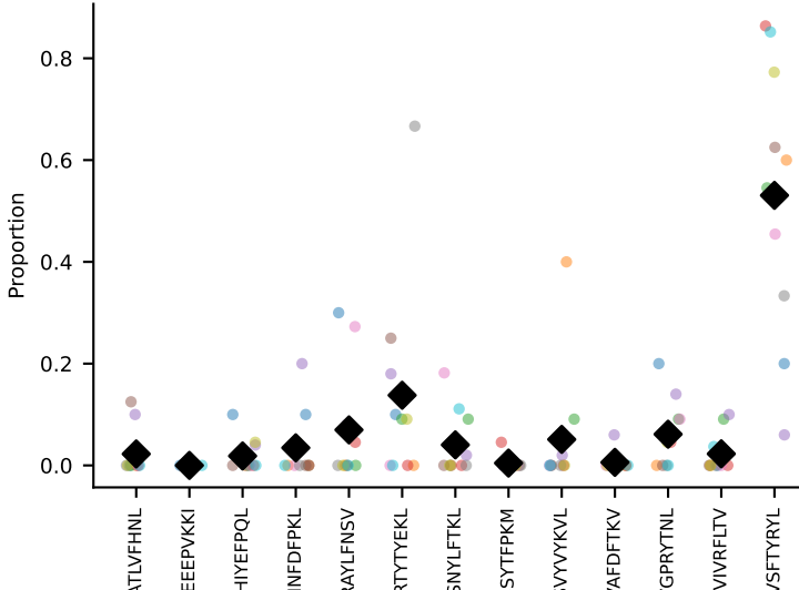
#229 AV9-4-CAVIDTEGADRLTF-AJ45_BV1-CTCSAVRVQNTLYF-BJ2-4 coh=0.629, n=17
