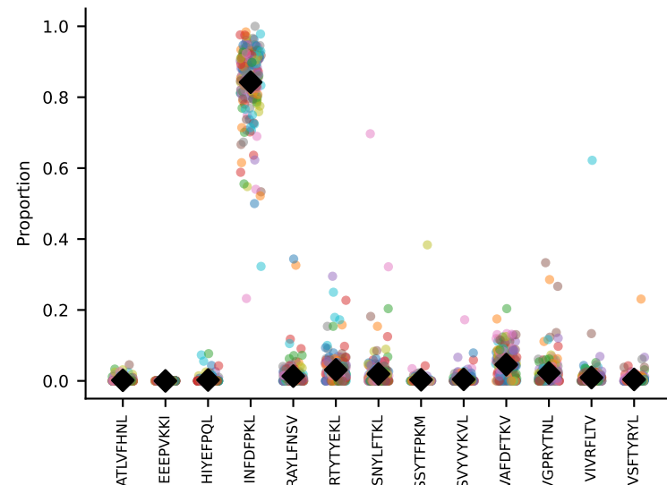
#264 AV13-2-CAIDQNAGAKLTF-AJ39_BV14-CASSLRGEQYF-BJ2-7 coh=0.968, n=197
