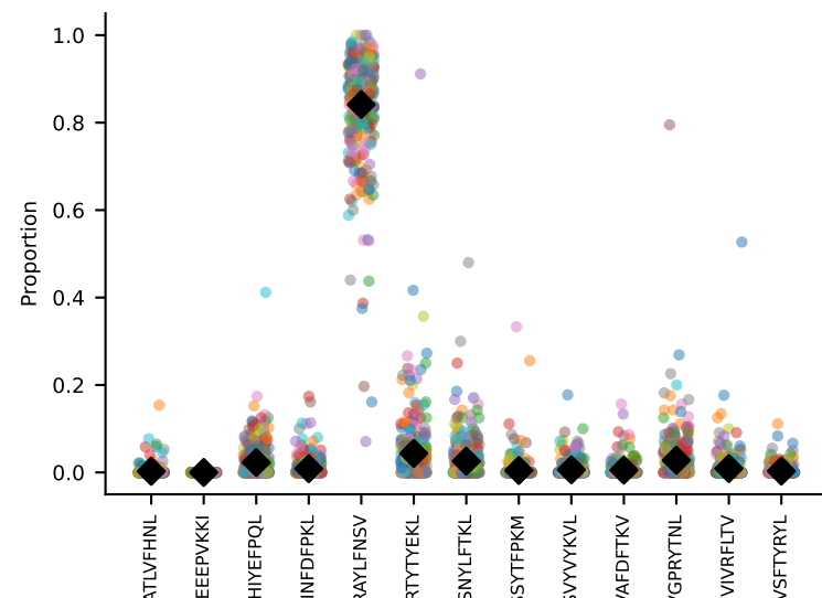
#123 AV16/DV11-CAMREPYQGGRALIF-AJ15_BV13-3-CASSERNQDTQYF-BJ2-7 coh=0.964, n=341
