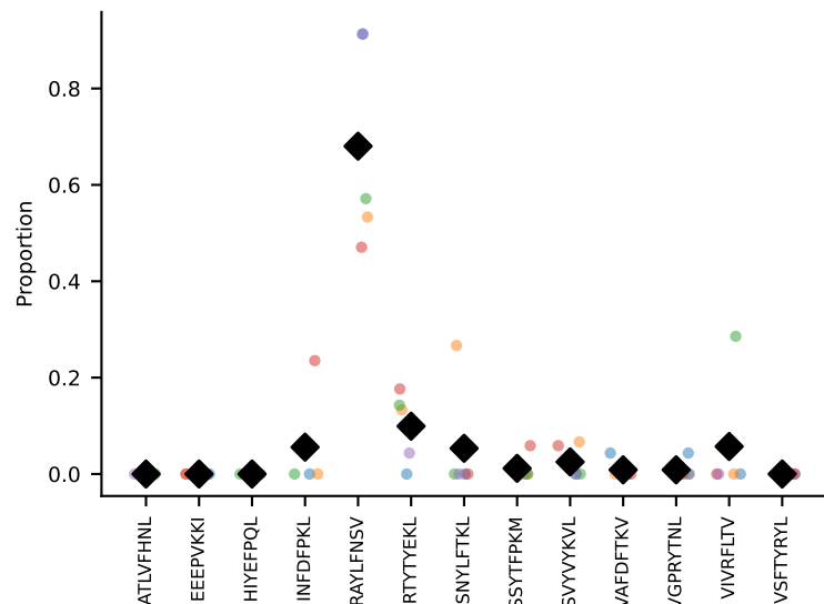
#328 AV16-CAMREANTGYQNFYF-AJ49_BV13-2-CASGEGAQNTLYF-BJ2-#329 AV16/DV11-CAMRESNTGYQNFYF-AJ49_BV13-2-CASGTGGANTLYF-BJ2-4 coh=0.857, n=18
