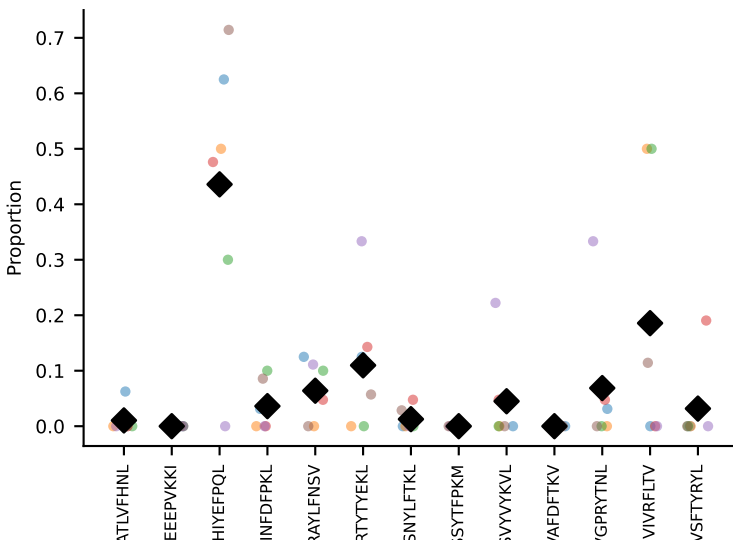
#238 AV13-3-CAMERSNNRIF-AJ31_BV2-CASSQDRRGDTQYF-BJ2-5 coh=0.530, n=6
