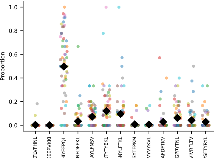
#372 AV13-1-CALERSNNRIFF-AJ31_BV2-CASSQDRRGDTQYF-BJ2- coh=0.619, n=64
