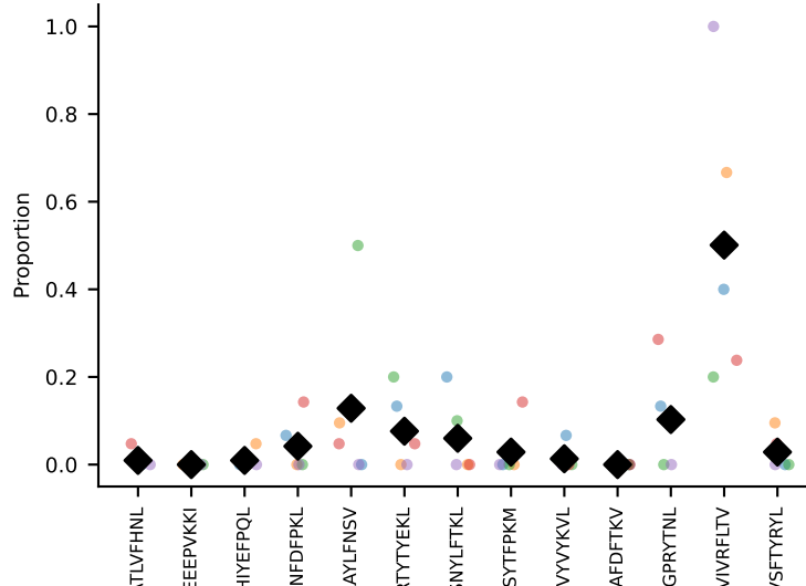
#232 AV7-2-CAASRGDYANKMIF-AJ47_BV13-3-CASSARVEQYF-BJ2- coh=0.605, n=5
