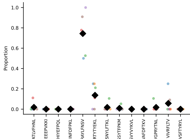
#173 AV9-4-CAVRTDYANKMIF-AJ47_BV3-CASSLSSEYEQYF-BJ2-7 coh=0.916, n=16
