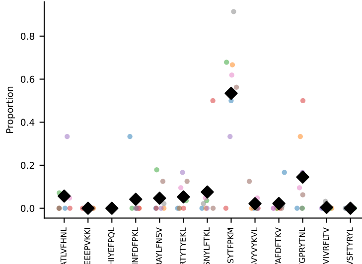
#371 AV14D-1-CAASEDSAGNKLTF-AJ17_BV20-CGARPDGTEVFF-BJ1 coh=0.623, n=5
