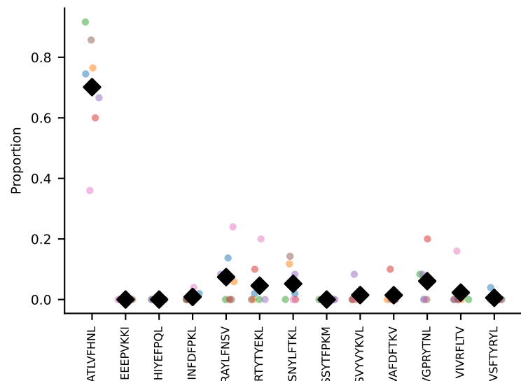
#314 AV10N-CAASMDYANKMIF-AJ47_BV3-CASSWTYNPLYF-BJ1-6 coh=0.890, n=24
