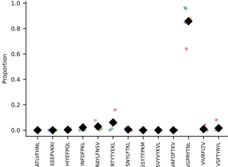
#390 AV9-2-CVLSSTSGGNYPKF-AJ6_BV1-CTCSAVRVDTEVFF-BJ1-1 coh=0.982, n=6
