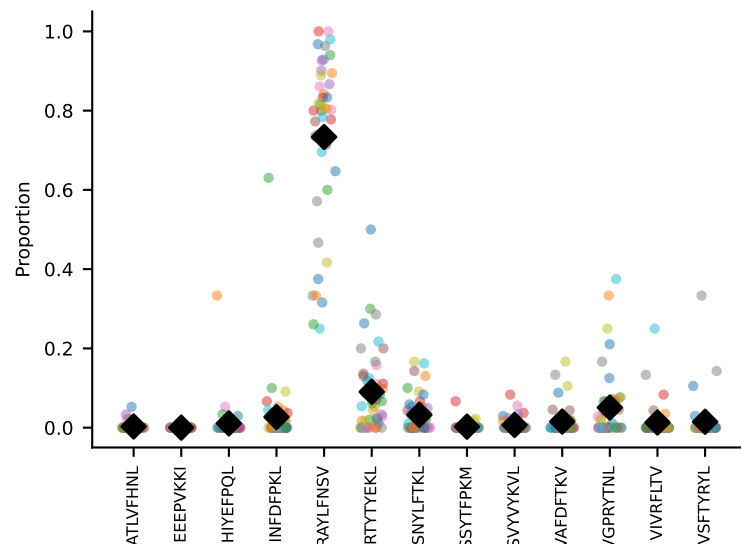
#325 AV13-1-CALVTGYQNFYF-AJ49_BV5-CASSQDRSQNTLYF-BJ2-4 coh=0.861, n=11
