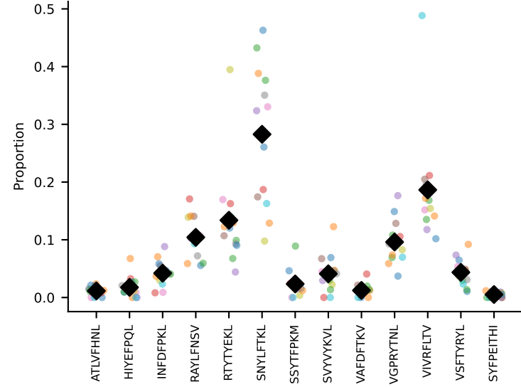
#189 AV12-2-CALNTGYQNIFY-AJ49_BV13-1-CASSDAGGYEQYF-BJ2-7 coh=0.828, n=13
