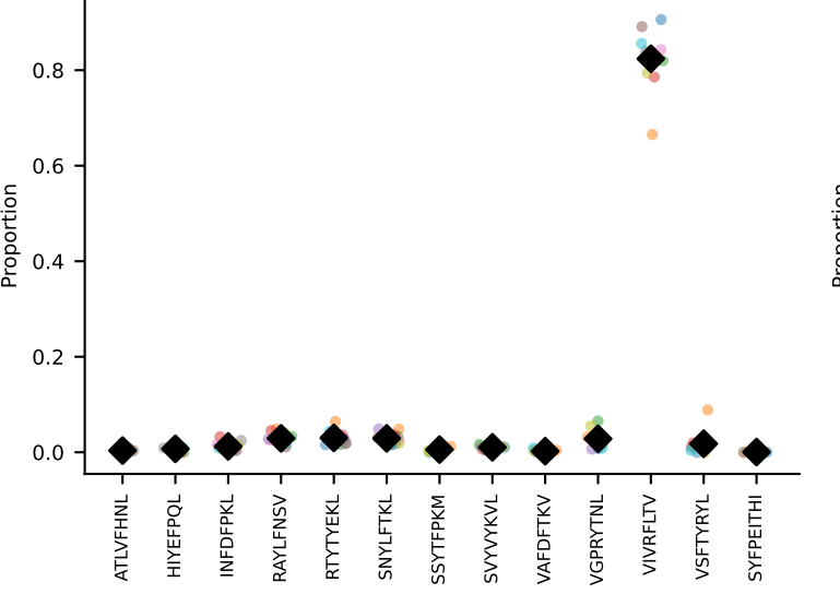
#19 AV12-1-CALSDPSNTDKVVF-AJ34*p03_BV13-1-CASSPHYNYAEQFF-BJ2-1 coh=0.996, n=10
