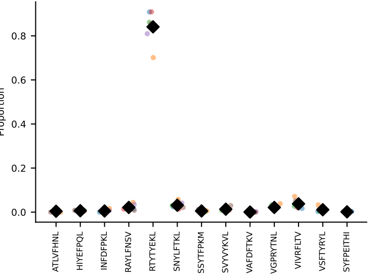
#17 AV13D-1-CAMELSSGSWQLIF-AJ22_BV4-CASSYGAQYF-BJ2-7 coh=0.997, n=6
