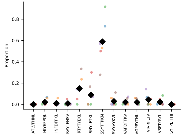
#188 AV4-3-CAADYQGGSAKLIF-AJ57_BV2-CASSQERLLGGAETLYF-BJ2-3 coh=0.833, n=7
