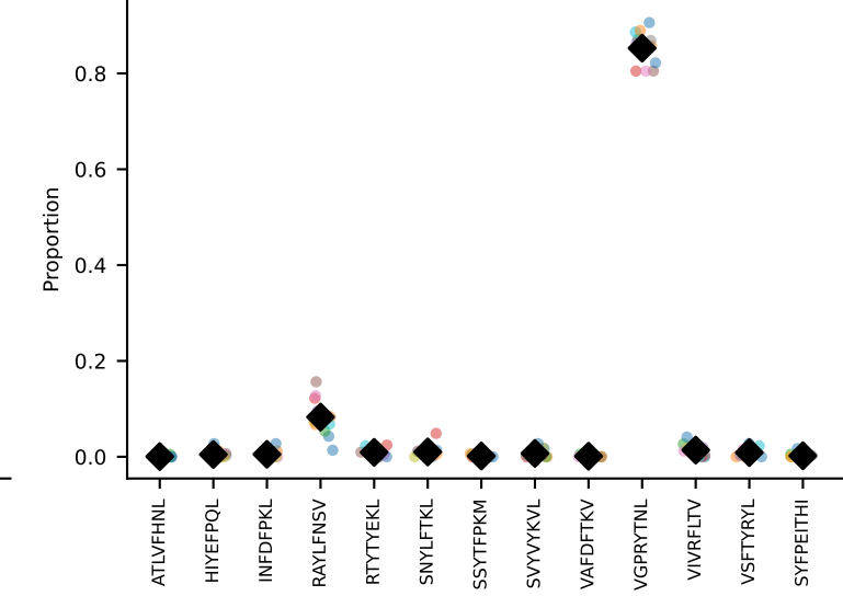
#22 AV9D-4-CALSPDTNAYKVIF-AJ30_BV12-1-CASSLWADTQYF-BJ2-5 coh=0.995, n=9
