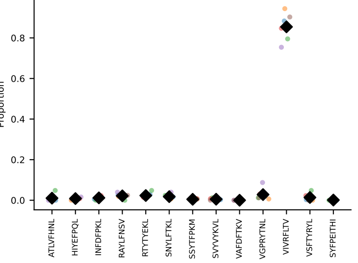
#20 AV4-3-CAAEANSAGNKLTF-AJ17*p02_BV13-3-CASSQLAEQFF-BJ2-1 coh=0.996, n=6
