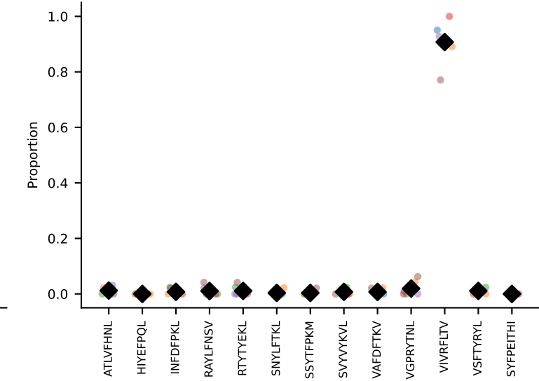
#95 AV16/DV11-CAMREDTGYNFYF-AJ49_BV13-1-CASGGVYEQYF-BJ2-5 coh=0.996, n=12
