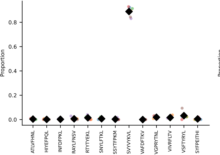
#94 AV7-3-CAVNAYKVIF-AJ30_BV13-2-CASGDLGGRDAETLYF-BJ2-3 coh=0.997, n=5
