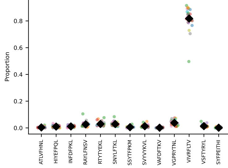
#21 AV16/DV11-CAMREDSSNTDKVVF-AJ34*p03_BV5-CASSQDLGGQNTLYF-BJ2-3 coh=0.995, n=28
