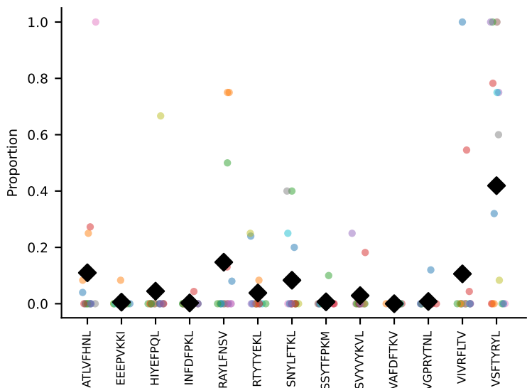
#70 AV6N-6-CALSATSSGQKLIV-AJ16_BV23-CSSSQSQTNTTEVFF-BJ1-1 coh=0.297, n=31
