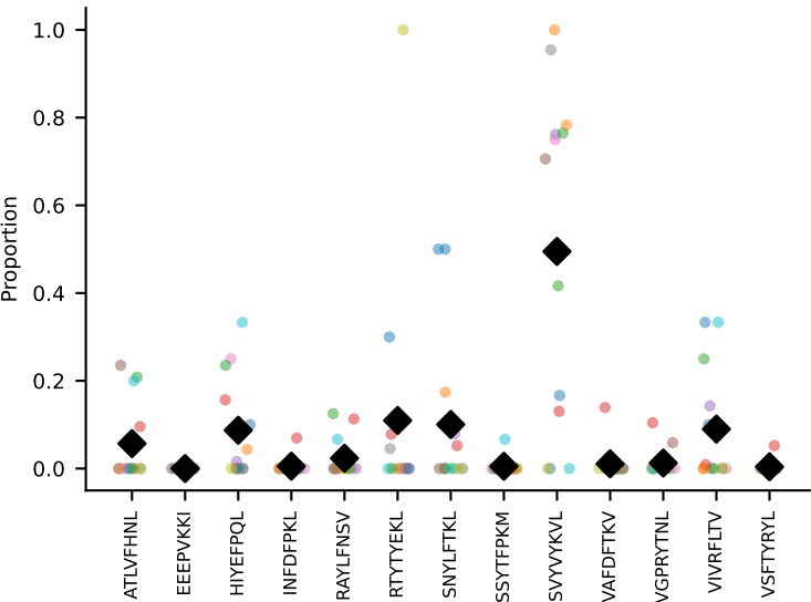
#236 AV9-4-CAVSAAGTGSNRLTF-AJ28_BV1-CTCSADWGVWAETLYF-BJ2-3 coh=0.455, n=6
