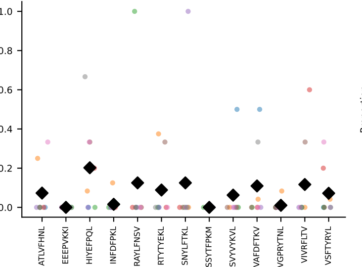
#157 AV16-CAMRETGYQNIFYF-AJ49_BV13-1-CASSDAYTEVFF-BJ1-1 coh=0.152, n=26
