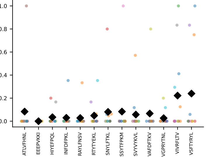
#365 AV13-2-CAIDPNTNKVVVF-AJ34_BV31-CAWSRLGVQNTLYF-BJ2-4 coh=0.146, n=7
