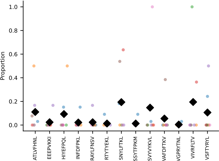
#363 AV8D-2-CATDSQGGRALIF-AJ15_BV3-CASSLHSSYEQYF-BJ2-7 coh=0.152, n=7
