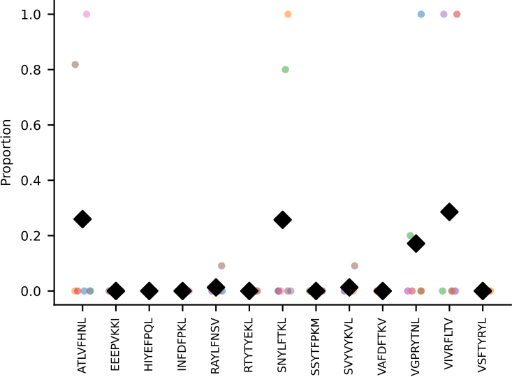
#213 AV8D-2-CATDAQGGRALIF-AJ15_BV19-CASSIGTSQNTLYF-BJ2-4 coh=0.149, n=8
