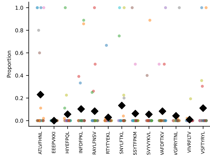
#382 AV8D-2-CATDNQGGRALIF-AJ15_BV13-1-CASSDLGVSYEQYF-BJ2-1 coh=0.116, n=10
