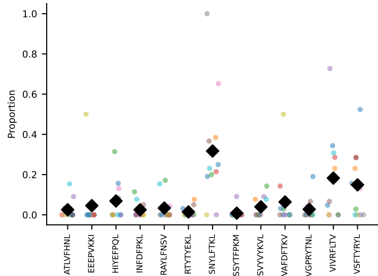
#32 AV14-2-CAASNSAGNKLTF-AJ17_BV3-CASSLGTGYEQYF-BJ2-7 coh=0.450, n=5
