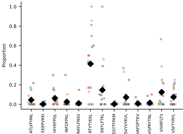
#237 AV7-1-CAVSDQGGRALIF-AJ15_BV19-CASSMRGVSDYTF-BJ1-2 coh=0.453, n=9
