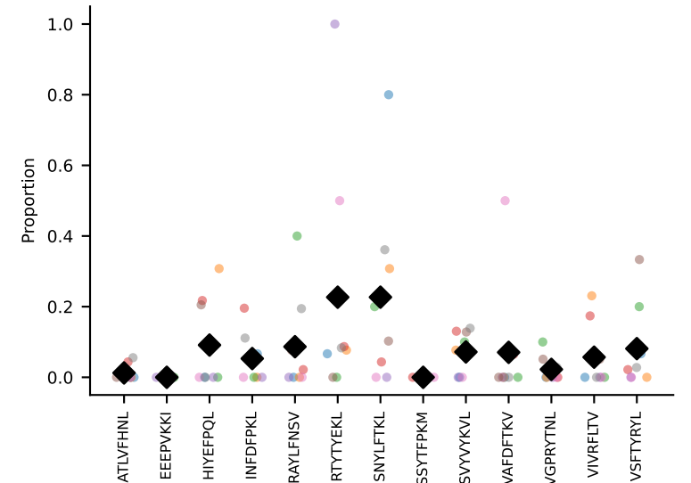
#270 AV10N-CAASPNNVLYF-AJ21_BV13-1-CASSDVGGQDTQYF-BJ2-5 coh=0.325, n=5
