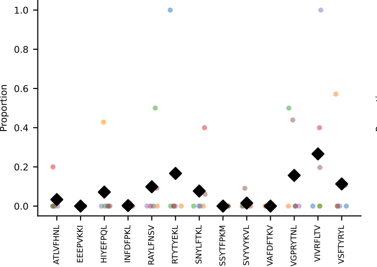
#158 AV6D-7-CALVLNTNTGKLTF-AJ27_BV31-CAWSLAGSGNTLYF-BJ1-3 coh=0.148, n=6
