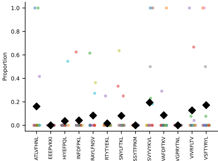
#380 AV16N-CAMREGTGGNNKLTF-AJ56_BV1-CTCRTGTDSYNPLYF-BJ1-6 coh=0.120, n=5
