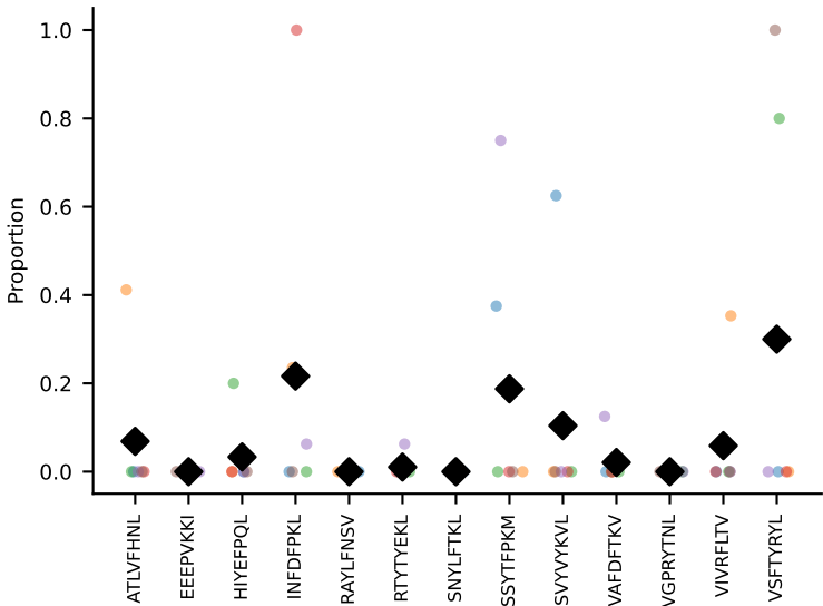
#379 AV3D-3-CALNMGYKLTF-AJ9_BV13-2-CASGARDWGGAQNTLYF-BJ2-4 #380 AV16N-CAMREGTGGNNKLTF-AJ56_BV1-CTCRTGTDSYNPLYF-BJ1-6 coh=0.121, n=5
