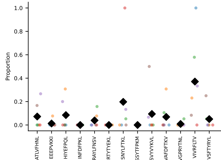
#268 AV9D-3-CAVSMQGGS AKLIF-AJ57_BV13-3-CASRDRGRD TQYF-BJ2-5 coh=0.328, n=5
