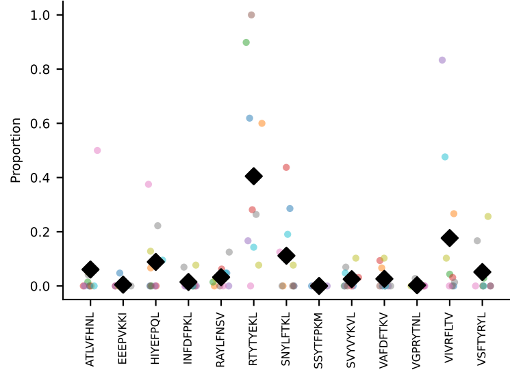
#33 AV16/DV11-CAMREGGGYKVVF-AJ12_BV13-2-CASGARTYNYAEQFF-BJ2-2 coh=0.441, n=10
