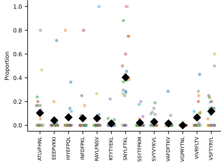
#176 AV6N-6-CARASSGSWQLIF-AJ22_BV13-1-CASSDAGTEVFF-BJ1-1 coh=0.443, n=23
