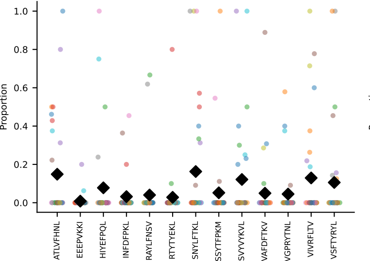
#211 AV7-4-CAAVITGNTGKLIF-AJ37_BV13-1-CASSGGNYAEQFF-BJ2-1 coh=0.152, n=6
