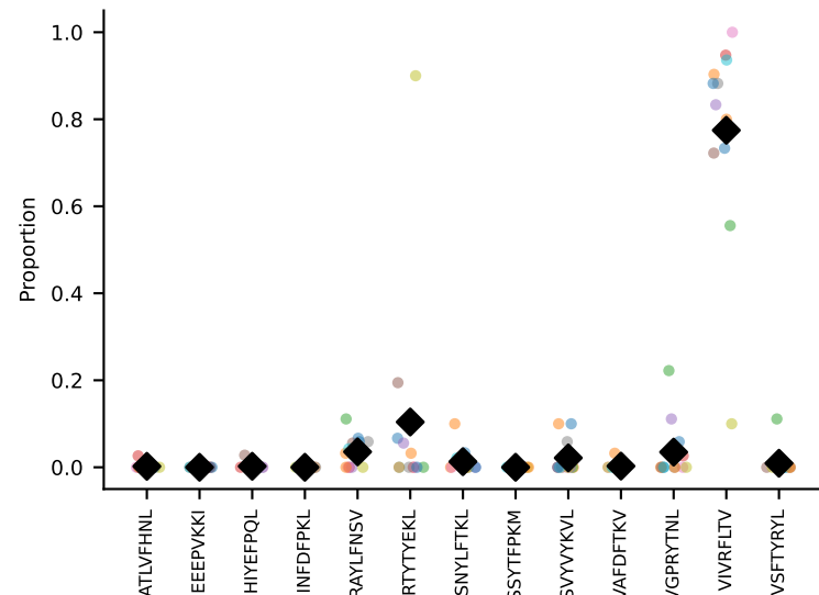
#126 AV16/DV11-CAMRDSGGSAKLTF-AJ42_BV1-CTCSADRVAETLYF-BJ2-3 coh=0.830, n=14
