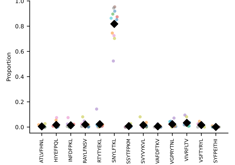
#8 AV7-3-CAVSIAGSWQLIF-AJ22_BV13-1-CASSDAGYEQYF-BJ2-7 coh=0.985, n=11
