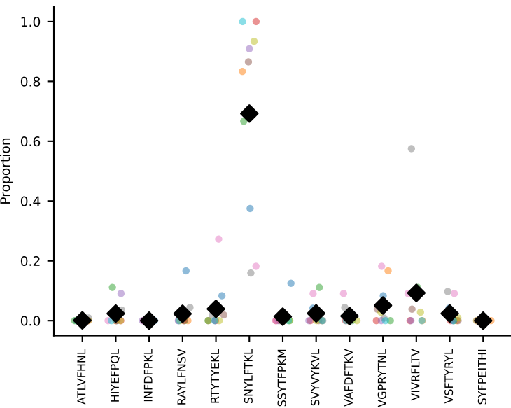
#16 AV7-3-CADDSGYNKLTF-AJ11*p02_BV13-2-CASGDVGGQNTLYF-BJ2-5 coh=0.739, n=10
