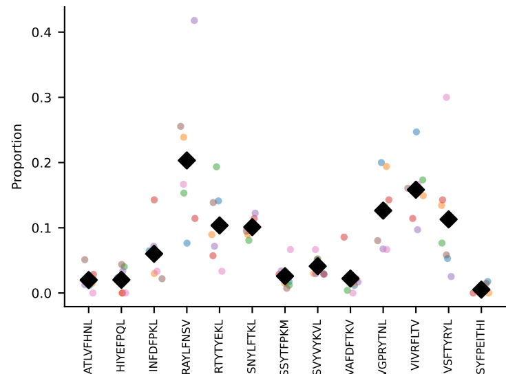
#96 AV6-6-CALGDDTGANTGKLTf-AJ52_BV13-2-CASGDWGGDTQYF-BJ2-1 coh=0.790, n=7
