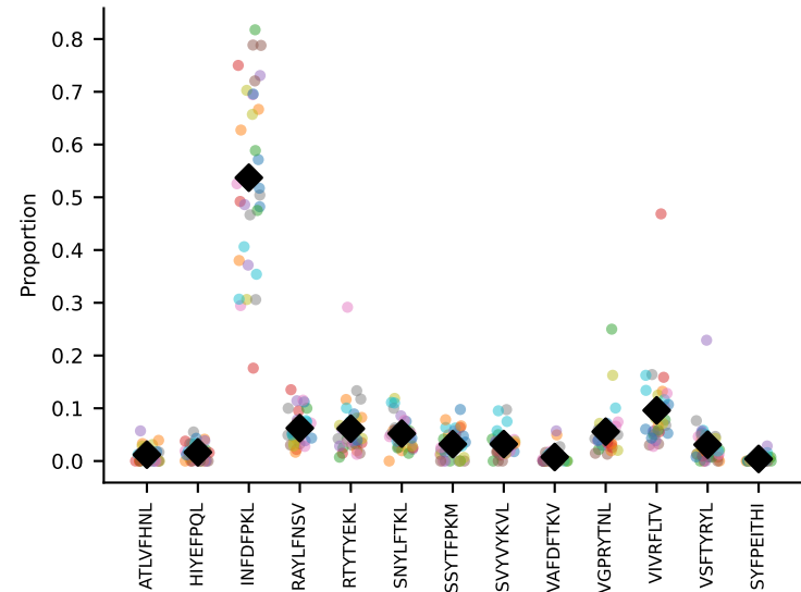
#65 AV16/DV11-CAMREGYQNIFY-AJ49_BV13-1-CASSGRNTEVFF-BJ1-1 coh=0.890, n=7
