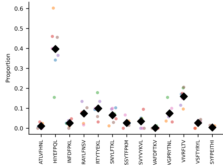
#69 AV5D-4-CAASEDSNYQLIW-AJ33_BV13-1-CASSDLGGQDTQYF-BJ2-5 coh=0.881, n=5
