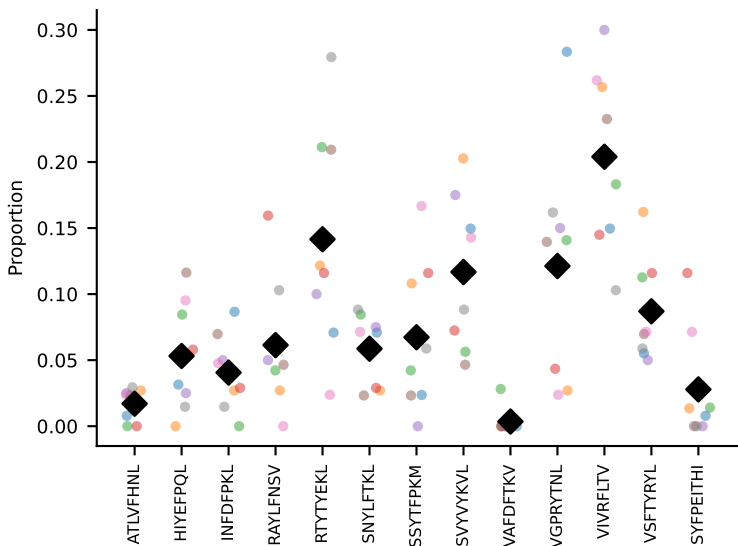
#108 AV16/DV11-CAMREDNNNAPRF-AJ43*p03_BV13-3-CASSDWGAETLYF-BJ2-2 coh=0.757, n=8
