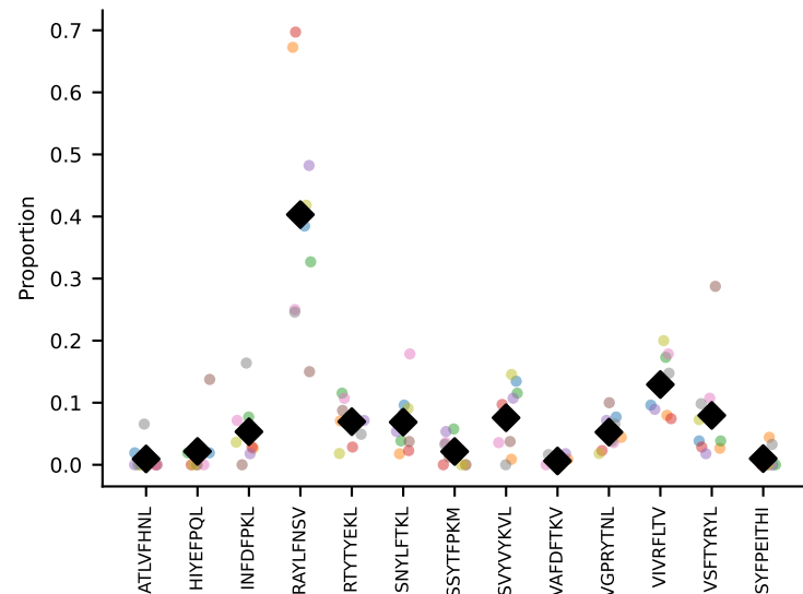
#92 AV8-1-CATDASSGSWQLIF-AJ22_BV4-CASTQANTEVFF-BJ1-1 coh=0.804, n=5
