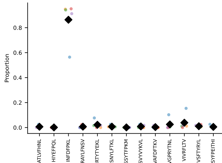
#31 AV7D-3-CAVIGSGSWQLIF-AJ22_BV13-2-CASGEPQGANSPLYF-BJ2-7 coh=0.972, n=26
