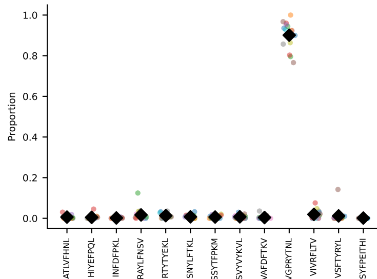
#19 AV16D/DV11-CAMREASSGSWLQIF-AJ22_BV13-2-CASGDPTGQEQYF-BJ2-7#20 AV9D-4-CALSANMGYKLTF-AJ9_BV13-1-CASSEGTGGIYEQYF-BJ2-7 coh=0.992, n=44
