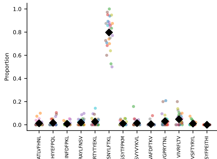
#35 AV9D-4-CALSATNAVKVIF-AJ30_BV13-2-CASGDAAGKDTQYF-BJ2-5 coh=0.960, n=7
