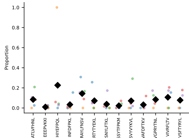
#16 AV13D-2-CAIDYNQGKLIF-AJ23_BV1-CTCSAVRISGNTLYF-BJ1-3 coh=0.355, n=5
