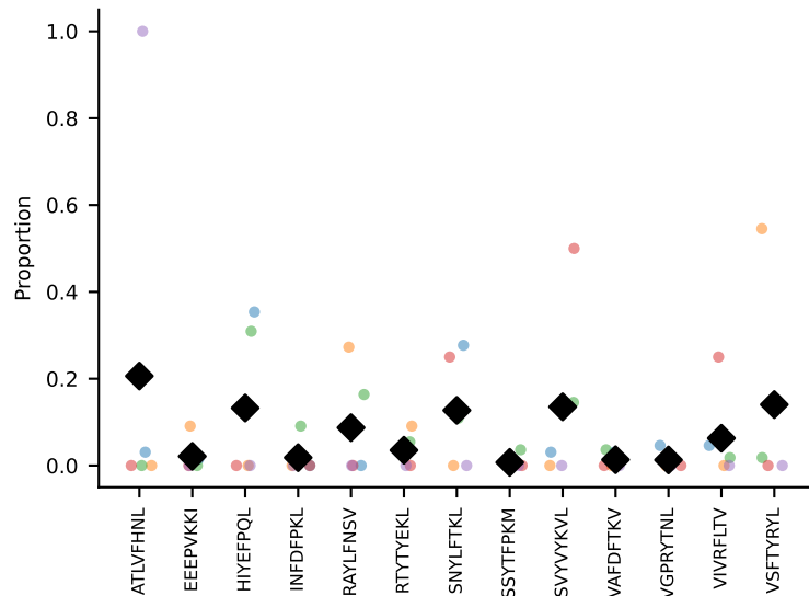
#59 AV13-2-CAMNTGNYKYVF-AJ40_BV5-CASSRQQDTQYF-BJ2-5 coh=0.147, n=7
