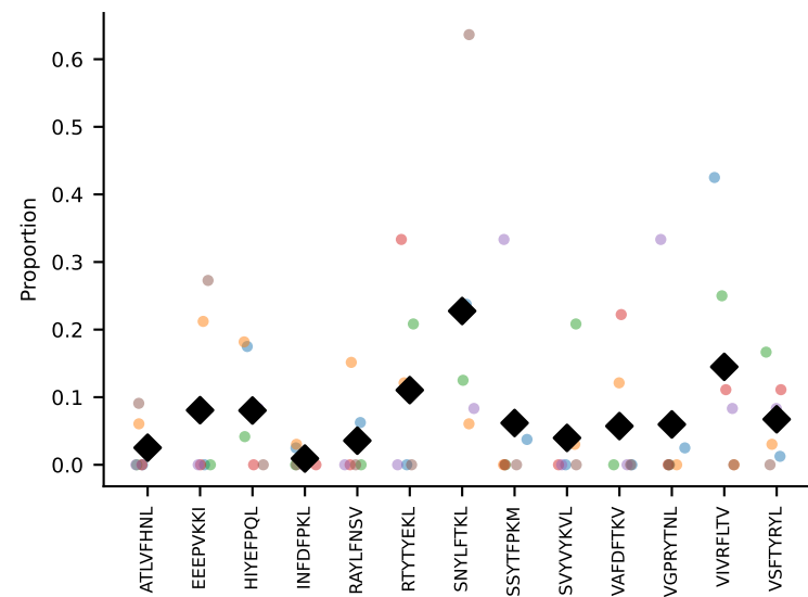
#33 AV14-2-CAASASSGSWQLIF-AJ22_BV31-CAWSLSGSGNTLYF-BJ1-3 coh=0.350, n=6
