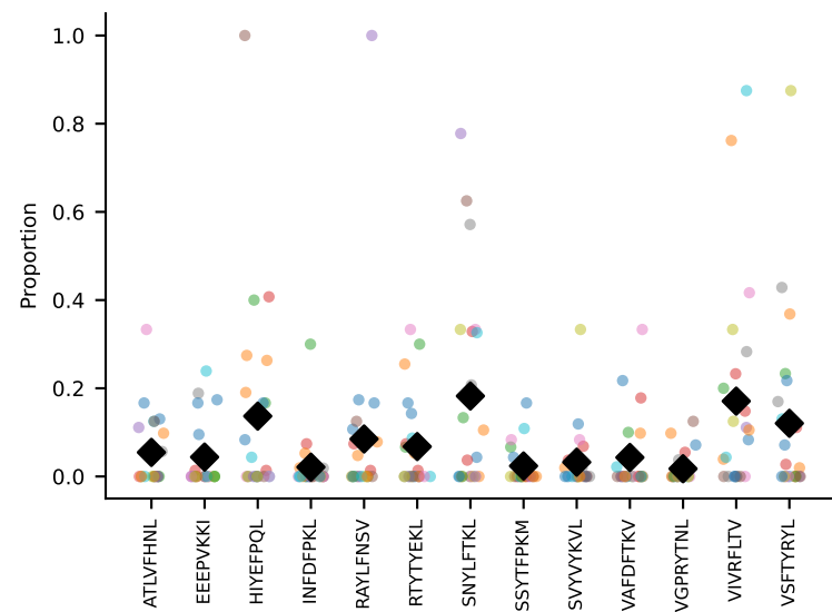
#36 AV7-5-CAVGGS GGKLTf-AJ44_BV4-CASSLGRHTEVFF-BJ1-1 coh=0.333, n=22
