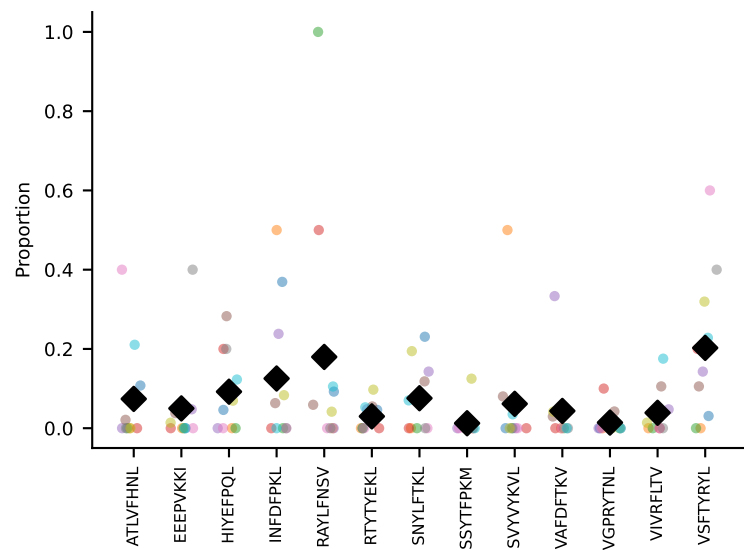
#35 AV6-6-CALGEDYSNNRLTL-AJ7_BV26-CASSHGGRNTLYF-BJ2-4 coh=0.335, n=10
