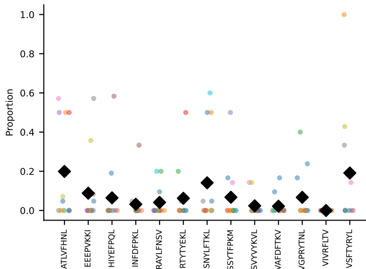
#54 AV7D-3-CAVQGGRALIF-AJ15_BV1-CTCSADQNSGNTLYF-BJ1-3 coh=0.211, n=10
