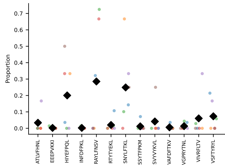
#32 AV14D-3/DV8-CAASASSGYNKLTf-AJ11_BV3-CASSLEGGAHEQYF-BJ1-1 coh=0.351, n=11
