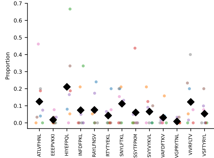
#29 AV3D-3-CAVSEGNTGKLIF-AJ37_BV1-CTCSADAVGSDYTF-BJ1-2 coh=0.376, n=5
