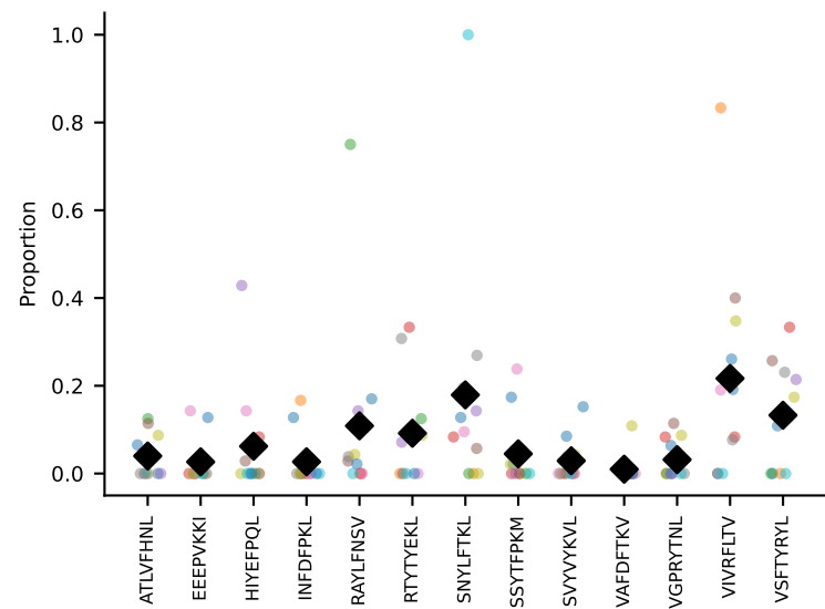
#30 AV14-2-CAASASSGSWQLIF-AJ22_BV31-CAWSLQSGSGNTLYF-BJ1-3 coh=0.355, n=6
