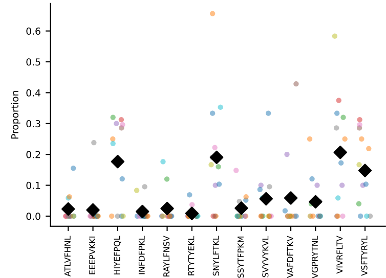
#21 AV6D-5-CALGDSGYNKLTf-AJ11_BV31-CAWSLRLGQDTQYF-BJ2-5 coh=0.431, n=5
