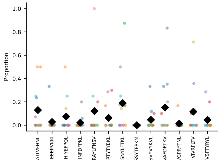
#55 AV16N-CAMREGDQGGRALIF-AJ15_BV13-1-CASSESRGPNERLFF-BJ1-4 coh=0.207, n=5
