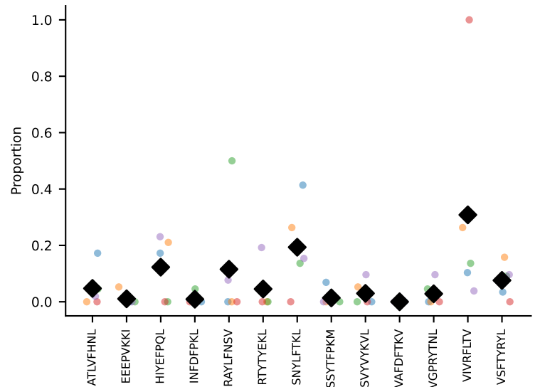
#23 AV6-6-CALGDYANKMIF-AJ47_BV13-1-CASSDADSNNQAPLF-BJ1-5 coh=0.420, n=5
