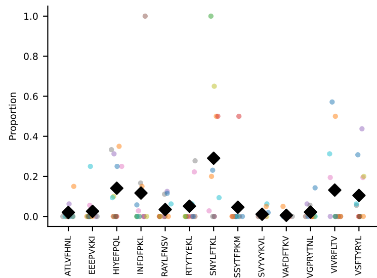
#34 AV13D-1-CAMERSNNRIFF-AJ31_BV2-CASSQDRRGDTQYF-BJ2-5 coh=0.346, n=12
