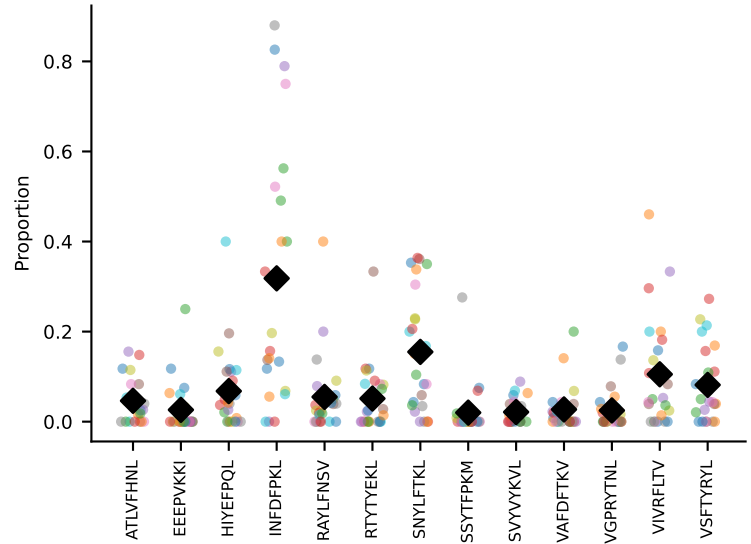
#18 AV7-1-CAVSDQGGRALIF-AJ15_BV19-CASSMRGVSDYTF-BJ1-2 coh=0.473, n=5
