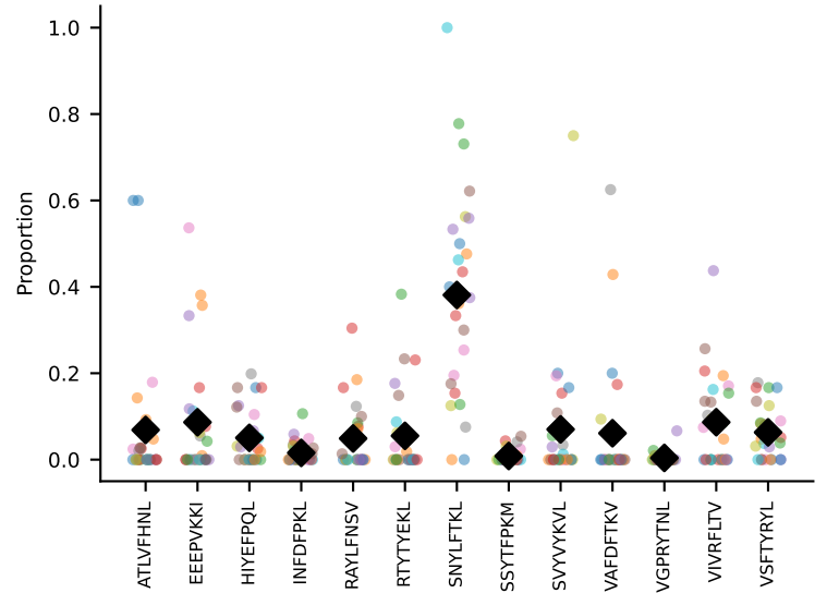
#19 AV8D-2-CATDNQGGRALIF-AJ15_BV5-CASSPGTGSERLFF-BJ1-4 coh=0.472, n=6
