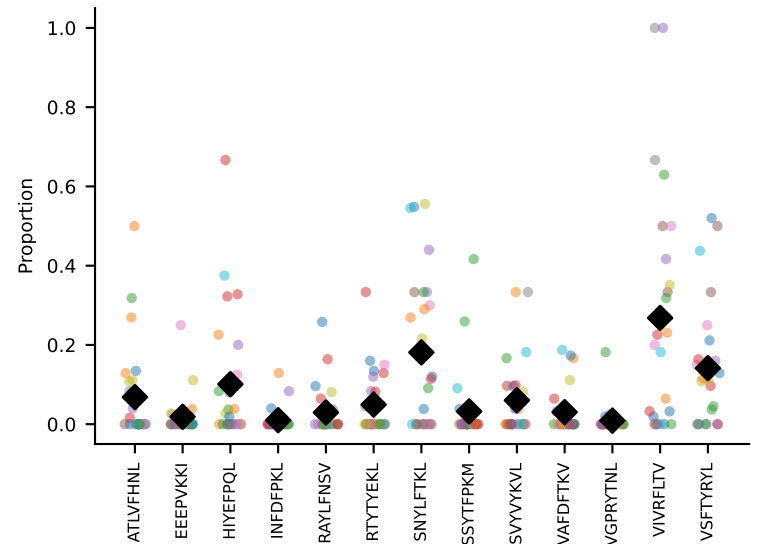
#24 AV14-2-CAASASSGSWQLIF-AJ22_BV31-CAWSLAGSGNTLYF-BJ1-3 coh=0.410, n=25
