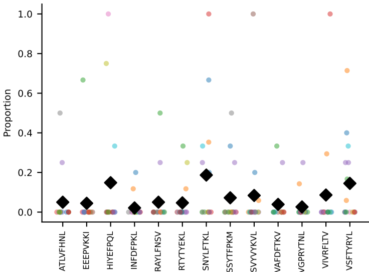
#57 AV12D-3-CALTNYNVLYF-AJ21_BV19-CASSITGDNSPLYF-BJ1-6 coh=0.175, n=15
