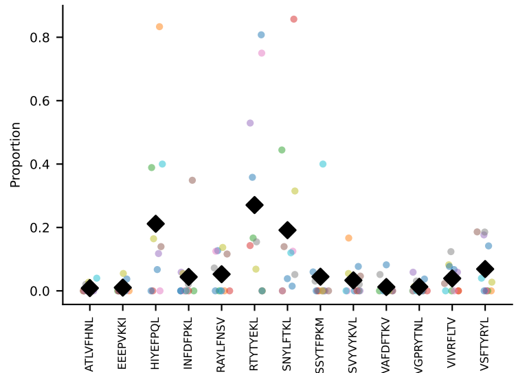
#22 AV8N-2-CAPGTGGYKVVF-AJ12_BV13-1-CASSEGTYQNTLYF-BJ2-4 coh=0.421, n=11
