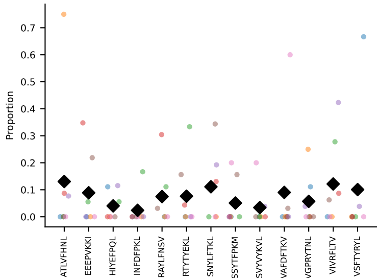
#58 AV19-CATNQGGSAKLIF-AJ57_BV5-CASSQQGNYAEQFF-BJ2-1 coh=0.173, n=7
