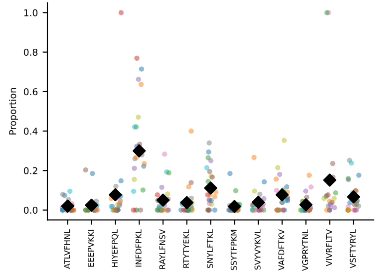
#20 AV13-2-CALEGRGSNYKLTf-AJ53_BV14-CASSSRYEQYF-BJ2-7 coh=0.455, n=5
