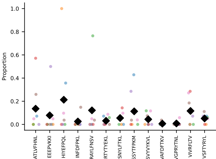
#53 AV14D-1-CAASASNYNVLYF-AJ21_BV5-CASSRDWDEYQF-BJ2-7 coh=0.213, n=7
