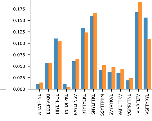
AV13-2-CAIDPNTGKLTf-AJ27_BV13-3-CASSDVNSDYTF-BJ1-2 PROP n:13→0 LOST
