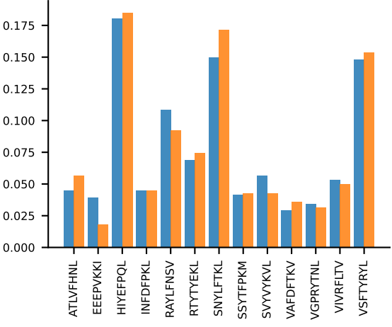
AV12-3-CALSDNYNQGLKIF-AJ23_BV2-CASSQAVSYEQYF-BJ2-7 PROP n:17→8
