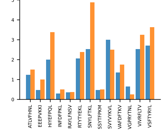
AV16-CAMREANTGYQNIFY-AJ49_BV13-2-CASGDGAQNTLYF-BJ2-4 MEAN n:14→0 LOST
