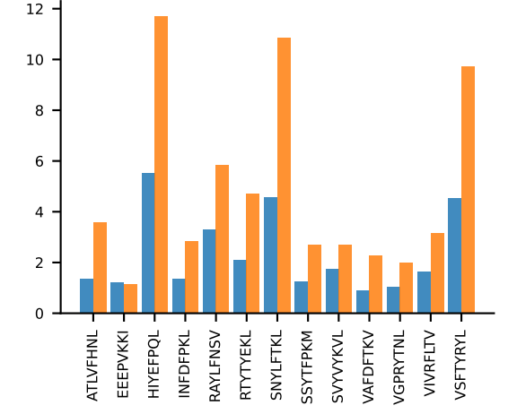
AV12-3-CALSDNYNQGLKIF-AJ23_BV2-CASSQAVSYEQYF-BJ2-7 MEAN n:17→8
