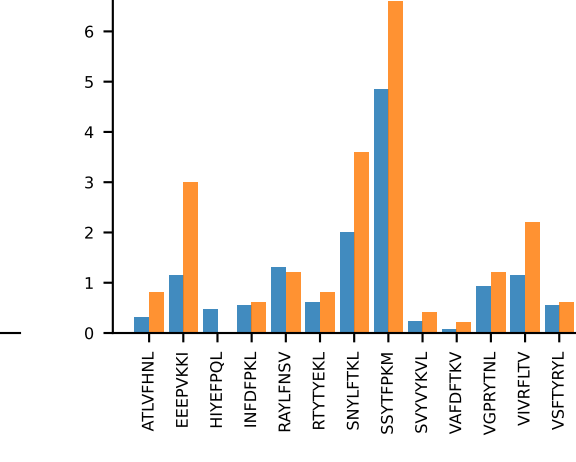
AV19-CAAGAAGYQNIFY-AJ49_BV17-CASSRRTGANTGQLYF-BJ2-2 MEAN n:13→5
