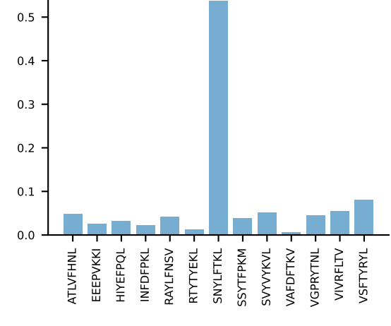
AV16-CAMREANTGYQNIFY-AJ49_BV13-2-CASGDGAQNTLYF-BJ2-4 PROP n:14→0 LOST
