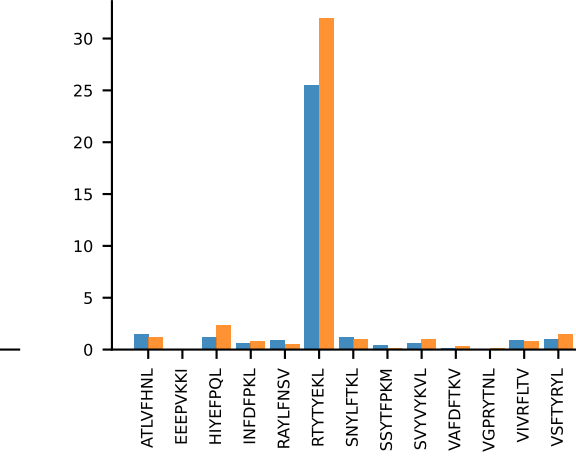
AV14-1-CAASADTGNKYKVF-AJ40_BV13-3-CASSDSNTEVFF-BJ1-1 MEAN n:14→0 LOST
