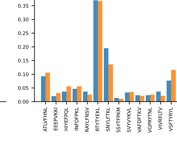
AV16N-CAMREGNSNNRIFF-AJ31_BV13-1-CASRDINTEVFF-BJ1-1 PROP n:13→6
