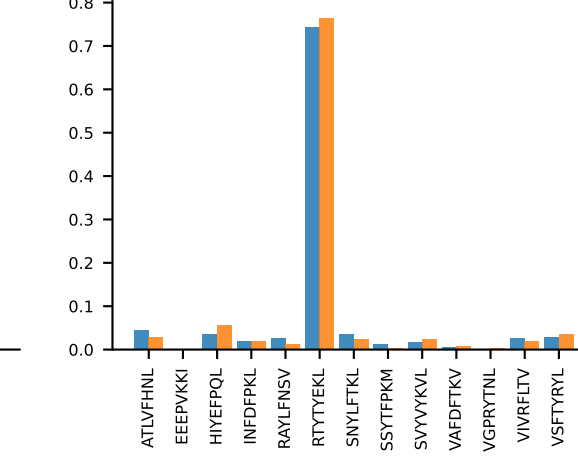
AV14-1-CAASADTGNKYKVF-AJ40_BV13-3-CASSDSNTEVFF-BJ1-1 PROP n:14→0 LOST
