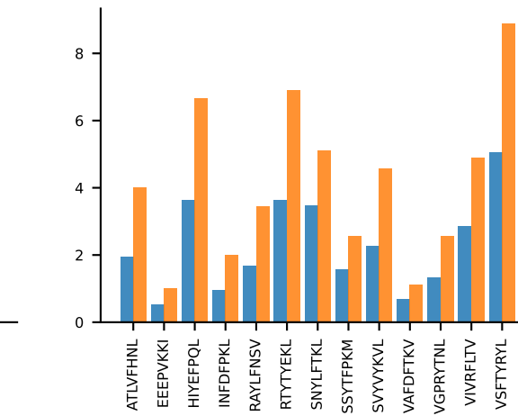
AV16-CAMREDTGYNFYF-AJ49_BV13-2-CASGDRGRNEQYF-BJ2-4 MEAN n:17→6
