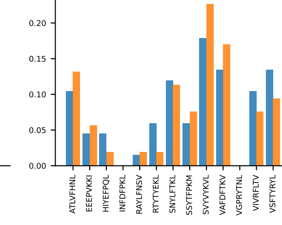
AV19-CAAGAAGYQNIFY-AJ49_BV17-CASSRRTGANTGQLYF-BJ2-2 PROP n:13→5
