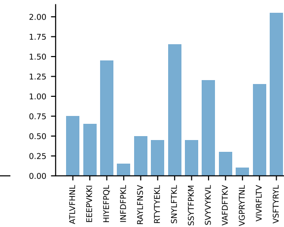
AV6-6-CALGESGGSNAKLTf-AJ42_BV13-3-CASSDAQTNSPLYF-BJ1-6 MEAN n:19→6
