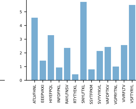
AV16N-CAMREGNSNNRIFF-AJ31_BV13-1-CASRDINTEVFF-BJ1-1 MEAN n:13→6
