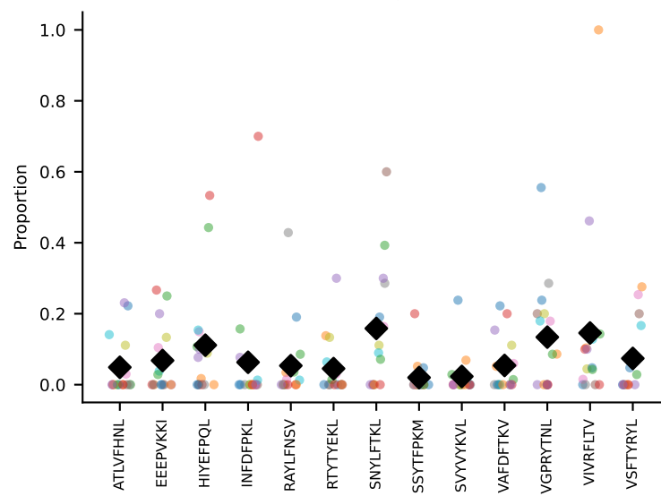
#43 AV12-2-CALRGTYGNYKYVF-AJ40_BV1-CTCSASRDPYNSPLYF-BJ1-6 coh=0.329, n=6
