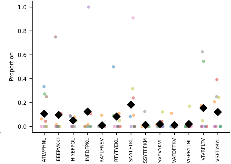
#80 AV16N-CAMREETGNTGKLIF-AJ37_BV1-CTCSANRVDTQYF-BJ2-5 coh=0.221, n=5
