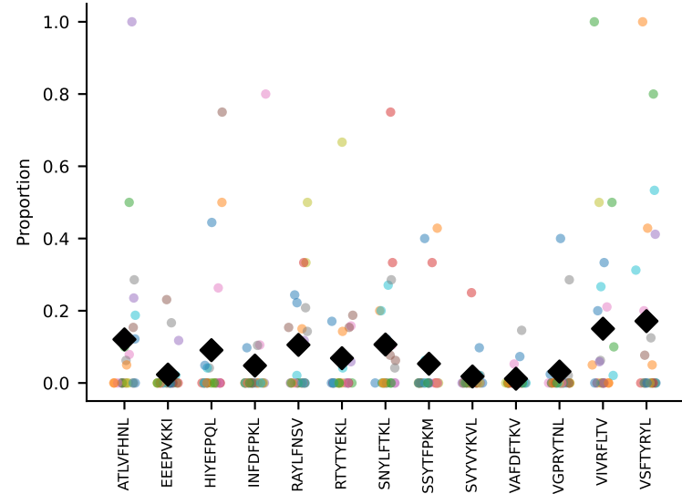
#72 AV16-CAMGTGSGGKLTf-AJ44_BV1-CTCSTRGANERLFF-BJ1-4 coh=0.255, n=23
