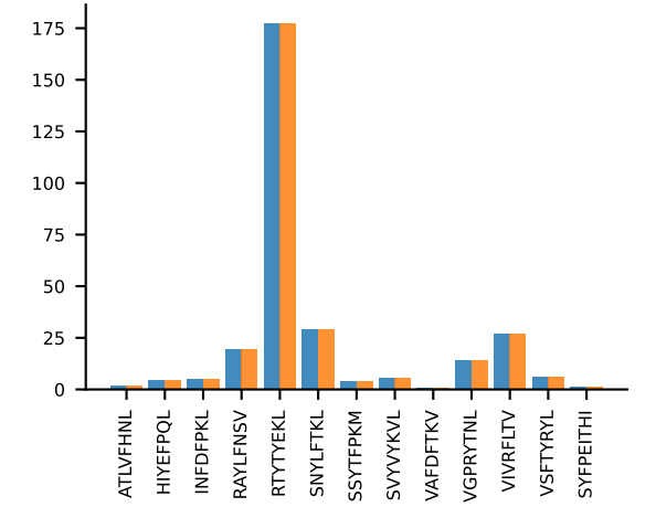
AV16/DV11-CAMRENTGANTGKLTf-AJ52_BV13-3-CASSSGGVKAEQFF-BJ2-4 MEAN n:15→15
