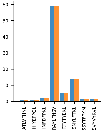
AV16D/DV11-CAMREDNNRIFF-AJ31_BV13-2-CASGEIATNTGQLYF-BJ2-7 PROP n:15→15
