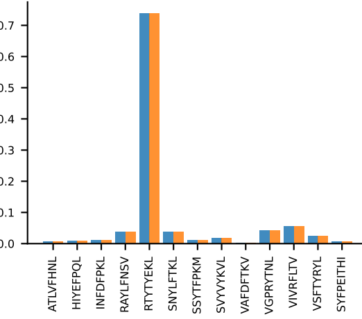
AV16/DV11-CAMRENTGANTGKLTf-AJ52_BV13-3-CASSSGGVKAEQFF-BJ2-4 PROP n:15→15
