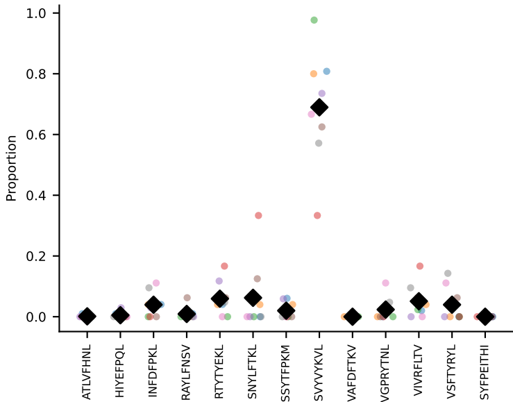
#18 AV7D-2-CAANTNTGKLTf-AJ27_BV1-CTCSADRVNNQAPLF-BJ1-5 coh=0.651, n=5
