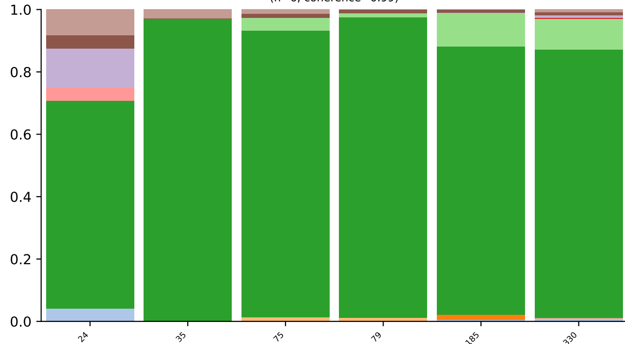
Dual AV16D/DV11-CAMREGNTGNYKYVF-AJ40/AV6-3-CAPPGGADRLTF-AJ45_BV13-2-CASGDLYEQYF-BJ2-7 (n=6, coherence=0.99)
