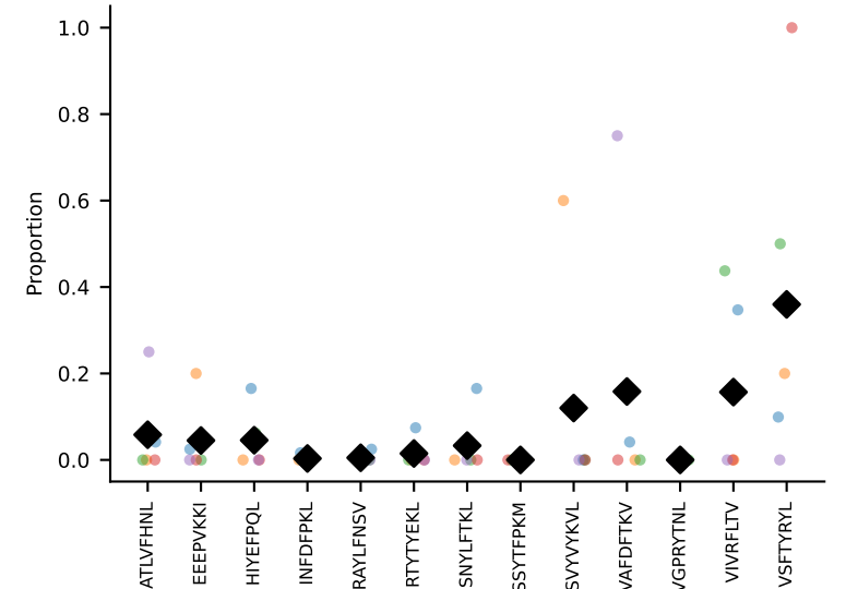
#44 AV14-2-CAASPYTGNYKYVF-AJ40_BV13-2-CASTNNNQAPLF-BJ1-5 coh=0.236, n=13
