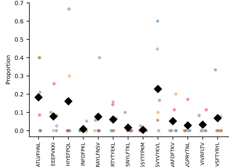
#29 AV9-2-CVLSTVGSGGKLTAL-AJ44_BV14-CASSFANTGQLYF-BJ2-2 coh=0.296, n=22
