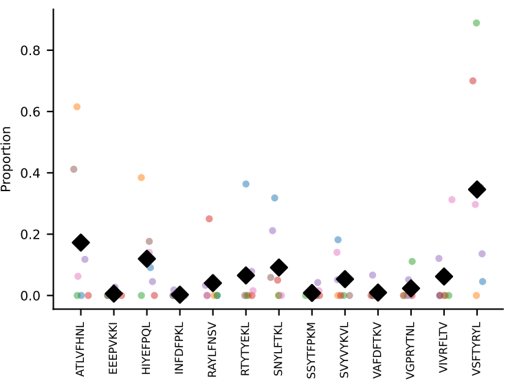
#17 AV16N-CAMREVYQGGRALIF-AJ15_BV16-CASSFVGNQDTQYF-BJ2-5 coh=0.349, n=6
