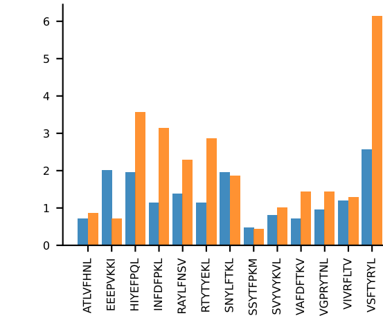
AV8N-2-CATENYGSSGNKLIF-AJ32_BV3-CASSLGREYTOYF-BJ2-5 MEAN n:19→5
