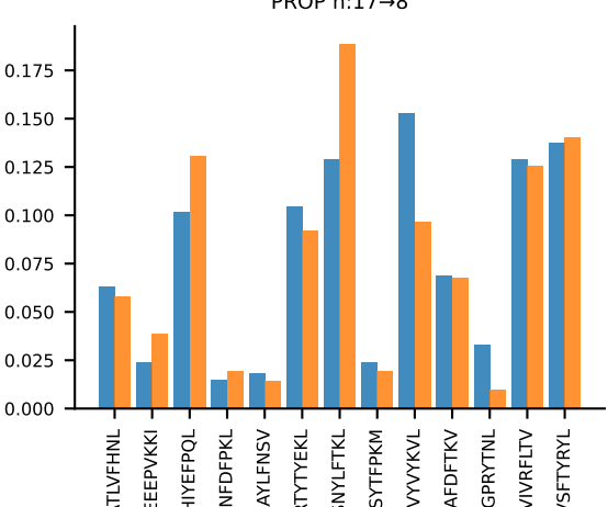
AV12-3-CALSDNYNQGLIF-AJ23_BV2-CASSQAVSYEQYF-BJ2-7 PROP n:17→8
