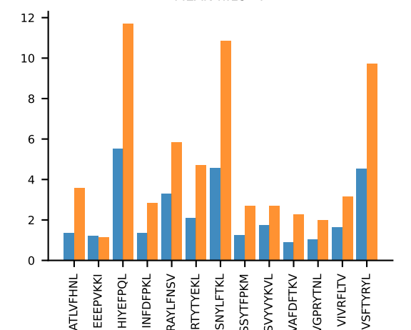
AV12-3-CALSDNYNQGLIF-AJ23_BV2-CASSQAVSYEQYF-BJ2-7 MEAN n:17→8
