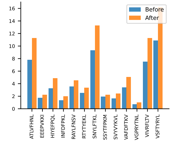
AV7N-4-CAVSEDGRGSALGRLHF-AJ18_BV1-CTCSAGGDYAEQFF-BJ2-4 MEAN n:19→7
