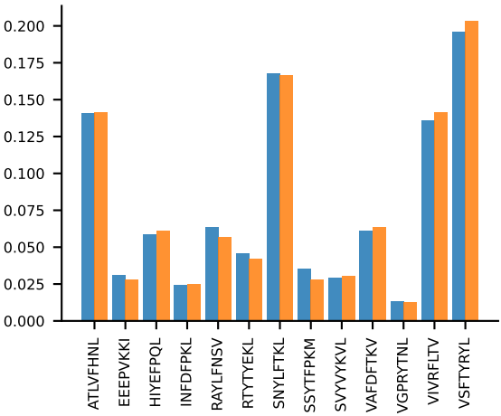
AV7N-4-CAVSEDGRGSALGRLHF-AJ18_BV1-CTCSAGGDYAEQFF-BJ2-4 PROP n:19→7
