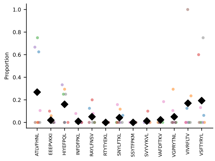
#65 AV7-2-CAASMRGSA LGR LHF-AJ18_BV14-CASSFRQGAVTGQLYF-BJ2-2 coh=0.276, n=6
