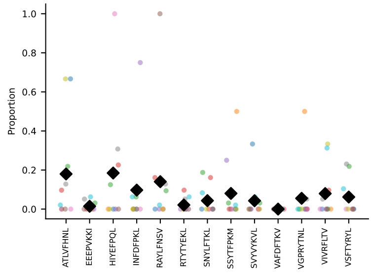
#69 AV14-2-CAASGTGYQNIFY-AJ49_BV2-CASSQAWGNQDTQYF-BJ2-5 coh=0.256, n=10
