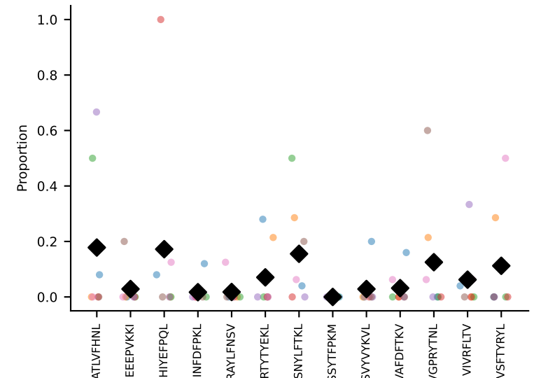
#84 AV14-2-CAASAASGSWQLIF-AJ22_BV31-CAWSLAGSGNTLYF-BJ1-3 coh=0.191, n=7
