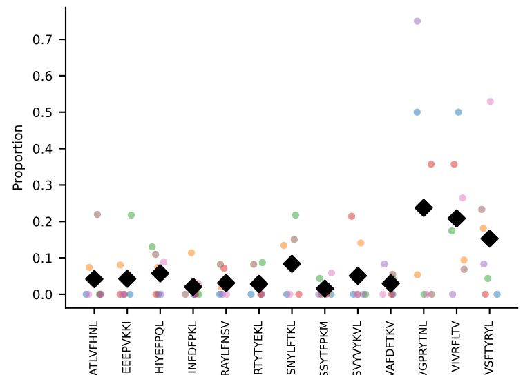
J1-1#24 AV9-2-CVFHDTNAYKVIF-AJ30_BV13-2-CASGDALFQDTQYF-BJ2-5 coh=0.400, n=10
