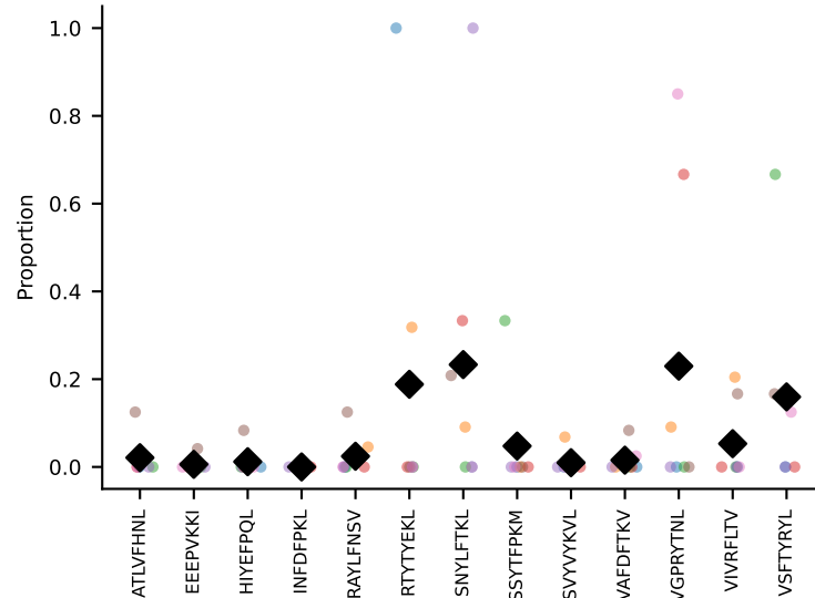
#75 AV14-3-CAASAAAYANKMIF-AJ47_BV3-CASSLGPA NTGQLYF-BJ2-2 coh=0.240, n=7
