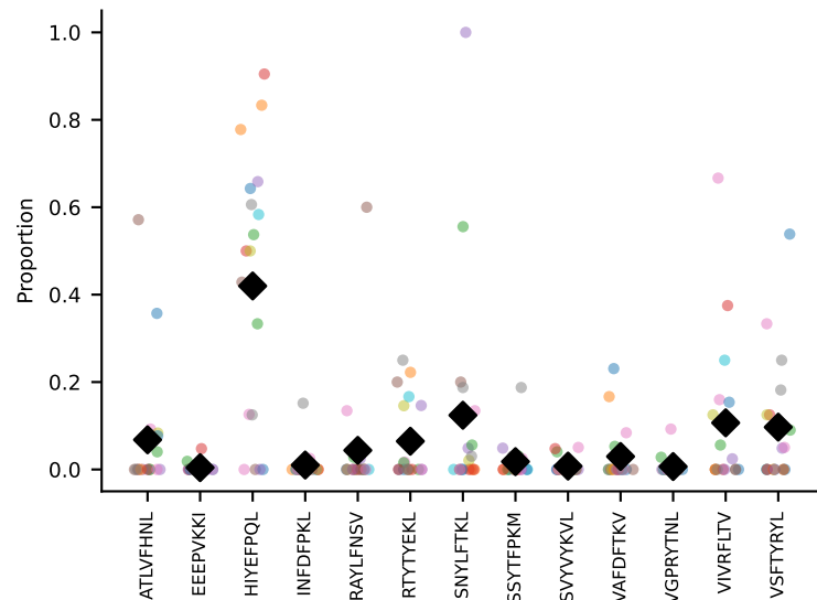
#19 AV12-3-CALSDNYNQGLIF-AJ23_BV2-CASSQAVSYEQYF-BJ2-7 coh=0.428, n=10
