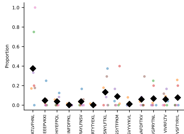
#22 AV7-4-CAASSDTNAYKVIF-AJ30_BV2-CASSQRTGVNTLYF-BJ2-4 coh=0.404, n=6
