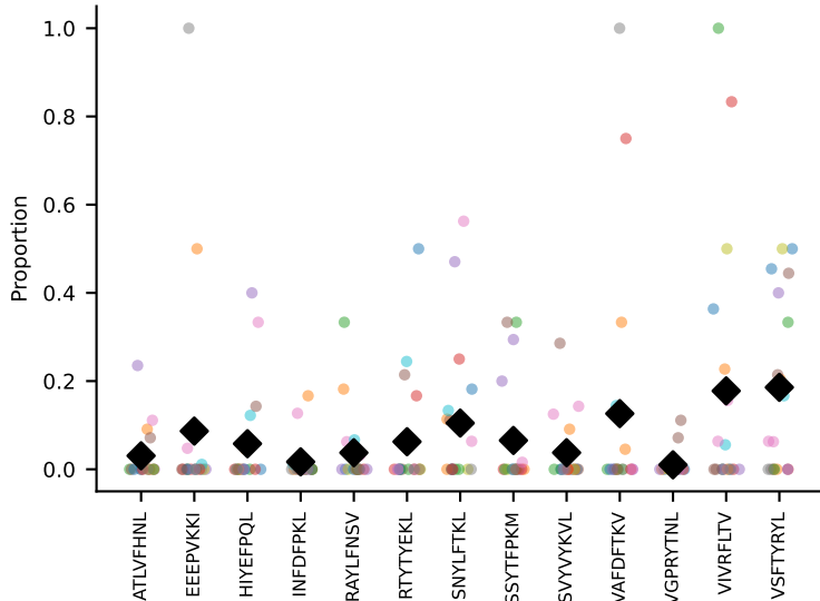
#73 AV7-3-CAVSAEGADRLTF-AJ45_BV1-CTCSADRGGSPLYF-BJ1-6 coh=0.255, n=18
