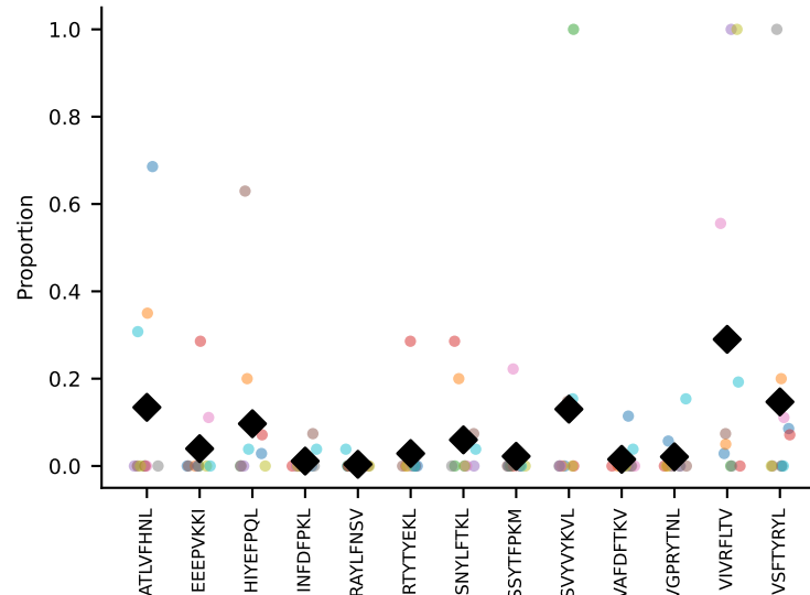
#83 AV8D-2-CATDDQGGRALIF-AJ15_BV19-CASSIGTSQNTLYF-BJ2-4 coh=0.193, n=9
