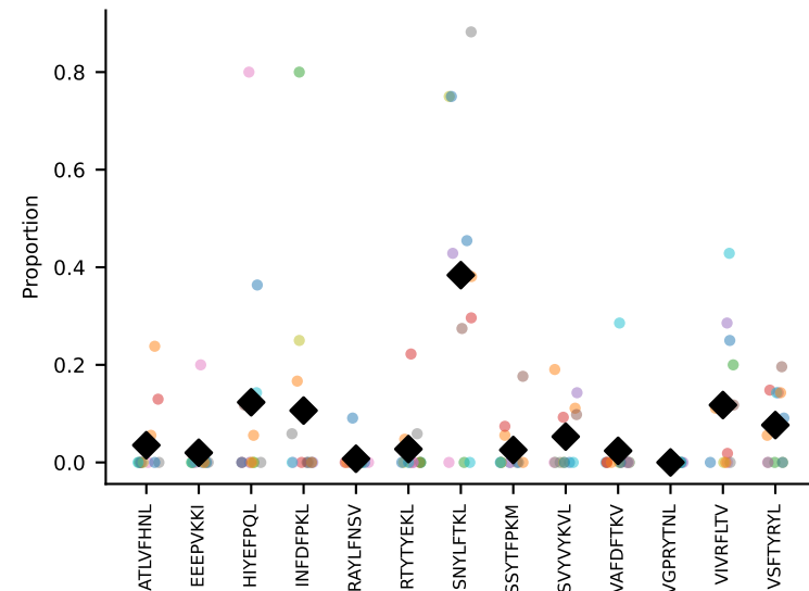
#18 AV14-1-CAASADTGNYKYVF-AJ40_BV13-3-CASSDSNTEVFF-BJ1-1 coh=0.447, n=7
