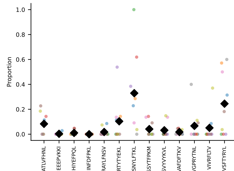
#21 AV7-5-CAVRNAGAKLTF-AJ39_BV1-CTCSATGGGNQAPLF-BJ1-5 coh=0.405, n=12
