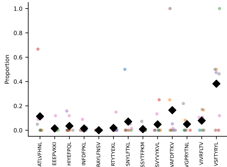
#23 AV14D-3/DV8-CAASASSGSWQLIF-AJ22_BV31-CAWSPLQGANTEVFF- coh=0.403, n=8
