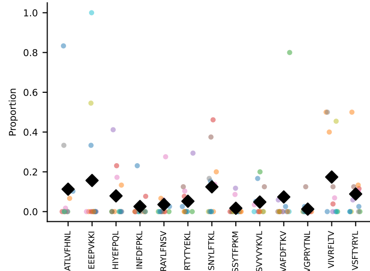
#74 AV17-CALEGSYGNEKITF-AJ48_BV1-CTCSGDRVSYEQYF-BJ2-7 coh=0.240, n=12
