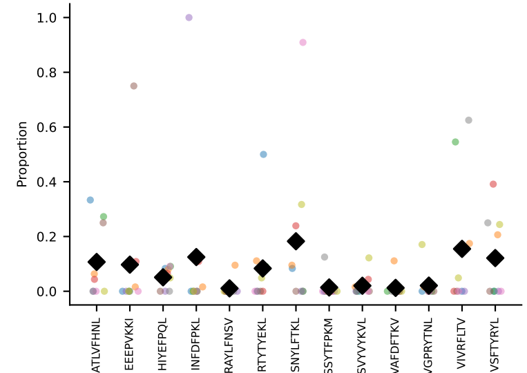
#76 AV8-1-CATDYDTNAYKVIF-AJ30_BV13-2-CASGDPIRNERLFF-BJ1-4 coh=0.238, n=9
