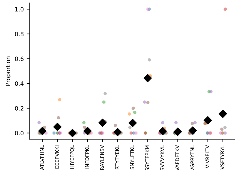
#20 AV14D-1-CAASADSGTYQRF-AJ13_BV13-2-CASGDALGDYEQYF-BJ2 coh=0.406, n=7
