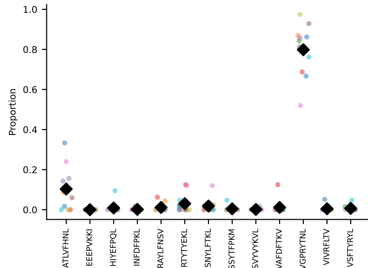
#148 AV14D-1-CAASSGSWQLIF-AJ22_BV17-CASRSRDIYNSPLYF-BJ1-6 coh=0.956, n=63
