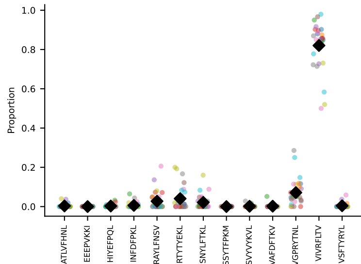
#121 AV16-CAMREANYGNEKITf-AJ48_BV31-CAWSLRDINERLFF-BJ1-4 coh=0.971, n=10
