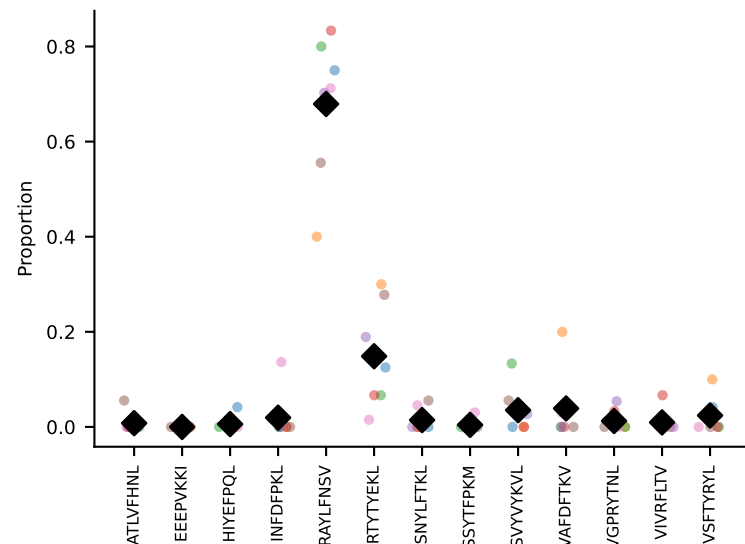
#211 AV12D-3-CALIASGSWQLIF-AJ22_BV13-2-CASGDAGNQAPLF-BJ1-5 coh=0.912, n=5
