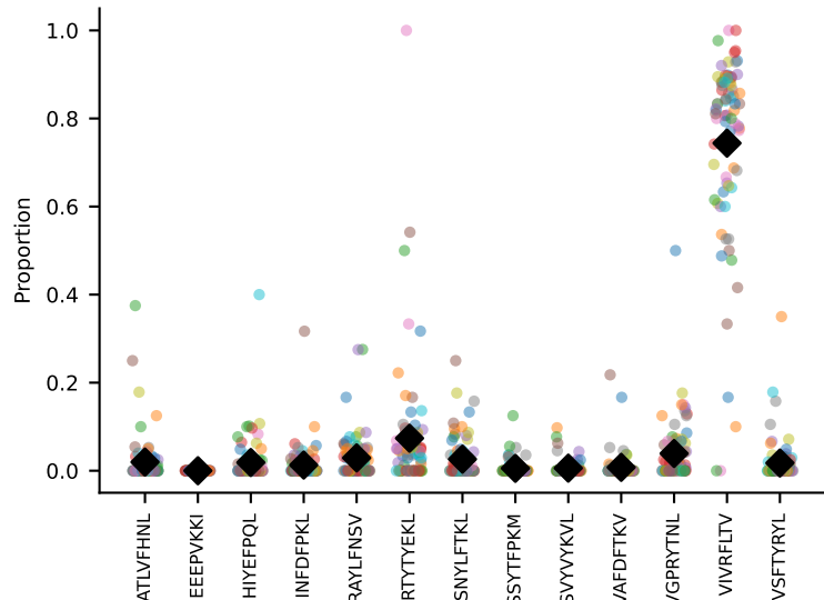
#399 AV13-1-CALVTGYQNFYF-AJ49_BV5-CASSQDRSQNTLYF-BJ2-4 coh=0.861, n=11
