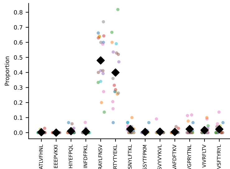
#263 AV7-2-CAASKGGRALIF-AJ15_BV12-2-CASSSGQGGISDYTF-BJ1-2 coh=0.838, n=8
