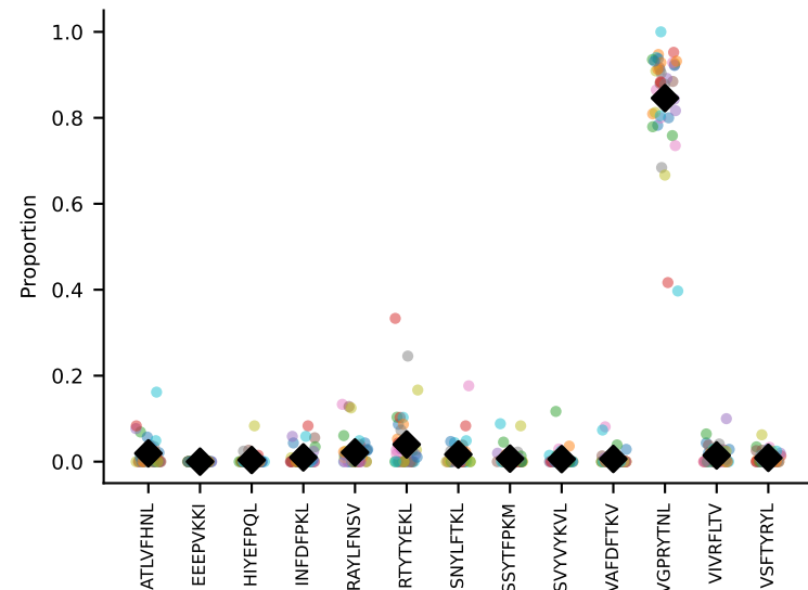
#119 AV9-4-CAVSVDYANKMIF-AJ47_BV3-CASSLGTGYEYf-BJ2-7 coh=0.972, n=31
