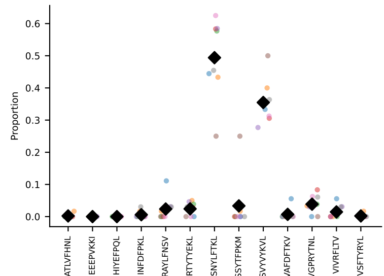
#203 AV8D-2-CATDTGKLTF-AJ27_BV3-CASSLDSNERLFF-BJ1-4 coh=0.920, n=8
