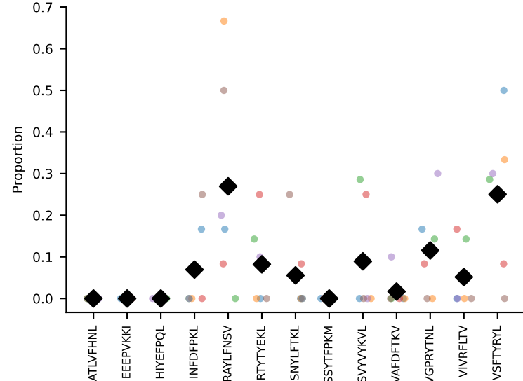
#439 AV8N-2-CATEDQGGRALIF-AJ15_BV5-CASSQEAISNERLFF-BJ1-4 coh=0.472, n=6
