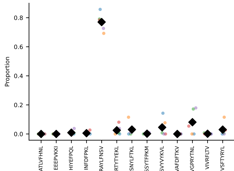
#376 AV5-1-CSASTDYANKMIF-AJ47_BV3-CASSLSGGNTQYf-BJ2-5 coh=0.969, n=5
