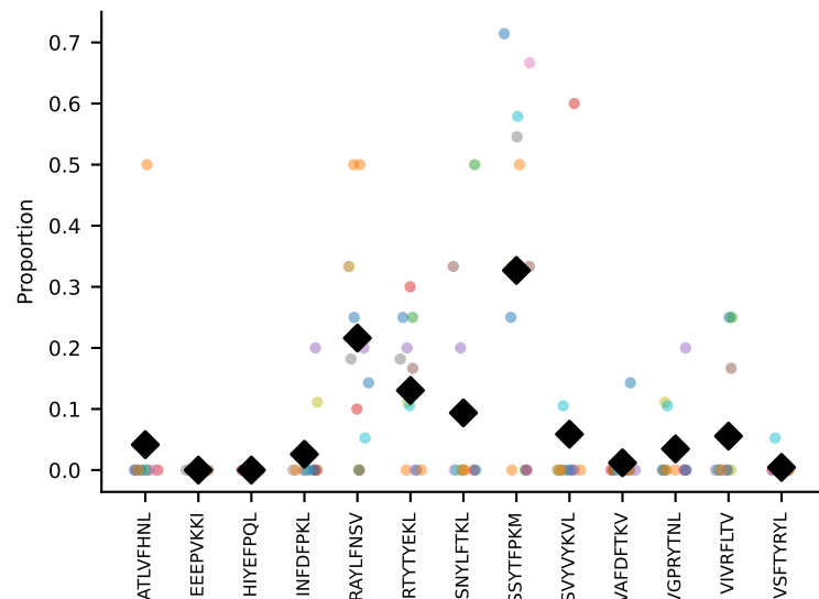
#357 AV8D-2-CATDAEGGRALIF-AJ15_BV13-3-CASSGGPTGQLYF-BJ2-2 coh=0.446, n=44
