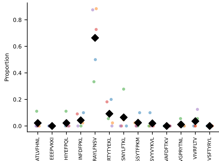
#403 AV16N-CAMRDTNAYKVIF-AJ30_BV13-2-CASGGANERLFF-BJ1-4 coh=0.845, n=18
