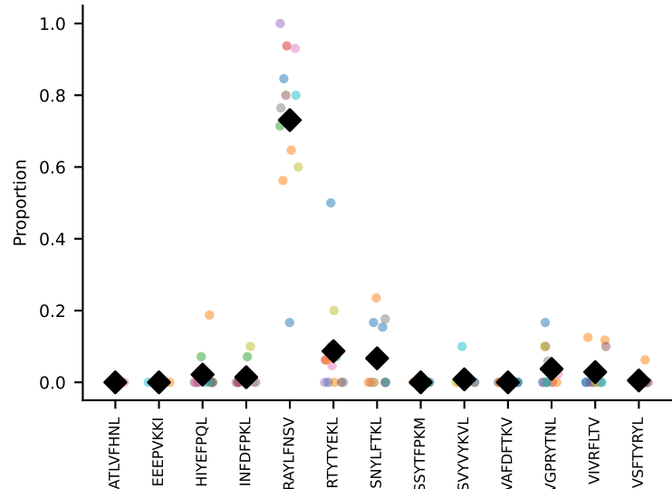
#252 AV16-CAMREDSNYQLIW-AJ33_BV3-CASSPGQISNERLFF-BJ1-4 coh=0.856, n=12
