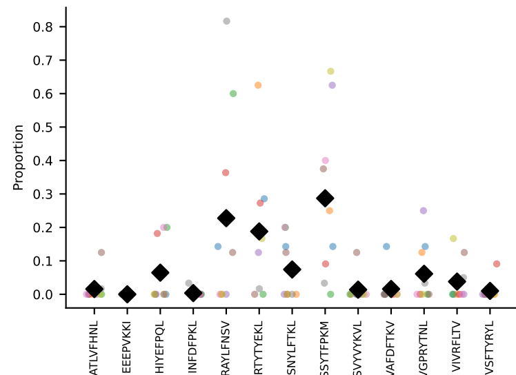
#355 AV16-CAMREGQGGSAKLIF-AJ57_BV1-CTCSADRFYEQYF-BJ2-7 coh=0.452, n=14
