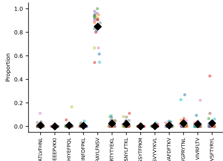
#138 AV7-5-CAVSMDYANKMIF-AJ47_BV3-CASSLAAVYEQYF-BJ2-7 coh=0.961, n=149
