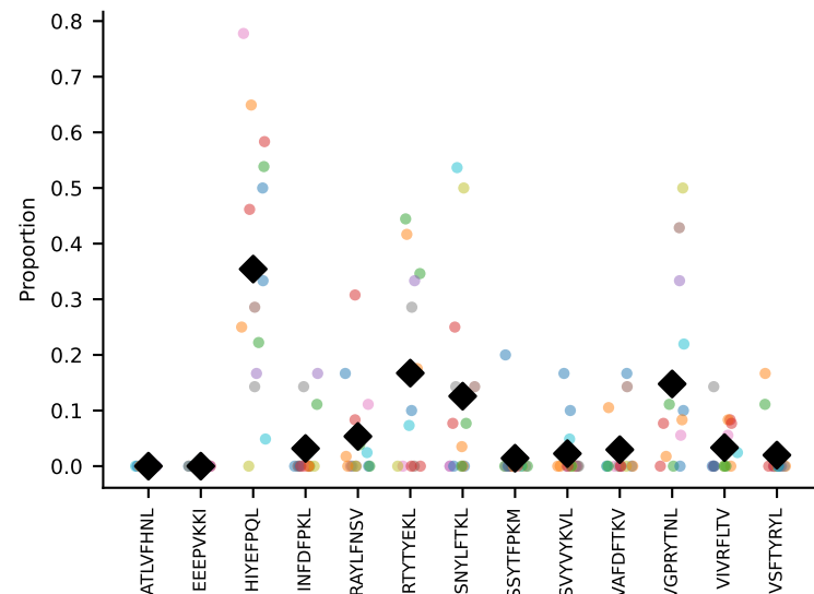
#343 AV6-6-CALGEAGGSNAKLTF-AJ42_BV14-CASSPGLSYNSPLYF-BJ1-6 coh=0.525, n=5
