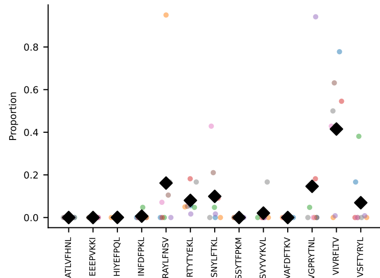
#442 AV19-CAAGSNYQLIW-AJ33_BV1-CTCSADWVSNERLFF-BJ1-4 coh=0.457, n=5
