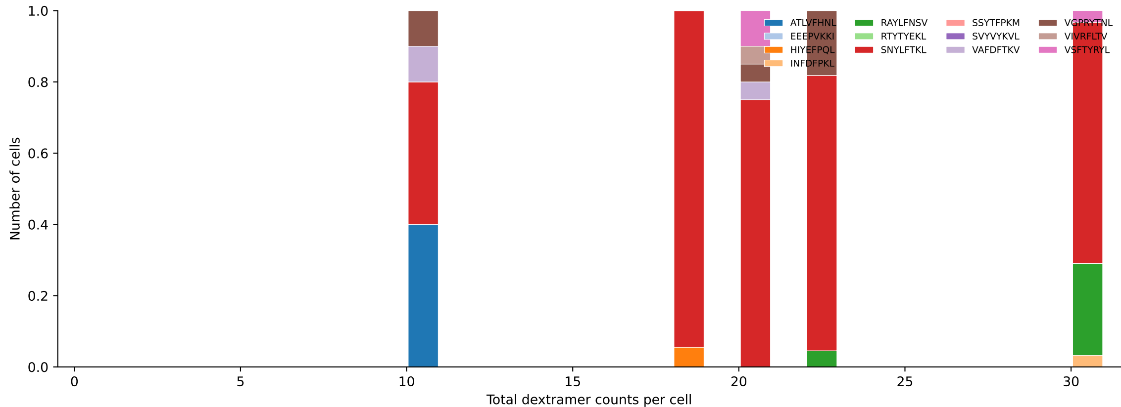
B10BR_HIL Combined | #404 AV7-2-CAAINNTNTGKLTf-AJ27_BV13-2-CASGDAGGGNERLFF-BJ1-4 (n=5) Total pMHC histogram — stacked by mean peptide proportion per bin [404/461]
