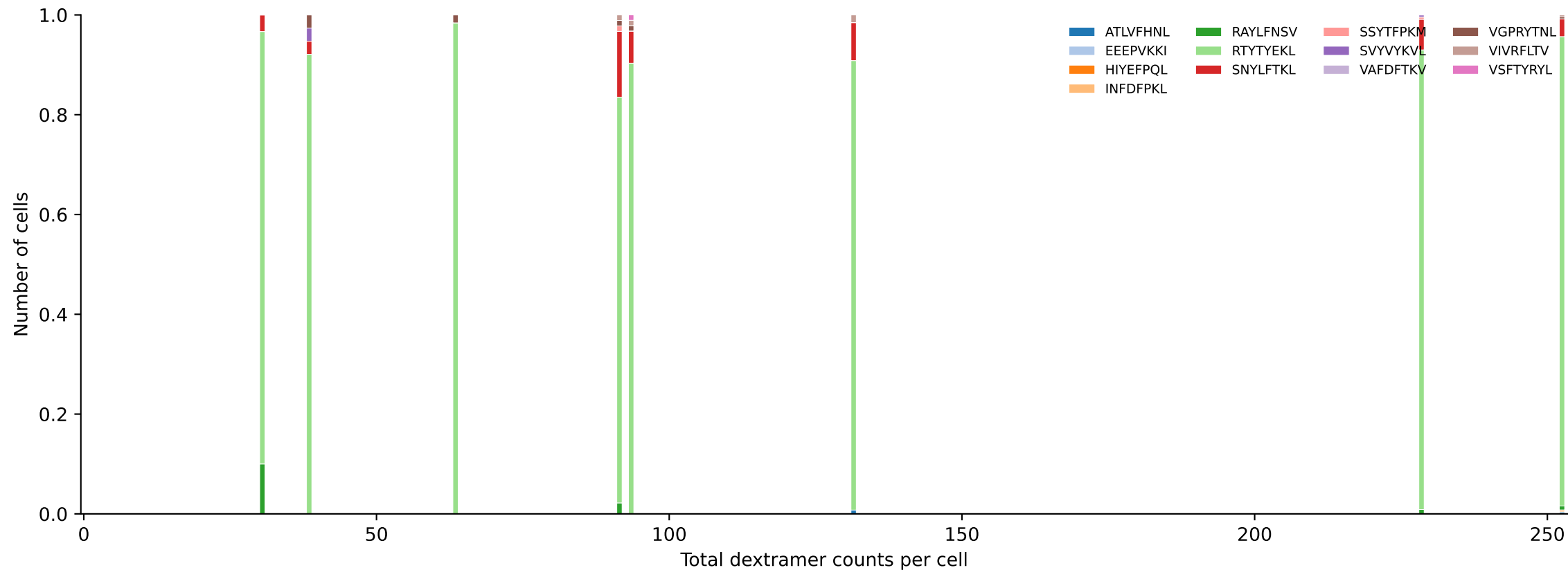
B10BR_HIL Combined | #248 AV16N-CAMREVSNYNVLYF-AJ21_BV13-2-CASGDQGNSGNTLYF-BJ1-3 (n=8) Total pMHC histogram — stacked by mean peptide proportion per bin [248/461]
