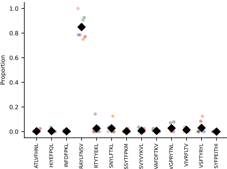
#31 AV16D/DV11-CAMREGSSGSWQLIF-AJ22_BV13-1-CASSDVGDEQYF-BJ2-7 coh=0.983, n=8
