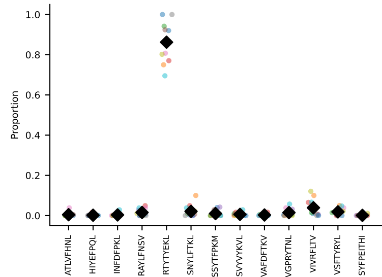
#24 AV9D-4-CALSANMGYKLTF-AJ9_BV13-1-CASSEGTGGIYEYF-BJ2-7 coh=0.989, n=10
