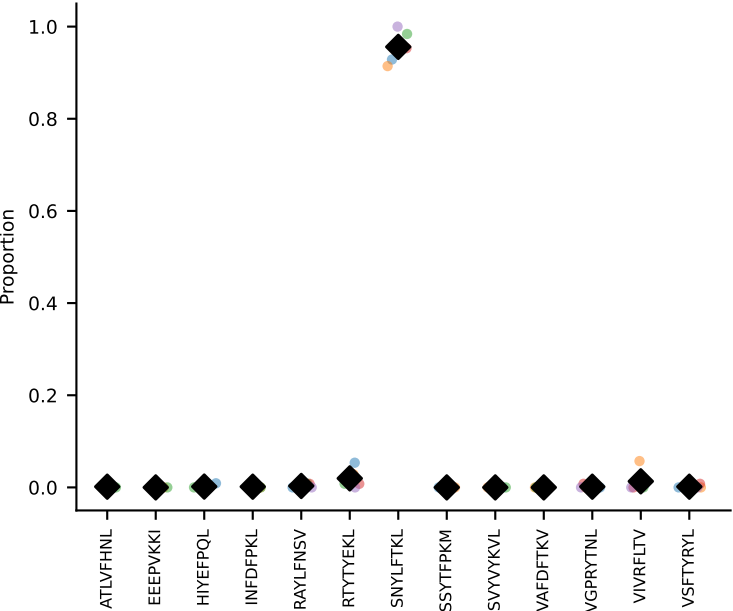
#2 AV16/DV11-CAMREGTNAYKVIF-AJ30_BV13-2-CASGDAWGQAGNTLYF-BJ1-3 coh=0.999, n=5
