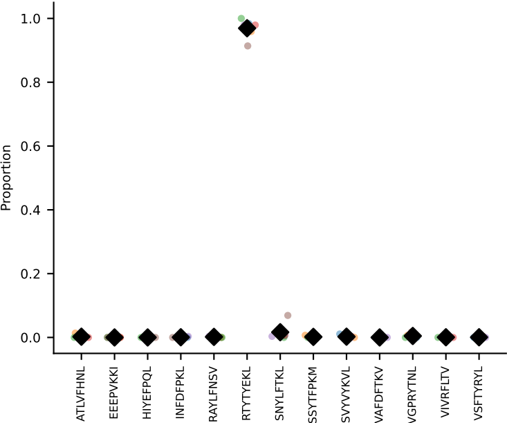
#1 AV16-CAMRKEGADRLTF-AJ45_BV13-1-CASSDNYEQYF-BJ2-7 coh=0.999, n=6
