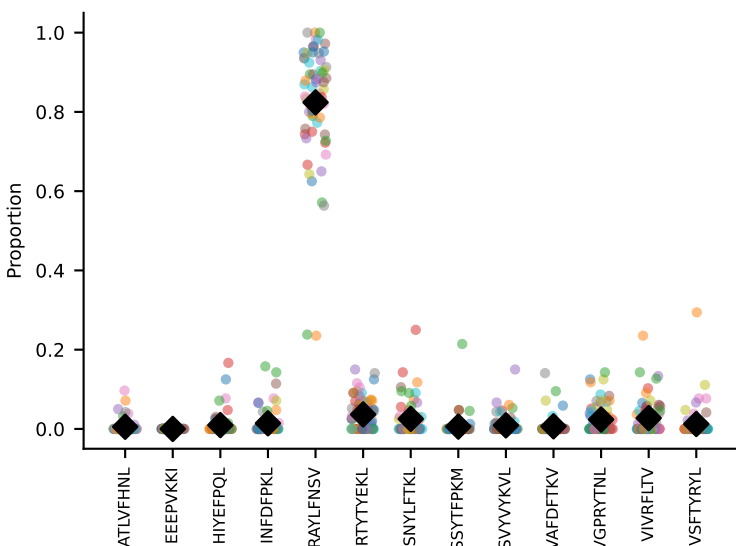
#69 AV16N-CAMRDDTNAYKVIF-AJ30_BV1-CTCSRDREGREYF-BJ2-7 coh=0.952, n=5
