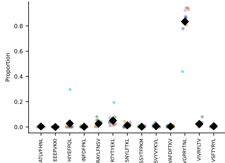
#60 AV8D-2-CATDATNYNVLYF-AJ21_BV3-CASSLQQEYEF-BJ2-7 coh=0.959, n=11
