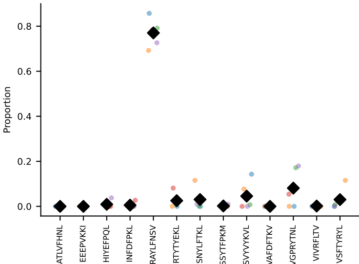
#53 AV16N-CAMREDSNYQLIW-AJ33_BV16-CASSLDGLNYAEQFF-BJ2-1 coh=0.964, n=9
