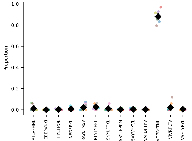
#18 AV7-2-CAATGNTGKLIF-AJ37_BV13-1-CASSDARVGEQYF-BJ2-7 coh=0.993, n=43
