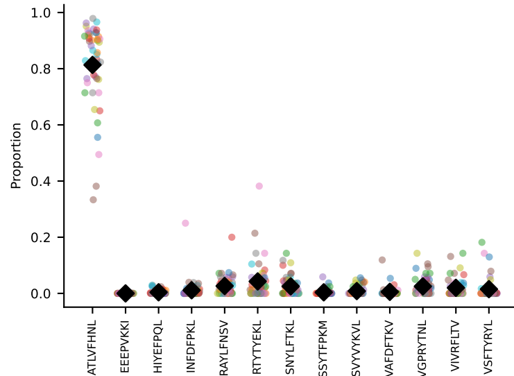
#59 AV16-CAMREDSNYQLIW-AJ33_BV3-CASSQGQISNERLFF-BJ1-4 coh=0.960, n=12
