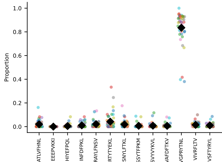
#54 AV8-1-CATDASSGSWQLIF-AJ22_BV13-2-CASGDEGTYNsPLYF-BJ1-6 coh=0.964, n=20
