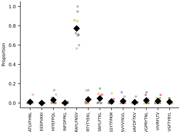
#57 AV16/DV11-CAMRADSNYQLIW-AJ33_BV3-CASSRGQISNERLFF-BJ1-4 coh=0.962, n=27
