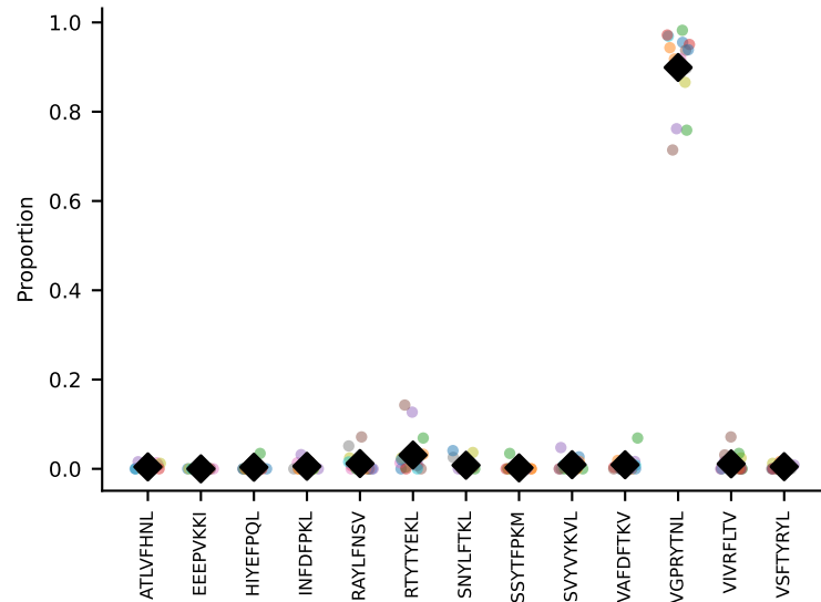
#19 AV14-2-CAASPSGSWQLIF-AJ22_BV13-1-CASSGGSDYTF-BJ1-2 coh=0.992, n=6
