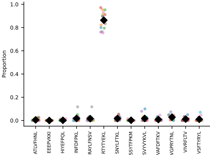
#21 AV16N-CAMRENNYAQGLTF-AJ26_BV13-2-CASGDWGWGEQYF-BJ2-7 coh=0.991, n=53
