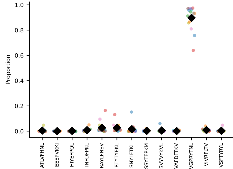
#24 AV14-1-CAARNTEGADRLTF-AJ45_BV3-CASSFSGGYEQYF-BJ2-7 coh=0.989, n=15
