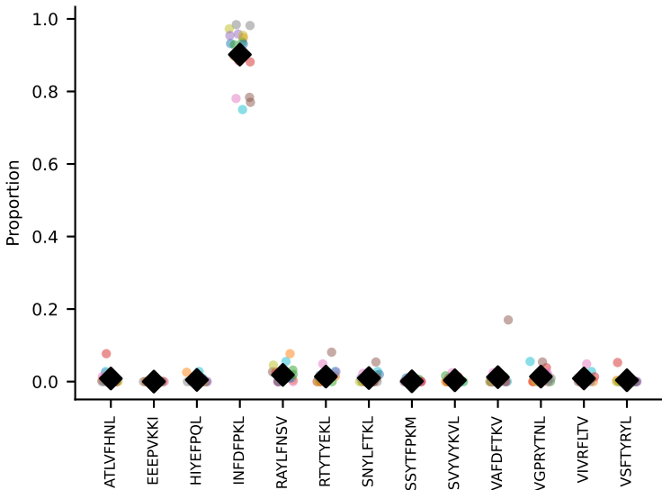
#17 AV7-2-CAAMSNYNVLYF-AJ21_BV31-CAWKTGGLNYAEQFF-BJ2-1 coh=0.993, n=17
