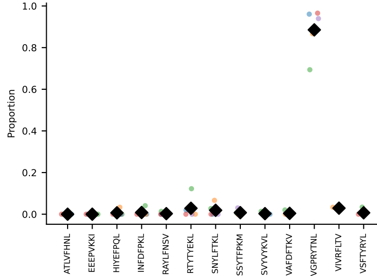
#22 AV6D-7-CALNTEGADRLTF-AJ45_BV3-CASSLGTGWYEQYF-BJ2-7 coh=0.991, n=5
