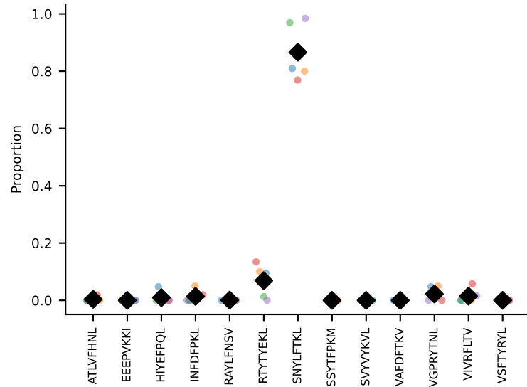
#23 AV9D-3-CALVSNTNKVVF-AJ34_BV13-1-CASSDVNTEVFF-BJ1-1 coh=0.991, n=5
