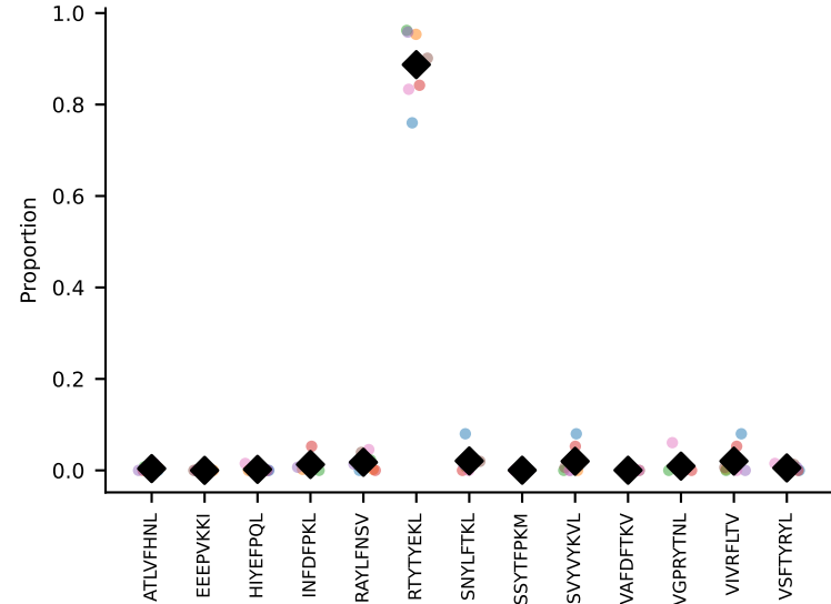
#20 AV7-2-CAAASSGSWQLIF-AJ22_BV13-1-CASSDAGYEQYF-BJ2-7 coh=0.992, n=7
