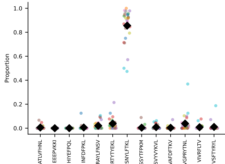
#55 AV13-1-CALEQGGS AKLIF-AJ57_BV12-2-CASSLEGADTEVFF-BJ1-1 coh=0.964, n=48
