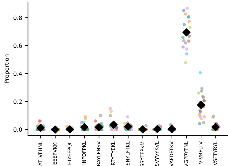
#58 AV13-2-CAPNNNAGAKLTf-AJ39_BV14-CASSDRIEYF-BJ2-7 coh=0.961, n=91
