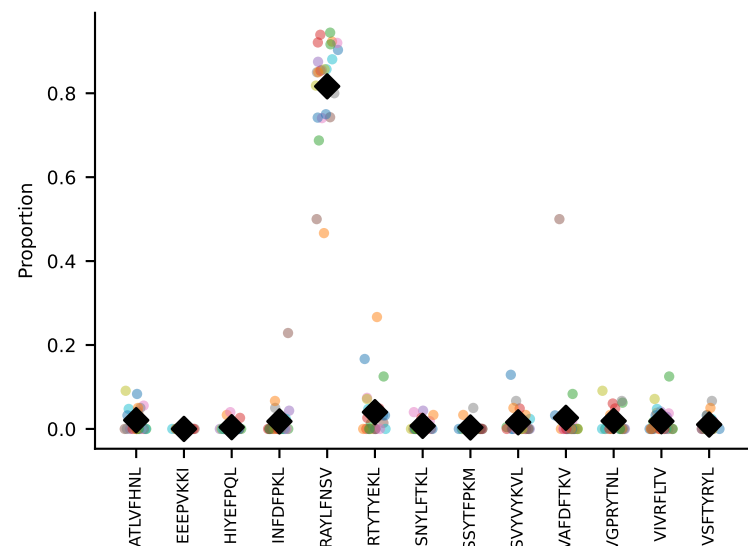
#72 AV7-1-CAATSSGQKLVF-AJ16_BV13-1-CASSDVGGRG TGQLYF-BJ2-4 coh=0.950, n=20
