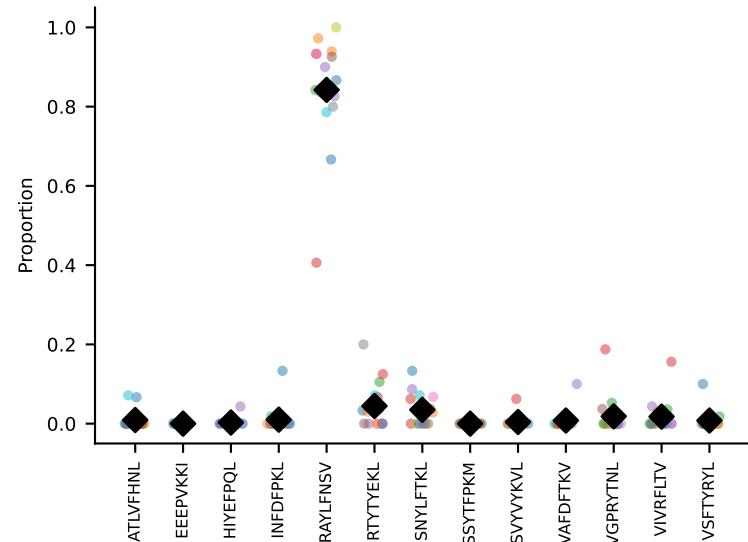
#56 AV14D-1-CAASAETGGYKVVf-AJ12_BV3-CASSLARGYEYF-BJ2-7 coh=0.962, n=40
