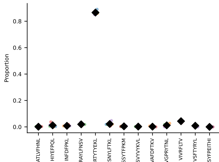
#6 AV9-2-CAASSDYANKMIF-AJ47_BV3-CASSSTGFEQYF-BJ2-7 coh=0.997, n=5
