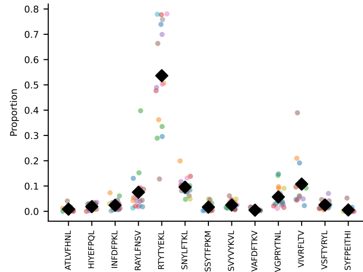
#72 AV16D/DV11-CAMREGNTGNYKYVF-AJ40_BV13-2-CASGDLYEQYF-BJ2-8 coh=0.857, n=17
