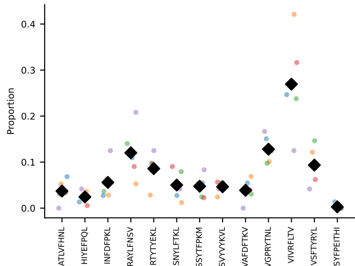
#78 AV8D-2-CATVGNRIFf-AJ31_BV1-CTCSAVRISNERLFF-BJ1-4 coh=0.845, n=21
