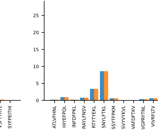
AV6-6-CALGDSNYQLIW-AJ33_BV13-3-CASRDVRSYEYQF-BJ2-7 MEAN n:5→5
