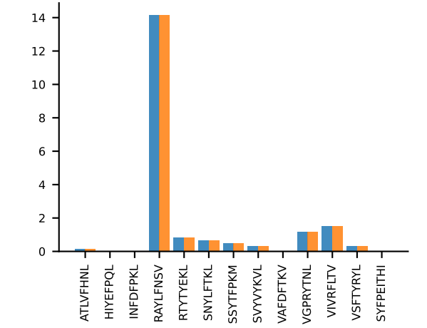
AV16/DV11-CAMRENTGYQNIFY-AJ49_BV13-2-CASGQGAGNTLYF-BJ1-1 MEAN n:5→5
