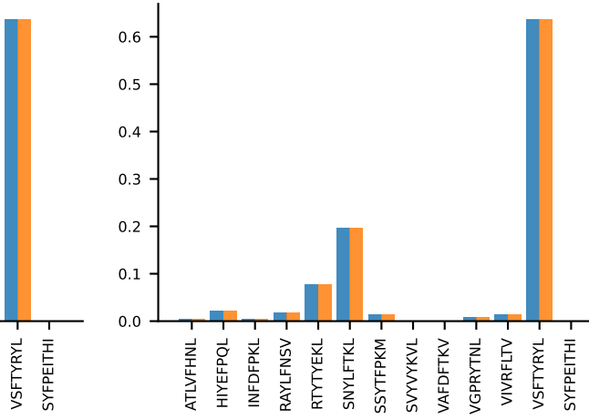
AV6-6-CALGDSNYQLIW-AJ33_BV13-3-CASRDVRSYEYQF-BJ2-7 PROP n:5→5
