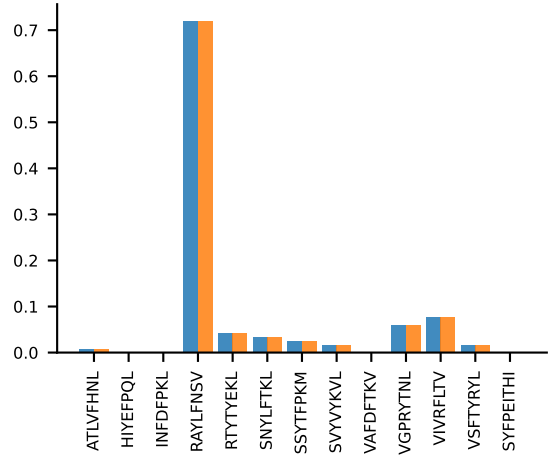
AV16/DV11-CAMRENTGYQNIFY-AJ49_BV13-2-CASGQGAGNTLYF-BJ1-1 PROP n:5→5
