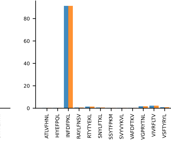
AV16/DV11-CAMREGRGGSAKLIF-AJ57_BV13-3-CASSWTGSYNPLFY-BJ1-1 MEAN n:5→5
