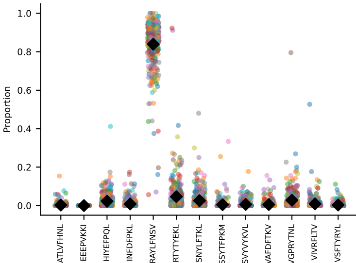
#77 AV16N-CAMREGNMGYKLTf-AJ9_BV13-2-CASGDNQGNsDYTF-BJ1-2 coh=0.956, n=29
