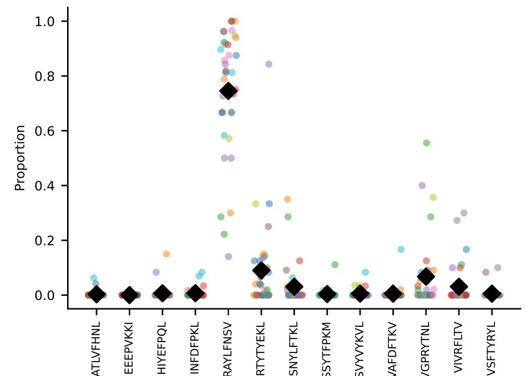
#167 AV16/DV11-CAMREDSTGYQNIFYF-AJ49_BV13-2-CASGTGGANTLYF-BJ2-4#168 AV16/DV11-CAMREDSTGYQNIFYF-AJ49_BV13-2-CASGTGGANTLYF-BJ2-4 coh=0.832, n=12
