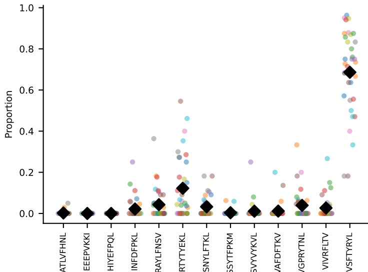
#161 AV16/DV11-CAMREDSTGYQNIFYF-AJ49_BV13-2-CASGTGGANTLYF-BJ2-4#162 AV16/DV11-CAMREDSTGYQNIFYF-AJ49_BV13-2-CASGTGGANTLYF-BJ2-4 coh=0.836, n=19
