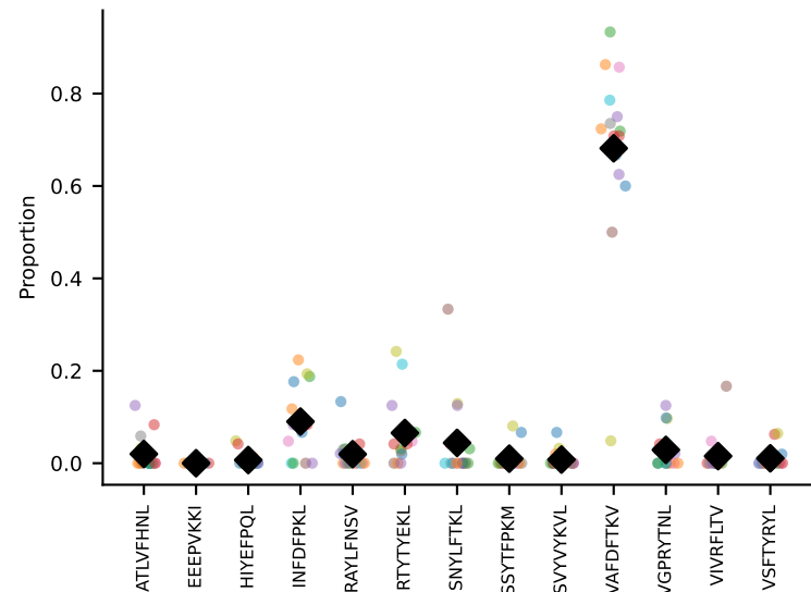
#155 AV12-2-CAASVSGDSNNRIFF-AJ31_BV1-CTCSAVRVQDTQYF-BJ2-5#156 AV16/DV11-CAMREDSNYQLIW-AJ33_BV3-CASSPGQISNERLFF-BJ1-6 coh=0.841, n=28
