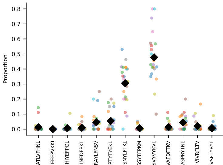
#153 AV19-CAAGATGYQNIFYF-AJ49_BV17-CASSRLGSSYEQYF-BJ2-7#154 AV3-3-CAVSATTNYGNEKITF-AJ48_BV13-1-CASSDLGGDTQYF-BJ2-5 coh=0.846, n=34
