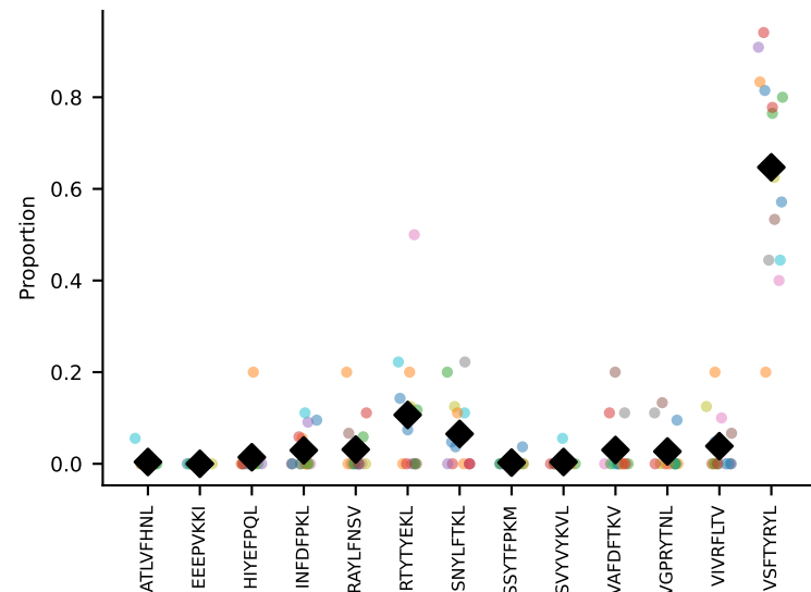
#163 AV16/DV11-CAMREDSTGYQNIFYF-AJ49_BV13-2-CASGTGGANTLYF-BJ2-4#164 AV16/DV11-CAMREDSTGYQNIFYF-AJ49_BV13-2-CASGTGGANTLYF-BJ2-4 coh=0.835, n=14
