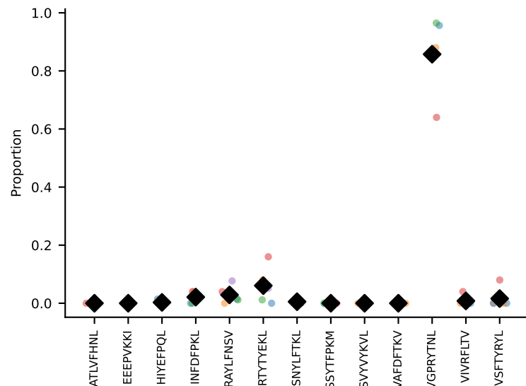
#47 AV16-CAMREGGAGNTGKLIF-AJ37_BV13-2-CASGELYEYF-BJ2-7 coh=0.982, n=9
