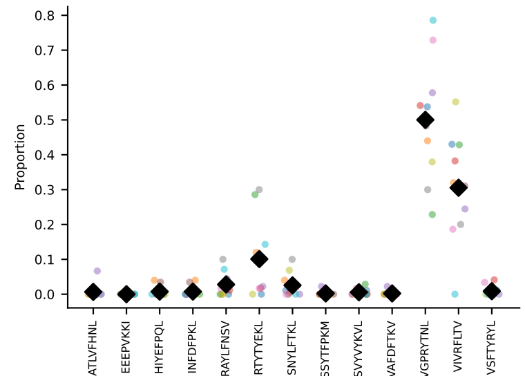
#159 AV16/DV11-CAMREDSTGYQNIFYF-AJ49_BV13-2-CASGTGGANTLYF-BJ2-4#160 AV16/DV11-CAMREDSTGYQNIFYF-AJ49_BV13-2-CASGTGGANTLYF-BJ2-4 coh=0.836, n=35
