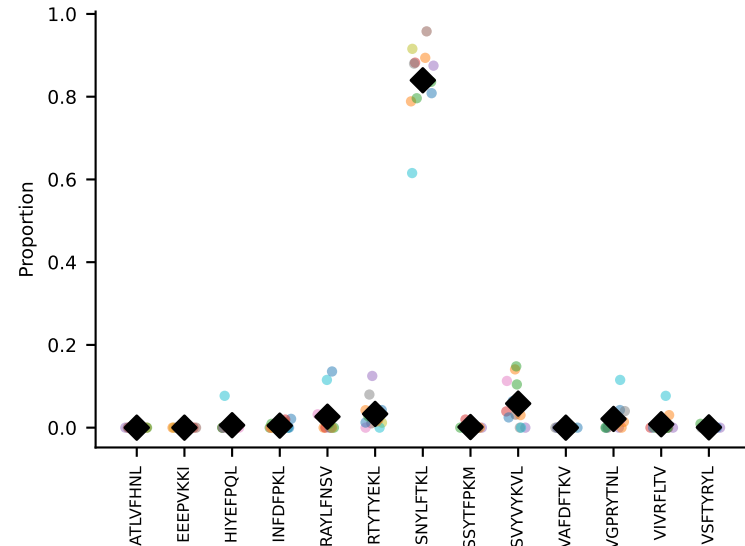
#41 AV17-CALGNNAGAKLTF-AJ39_BV13-1-CASSILGGSYEYF-BJ2-7 coh=0.985, n=15
