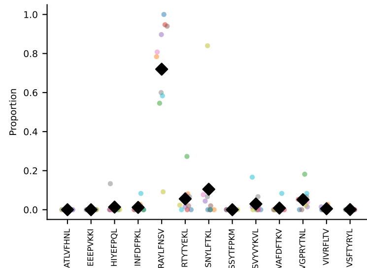
#173 AV14D-3/DV8-CAASEGSALGRLHF-AJ18_BV12-2-CASSLDSNQDTQYF-BJ2-2 coh=0.783, n=5
