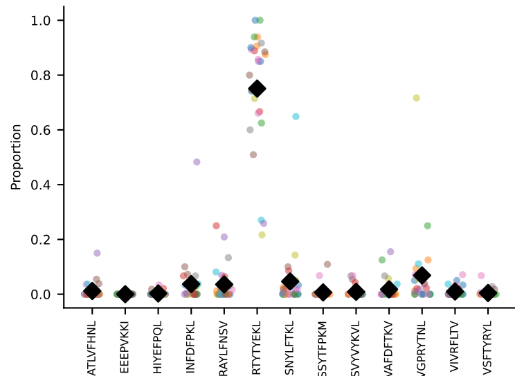
#157 AV16N-CAMLTGYQNIFYF-AJ49_BV1-CTCSADRGVNSPLYF-BJ1-6#158 AV16/DV11-CAMREDSTGYQNIFYF-AJ49_BV13-2-CASGTGGANTLYF-BJ2-4 coh=0.838, n=21
