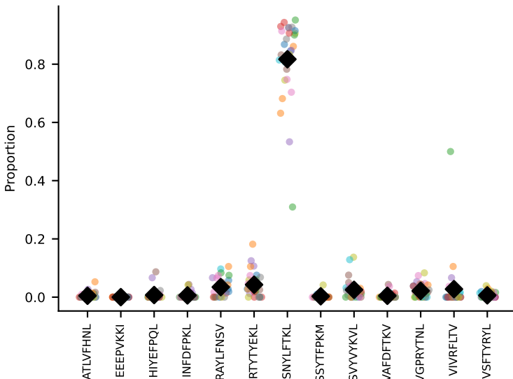
#81 AV16/DV11-CAMRESNTGYQNfYF-AJ49_BV13-2-CASGEGQGKNTLYF-BJ2-4 coh=0.953, n=7
