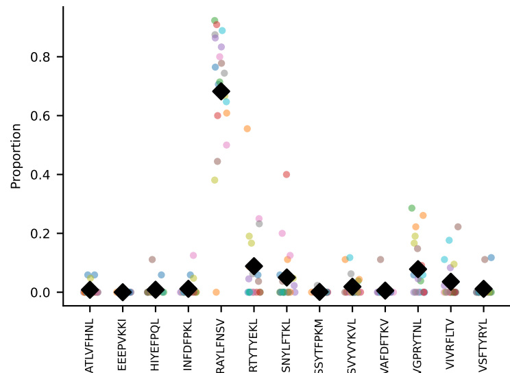
#165 AV16/DV11-CAMREDSTGYQNIFYF-AJ49_BV13-2-CASGTGGANTLYF-BJ2-4#166 AV16/DV11-CAMREDSTGYQNIFYF-AJ49_BV13-2-CASGTGGANTLYF-BJ2-4 coh=0.832, n=20
