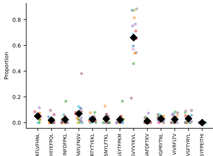
#102 AV16/DV11-CAMREANYGNEKITF-AJ48_BV1-CTCSADRVHSDYTF-BJ2-5 coh=0.881, n=6
