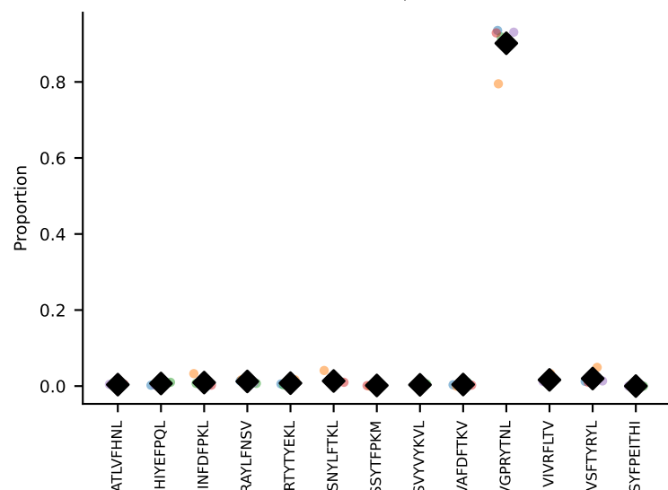
#11 AV6-4-CALVTDYAQGLTF-AJ26_BV3-CASSLAGDEQYF-BJ2-7 coh=0.999, n=5
