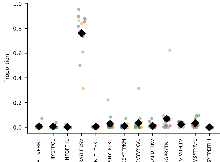
#103 AV16D/DV11-CAMREGSSGSWLIF-AJ22_BV1-CTCSADRAETLYF-BJ2-3 coh=0.880, n=7
