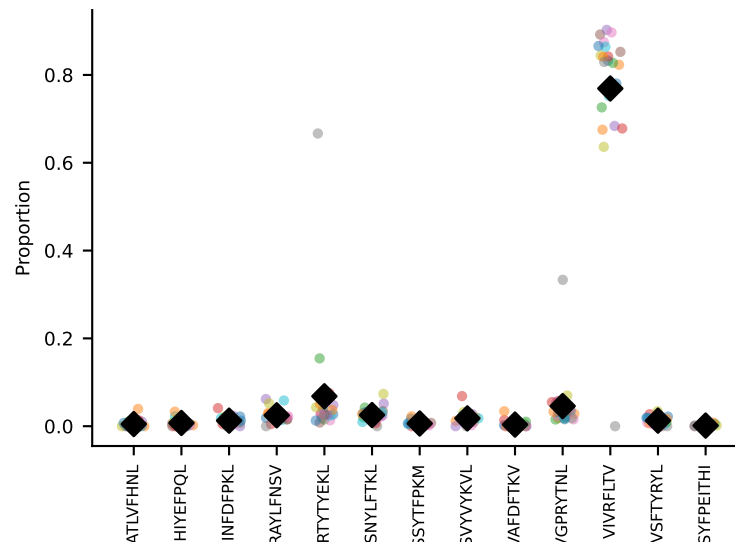
#73 AV8-1-CATDASSGSWQLIF-AJ22_BV4-CASTAANTEVFF-BJ1-1 coh=0.910, n=22
