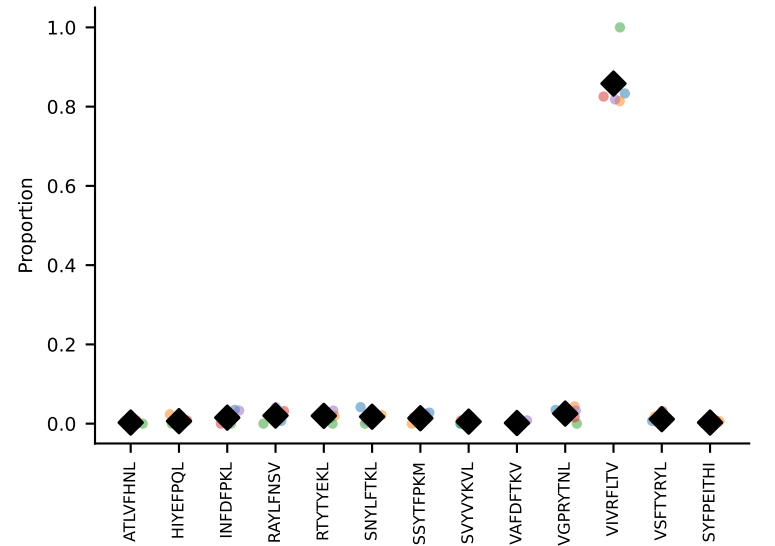
#8 AV12-1-CALSDPSNTDKVVF-AJ34*p03_BV13-1-CASSPHYNYAEQFF-BJ2-1 coh=0.996, n=10
