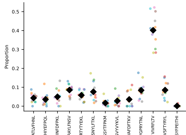
#71 AV8-1-CATDASSGSWQLIF-AJ22_BV4-CASTAANTEVFF-BJ1-1 coh=0.912, n=12
