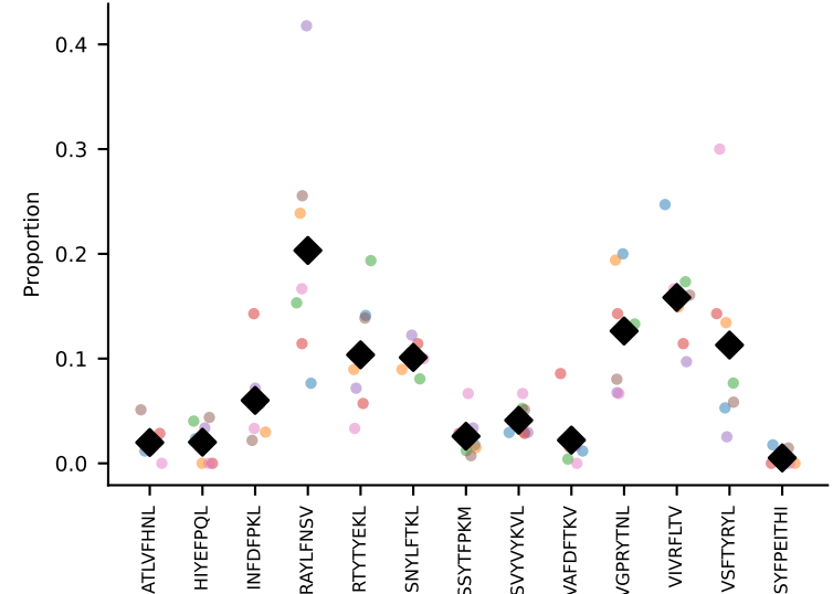
#115 AV12-2-CALSDTGANTGKLTf-AJ52_BV1-CTCSADPSYEQYf-BJ2-7#116 AV16/DV11-CAMREGLGGNNKLTf-AJ56_BV1-CTCSAAGTGNTVFF-BJ2-5 coh=0.781, n=7
