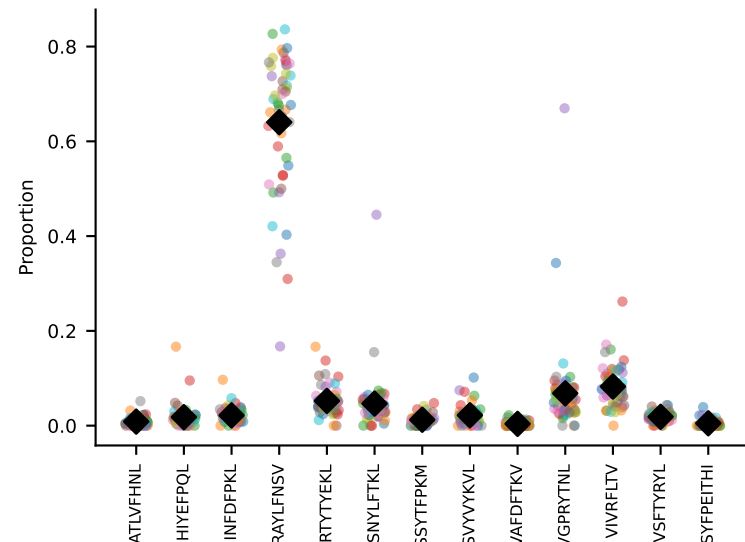
#61 AV1-CAVRDSYAQGLTF-AJ26_BV13-1-CASSDDRVGNTLYF-BJ1-3 coh=0.927, n=50
