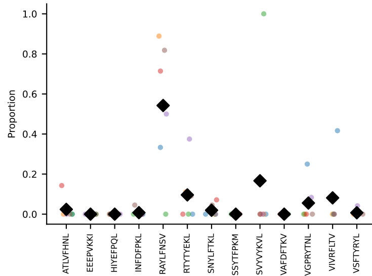
#223 AV8N-2-CATEDQGGRALIF-AJ15_BV5-CASSQEASNERLFF-BJ1-4 coh=0.472, n=6
