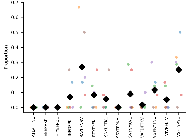
#227 AV3-3-CAVSASNAGAKLTF-AJ39_BV5-CASSPDRGDERLFF-BJ1-4 coh=0.455, n=55
