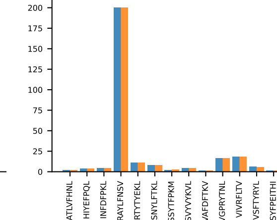
AV12D-1-CALSDQNKLTf-AJ56_BV14-CASRS DWNQDTQYF-BJ2-7 MEAN n:24→24
