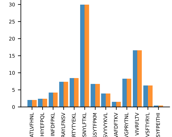
AV4-3-CAAEADTGNKYKVF-AJ40_BV31-CAWSLWTGVEQYF-BJ2-7 MEAN n:31→29
