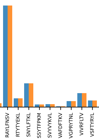
AV16D/DV11-CAMREDNNRIFF-AJ31_BV13-2-CASGEIATNTGQLYF-BJ2-7 PROP n:15→14
