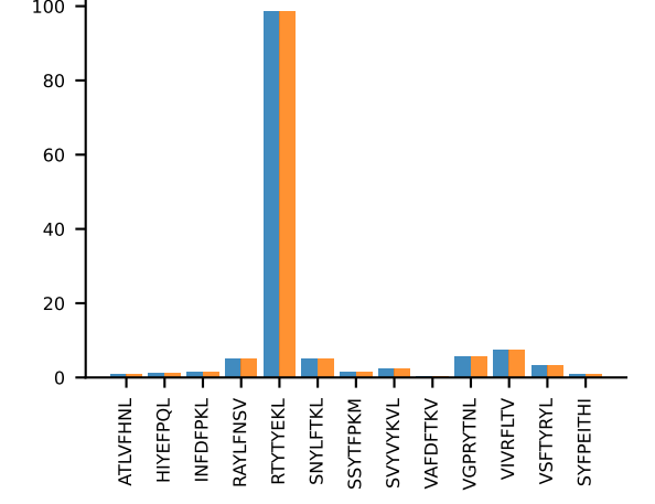
AV16/DV11-CAMRENTGANTGKLTf-AJ52_BV13-3-CASSSGGVKAEQFF-BJ2-4 MEAN n:15→15
