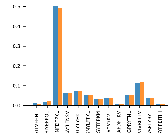
AV4-3-CAAEADTGNKYKVF-AJ40_BV31-CAWSLWTGVEQYF-BJ2-7 PROP n:31→29
