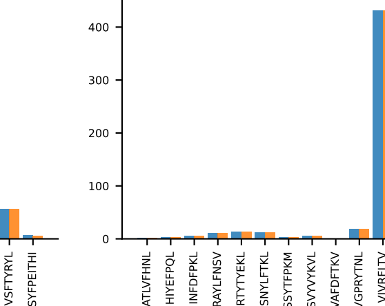
AV16D/DV11-CAMREDS SNTDKVVF-AJ34*p03_BV5-CASSQDLGGQNTLYF-BJ2-4 MEAN n:31→31
