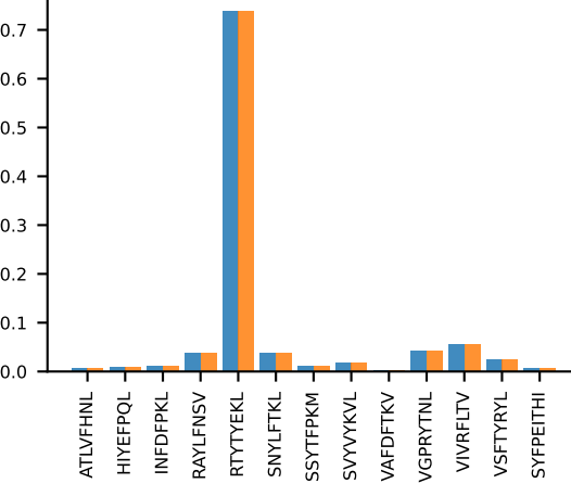
AV16/DV11-CAMRENTGANTGKLTf-AJ52_BV13-3-CASSSGGVKAEQFF-BJ2-4 PROP n:15→15
