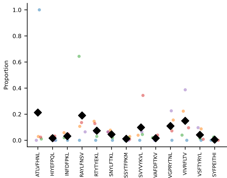
#140 AV16/DV11-CAMREDSGGSNYKLTf-AJ53_BV13-2-CASGGAGNSPLYF- coh=0.331, n=5
