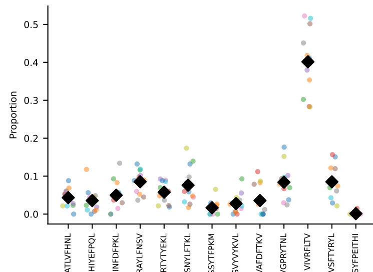
#70 AV6-6-CALGTFSENTDKVVF-AJ34*p03_BV13-1-CASSDVRDSGNTLYF-BJ1-3 coh=0.912, n=12
