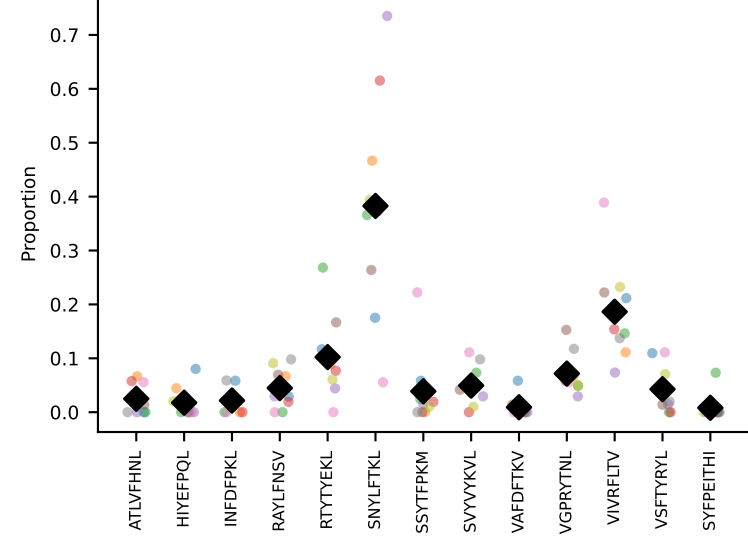
#119 AV13-1-CAMNQGS AKLIF-AJ57_BV1-CTCSALNYAEQFF-BJ2-1-#120 AV16D/DV11-CAMRDTNAYKVF-AJ30_BV13-2-CASGDVGGGQNTLYF-BJ2-1 coh=0.768, n=5
