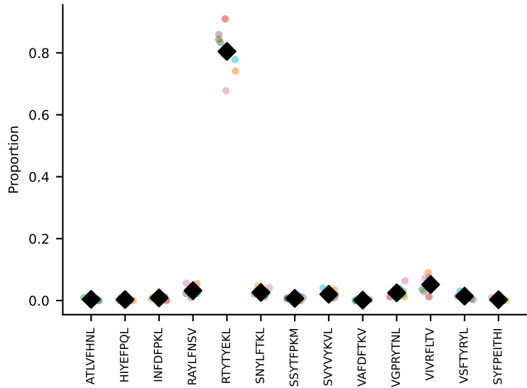
#10 AV16/DV11-CAMREDSSNTDKVVF-AJ34*p03_BV5-CASSQDLGGQNTLY-BJ2-1 coh=0.996, n=31
