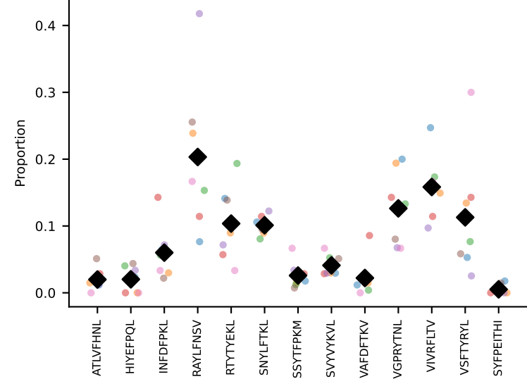
#115 AV12-2-CALSDTGANTGKLTF-AJ52_BV1-CTCSADPSYEQYF-BJ2-7-#116 AV16/DV11-CAMREGLGGNNKLTF-AJ56_BV1-CTCSAAGTGNTVFF-BJ2-1 coh=0.781, n=7
