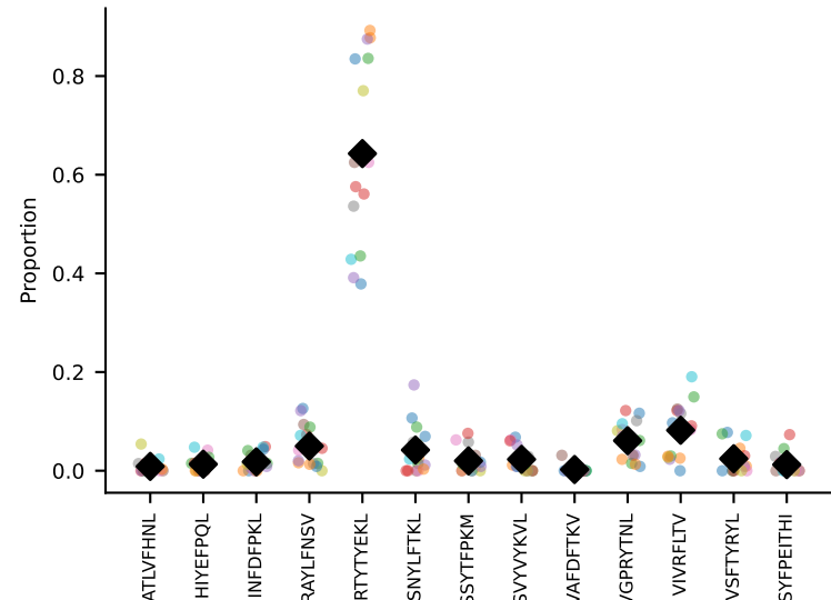
#56 AV5-1-CSASTGGFASALT F-AJ35_BV2-CASSQDGAGANSDYTF-BJ1-2 coh=0.938, n=5
