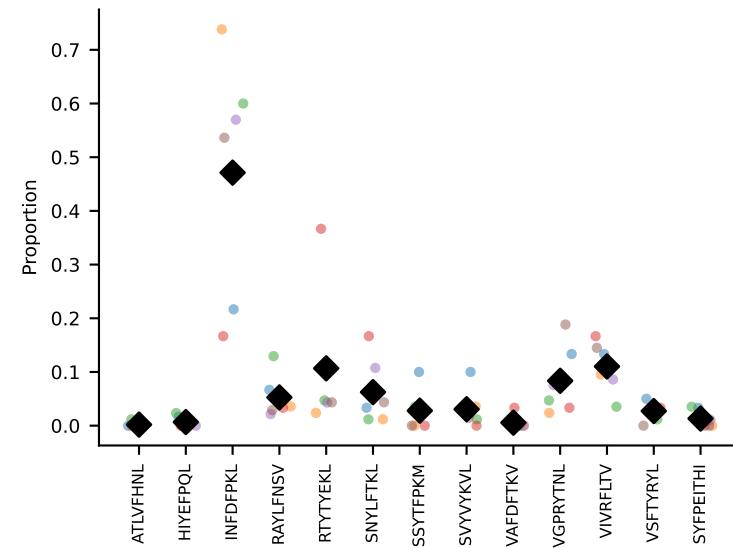
#127 AV13-1-CAANTGANTGKLTF-AJ52_BV17-CASSPGQGHTGQLYF-BJ2-2 coh=0.740, n=12
