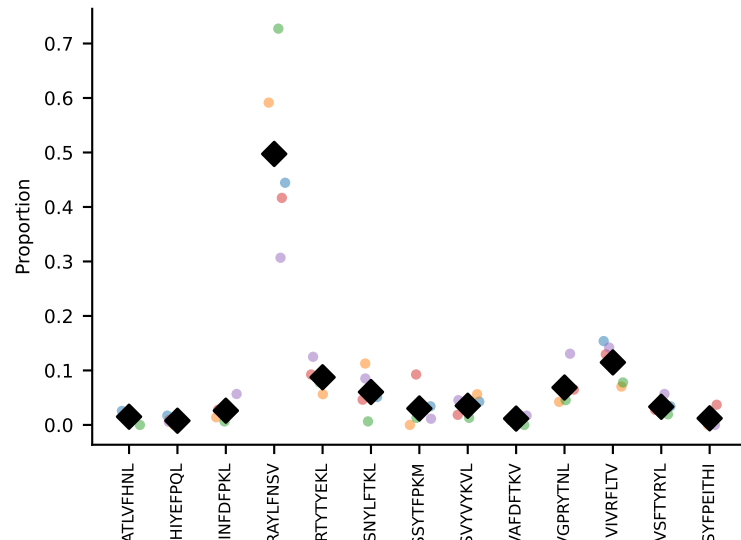
#58 AV16D/DV11-CAMREGSSGSWQLIF-AJ22_BV1-CTCSADRVYAEQFF-BJ2-1#59 AV9D-3-CAVSPDTNAYKVIF-AJ30_BV13-2-CASGDWGRGEYF-BJ2-7 coh=0.931, n=6
