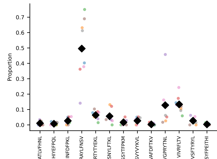
#106 AV16D/DV11-CAMREGNTNTGKLTf-AJ27_BV1-CTCSADGVYAEQFF-BJ2-1 coh=0.809, n=14
