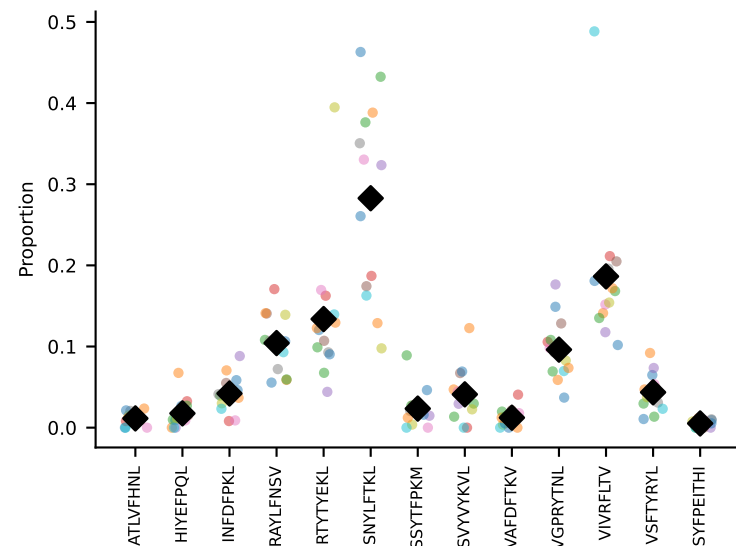
#101 AV16D/DV11-CAMREDQGGRALIF-AJ15_BV1-CTCSGQGALYEQYF-BJ2-1 coh=0.824, n=9
