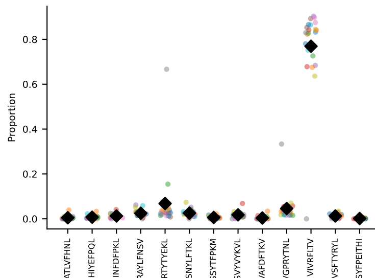
#72 AV8-1-CATDASSGSWQLIF-AJ22_BV4-CASTAANTEVFF-BJ1-1 coh=0.910, n=22
