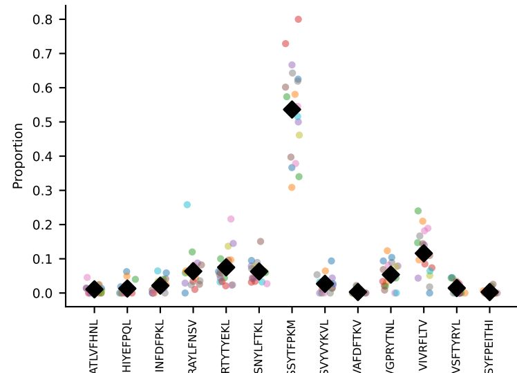
#59 AV9D-3-CAVSPDTNAYKVIF-AJ30_BV13-2-CASGDWGRGEYF-BJ2-7 coh=0.930, n=58
