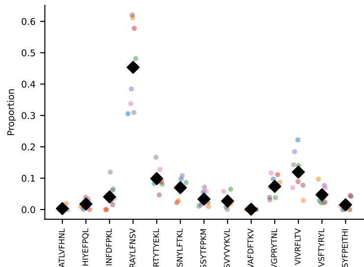
#71 AV6-6-CALGTFSENTDKVVF-AJ34*p03_BV13-1-CASSDVRDSGNTLYF-BJ1-3 coh=0.912, n=18
