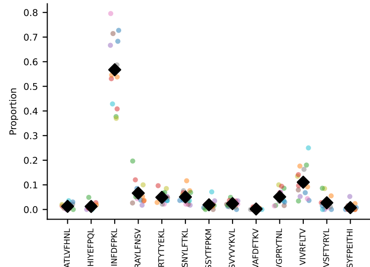
#53 AV16D/DV11-CAMREDNNRIFF-AJ31_BV13-2-CASGEIATNTGQLYF-BJ2-25 coh=0.942, n=15
