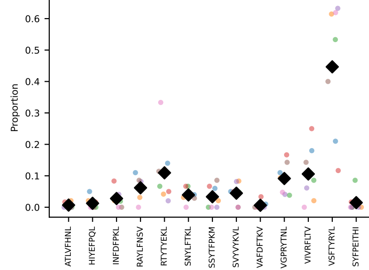
#119 AV13-1-CAMNQGS AKLIF-AJ57_BV1-CTCSALNYAEQFF-BJ2-1-#120 AV16D/DV11-CAMRDTNAYKVF-AJ30_BV13-2-CASGDVGGGQNTLYF-BJ2-1 coh=0.768, n=5
