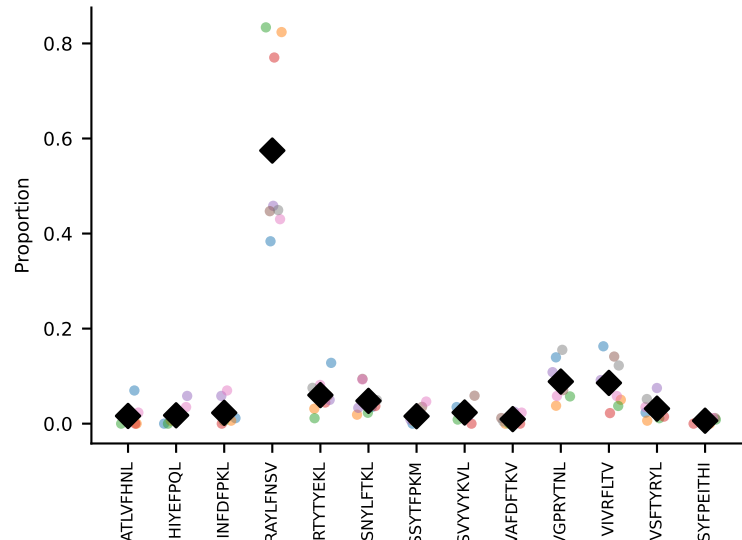
#54 AV3-3-CAVMPNYNVLYF-AJ21*p03_BV13-2-CASGDLGTDNNQAPLF-BJ1-17 coh=0.939, n=8
