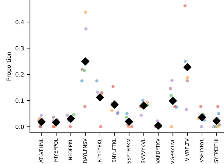
#115 AV12-2-CALSDTGANTGKLTF-AJ52_BV1-CTCSADPSYEQYF-BJ2-7-#116 AV16/DV11-CAMREGLGGNNKLTF-AJ56_BV1-CTCSAAGTGNTVFF-BJ2-1 coh=0.781, n=7
