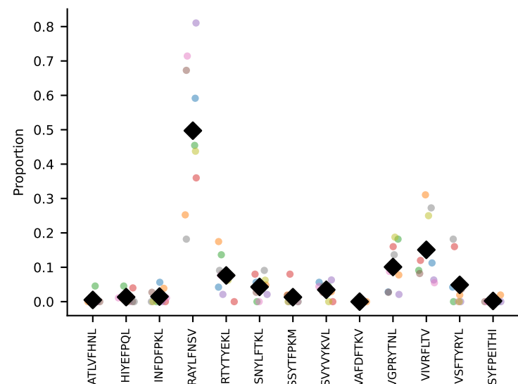
#105 AV16/DV11-CAMREGDTGYQNFYF-AJ49_BV1-CTCSADRAQDTQYF-BJ2-1 coh=0.810, n=5
