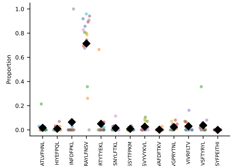
#92 AV8-1-CATEPDTGYQNIFY-AJ49_BV3-CASSLAWGLNYAEQFF-BJ2-1 coh=0.727, n=5
