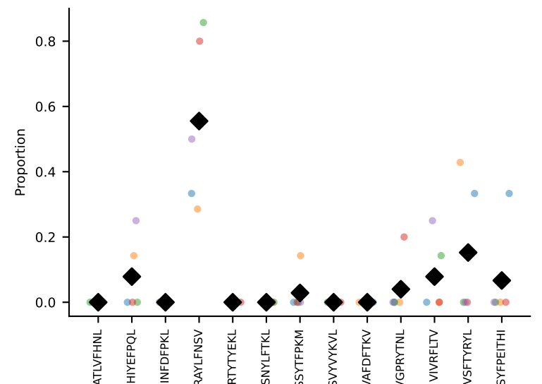
#96 AV7D-2-CAANTNTGKLTf-AJ27_BV1-CTCSADRNVNQAPLF-BJ1-5 coh=0.651, n=5
