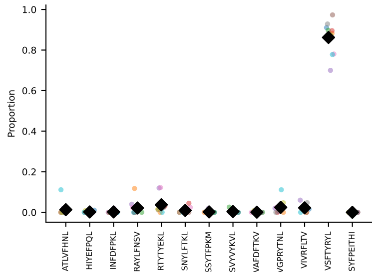
#24 AV9D-4-CALSANMGYKLTF-AJ9_BV13-1-CASSEGTTGGIYEYF-BJ2-7 coh=0.989, n=10
